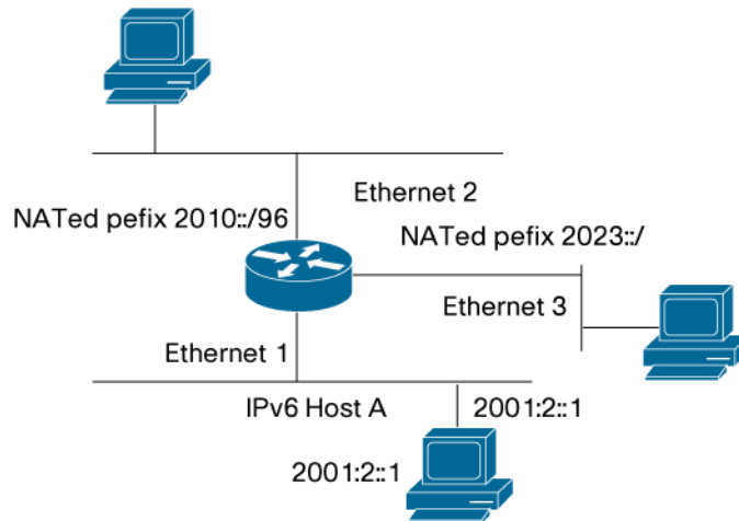
Figure 6. A Multiple Exits NAT-PT Topology
