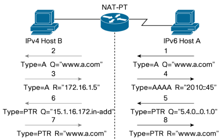
Figure 3. DNS Requests Flow in a NAT-PT for IPv6 Initiated Communications.
