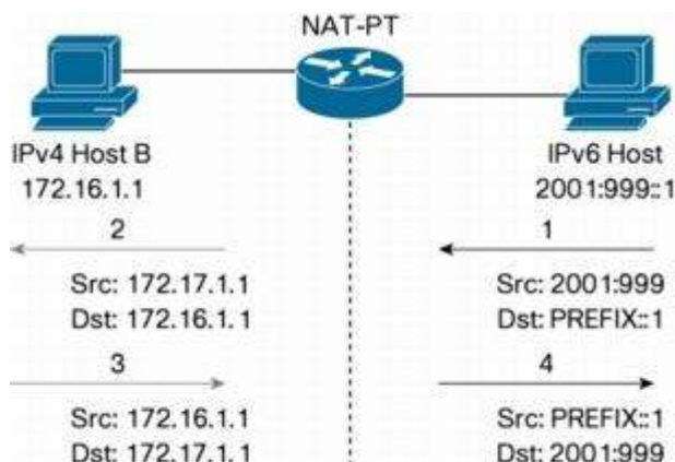
Figure 2. IPv6 Initiated Communication with Static Mapping
