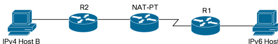
Figure 4. A Simple NAT-PT Setup where ICMP Packet Translations Occurs
