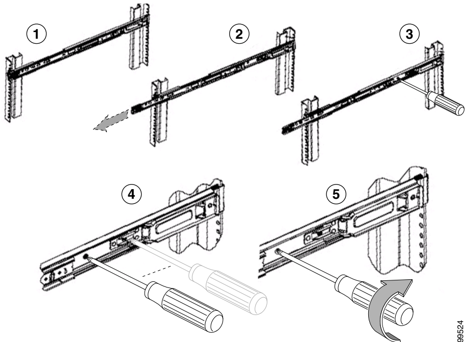
Figure 2-6 Attaching Screws to Telescopic Rail
