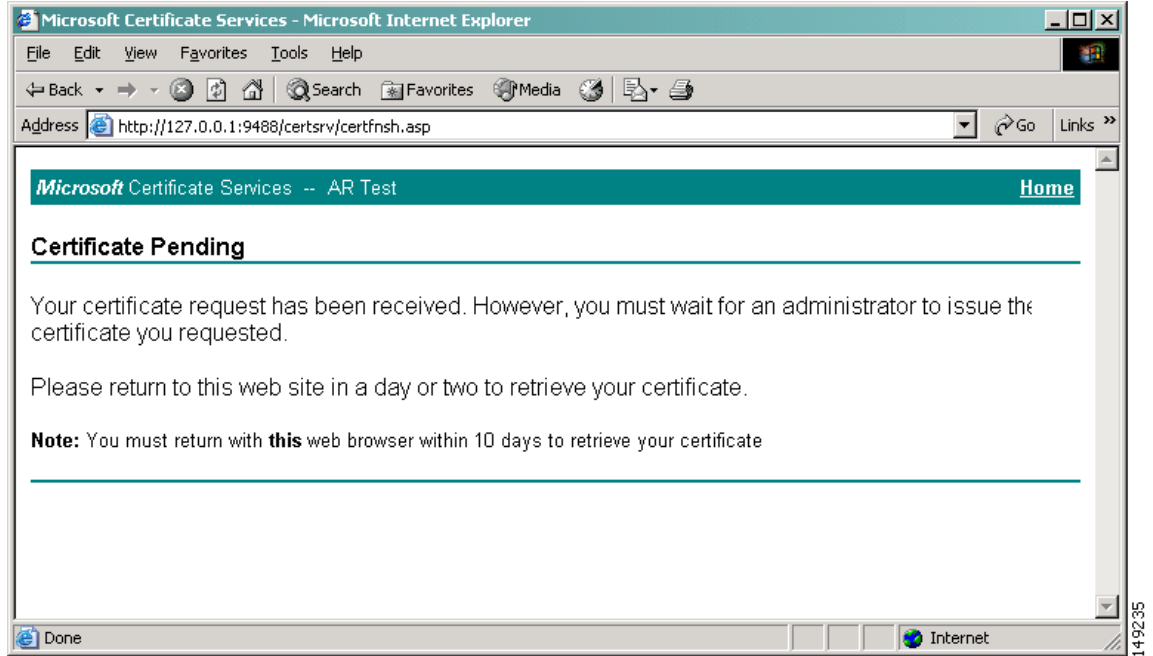
Figure 2-6 Certificate Pending
