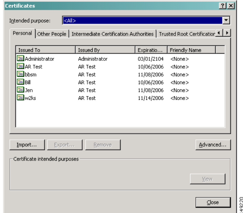
Figure 2-13 Certificates Dialog
