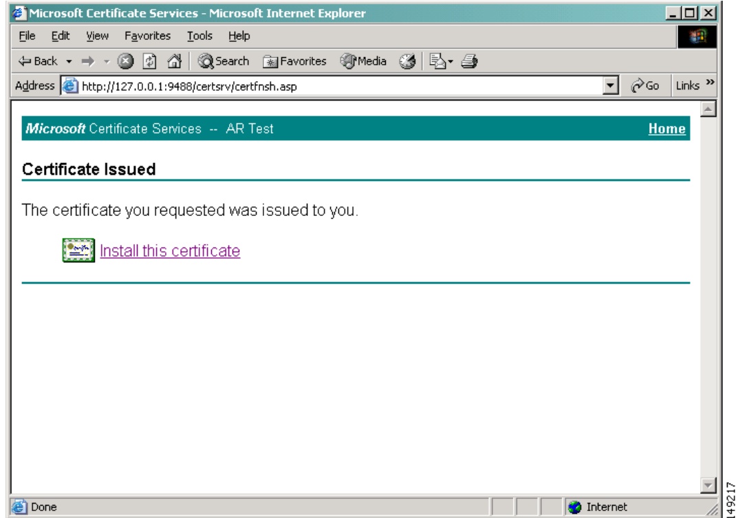
Figure 2-11 Certificate Issued
