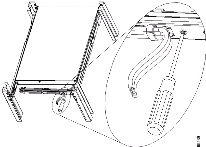
Figure 2-12 Fastening the Server into the Rack
