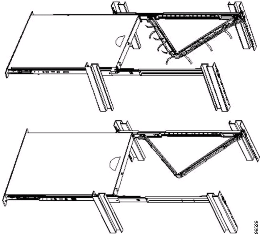
Figure 2-11 Installing Cable in Management Arm
