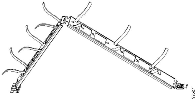
Figure 2-9 Attaching Velcro to Management Arm
