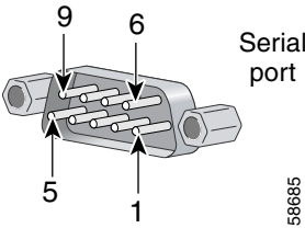
Figure 1-3 Pin Numbers for the Serial Port Connectors
