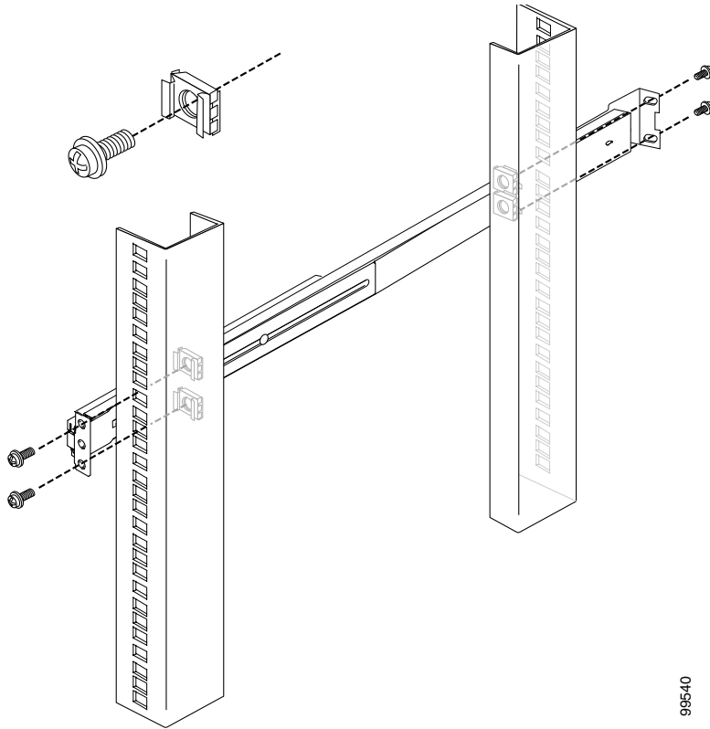
Figure 2-5 Attaching Back Rail to Rack
