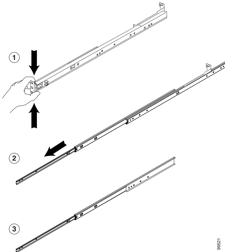
Figure 2-2 Removing the Server Rail
