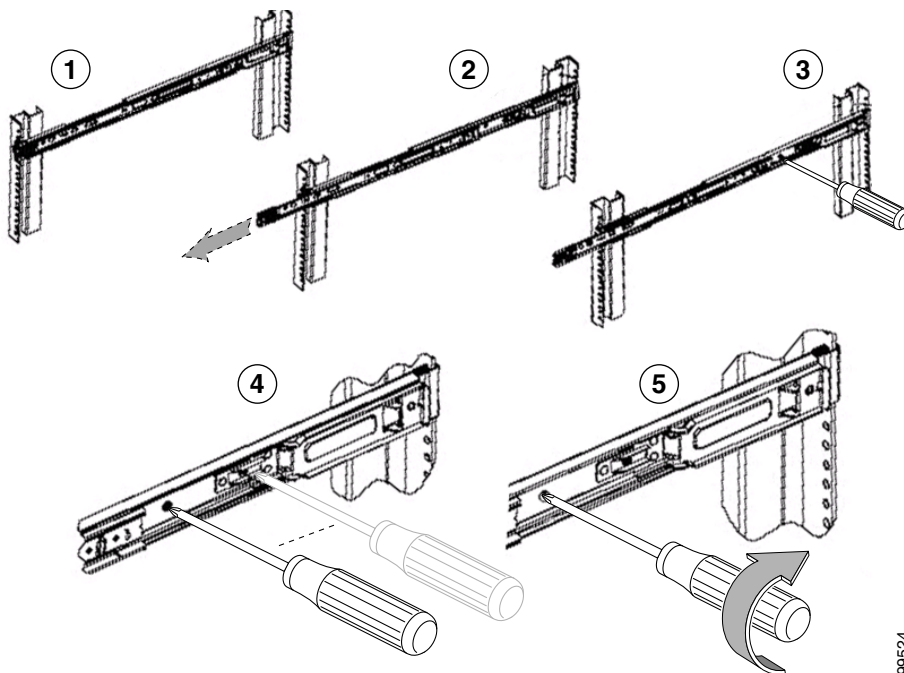
Figure 2-6 Attaching Screws to Telescopic Rail
