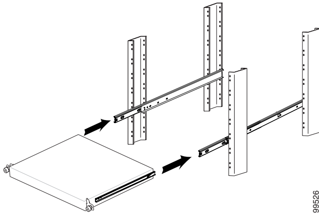
Figure 2-8 Sliding Chassis onto Rack
