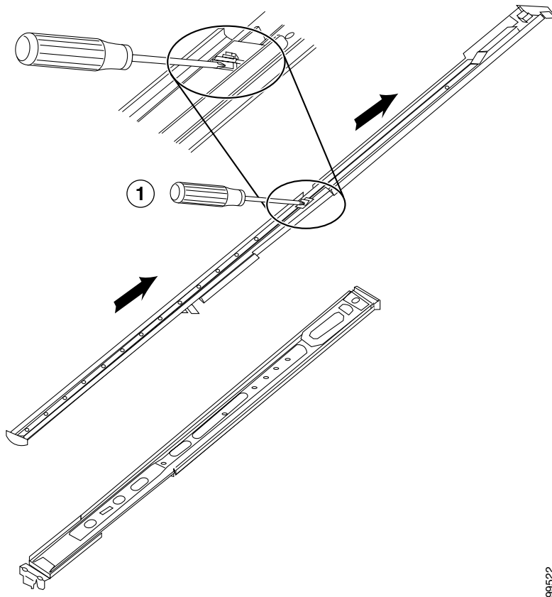
Figure 2-3 Telescoping the Rail
