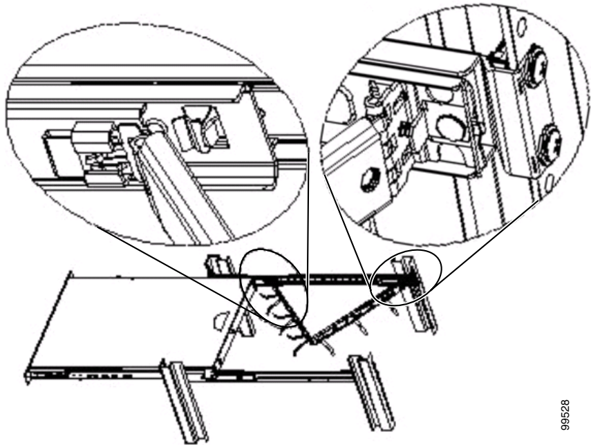
Figure 2-10 Attaching Management Arm
