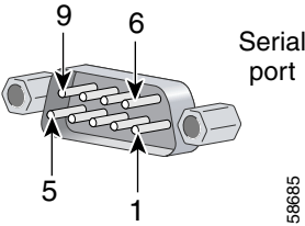
Figure 1-3 Pin Numbers for the Serial Port Connector
