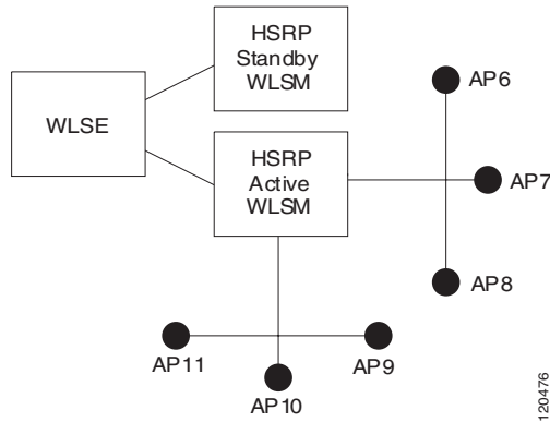
Figure 4-3 WLSE-WLSM Communications
