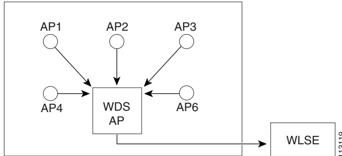
Figure 4-2 Additional Radio Management Communications
