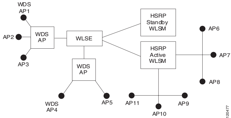
Figure 4-4 Sample Network Using AP-WDS and WLSM-WDS Devices
