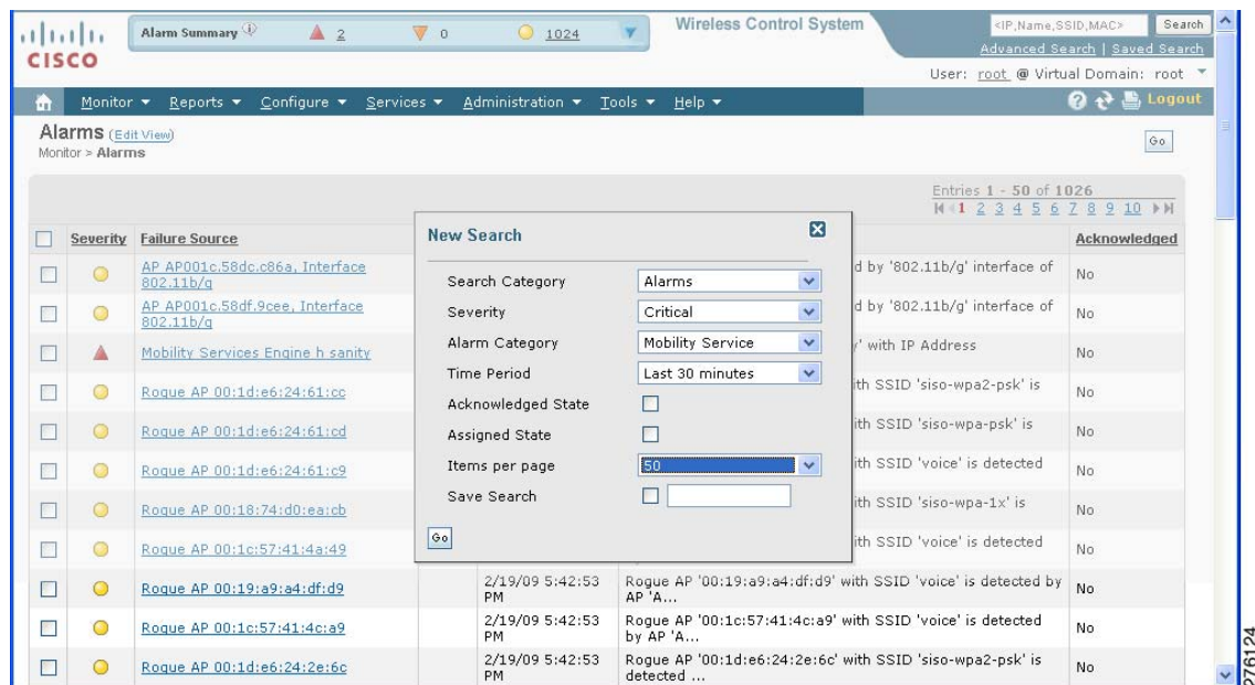
Figure 7-1 Advanced Search Alarm Panel
