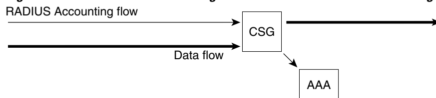
Figure 5-1 RADIUS Accounting and Data Flows—RADIUS Accounting Proxy or Monitor
