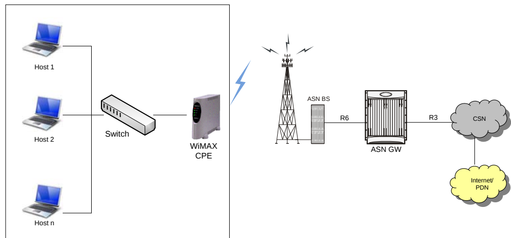
Figure 1-1 Multi Host Support with WiMAX Network
