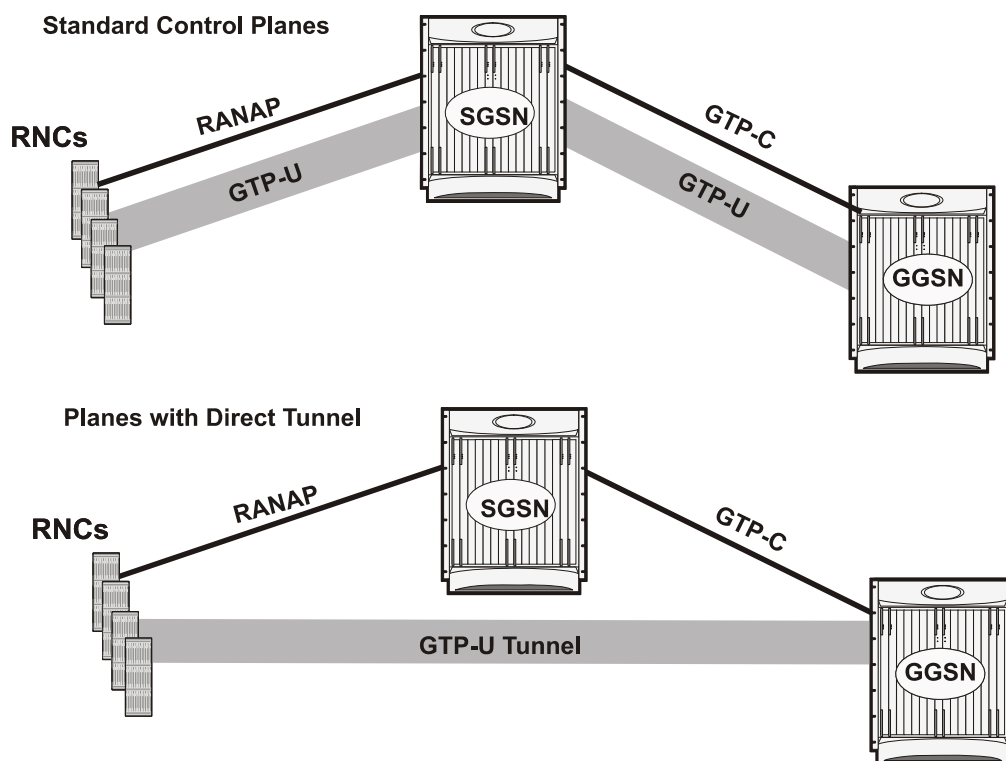
Figure 1-3 Direct Tunnel Support in GGSN
