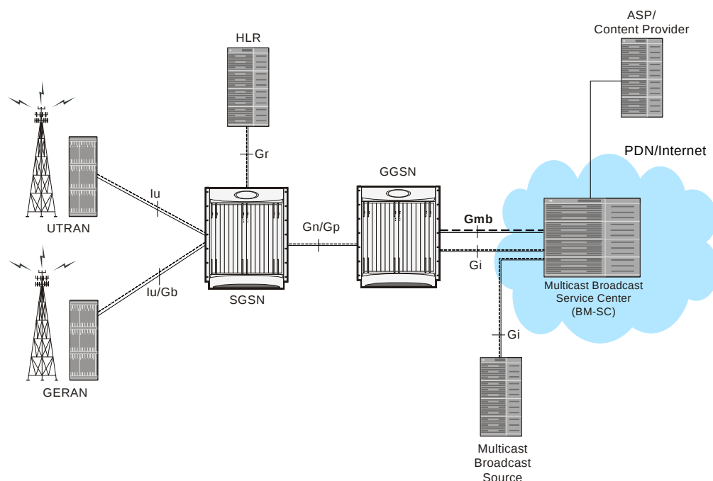
Figure 1-2 MBMS Reference Architecture in UMTS network
