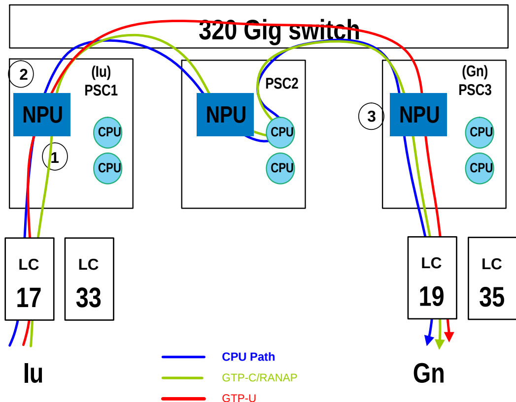
Figure 1-5 SGSN NPU FastPath
