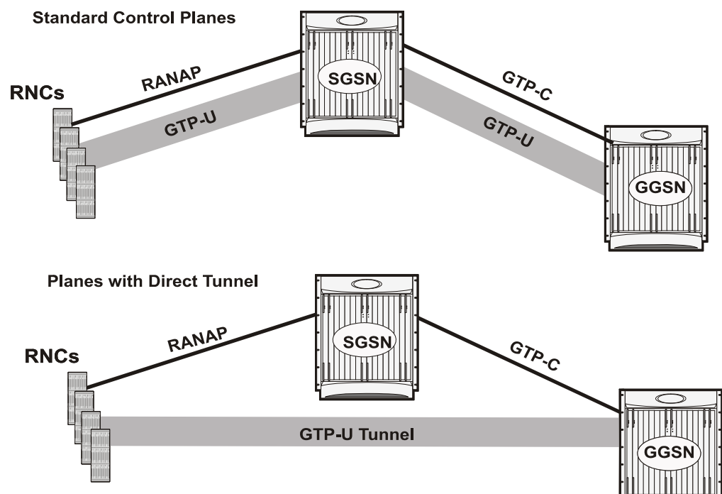
Figure 1-4 SGSN Direct Tunnel
