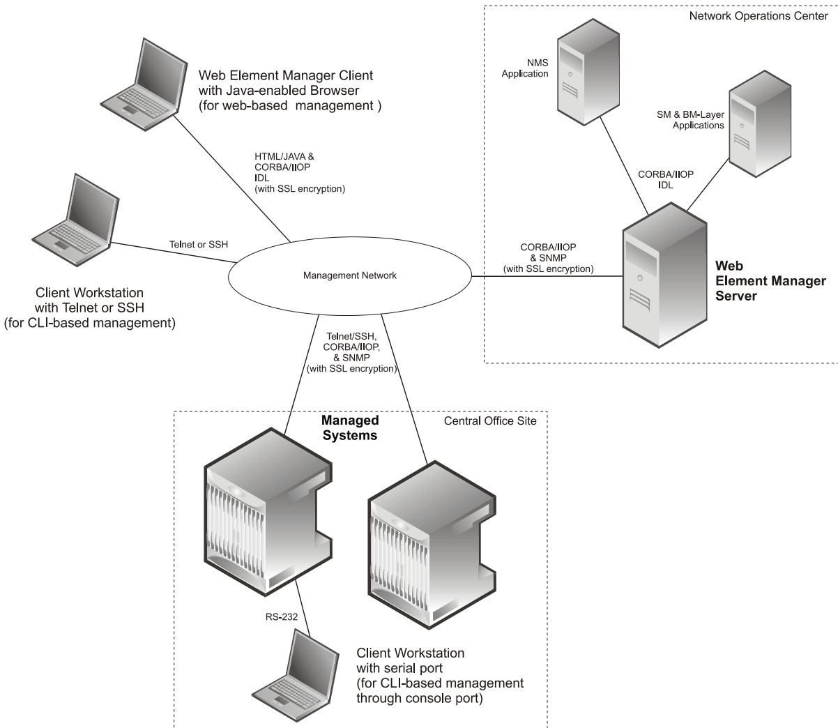
Figure 99. Element Management Methods
