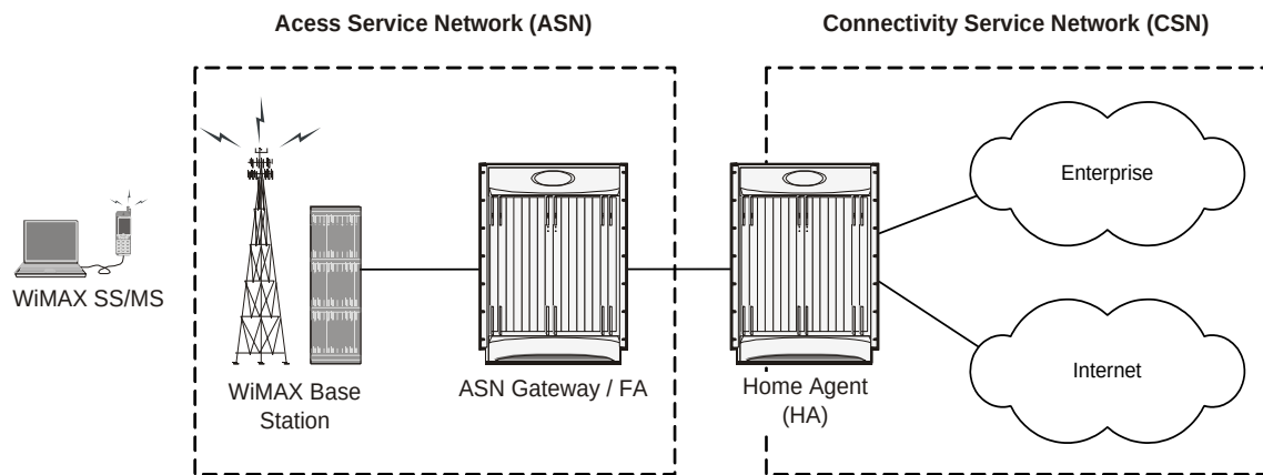
Figure 30. Basic ASN Gateway Mobile IP Network
