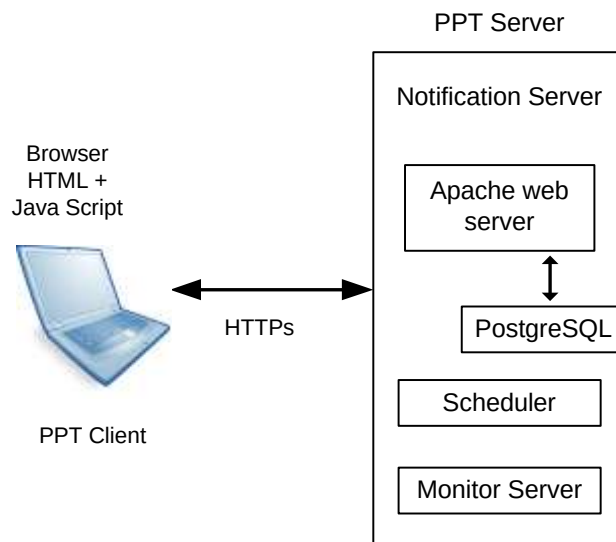
Figure 227. PPT Architecture
