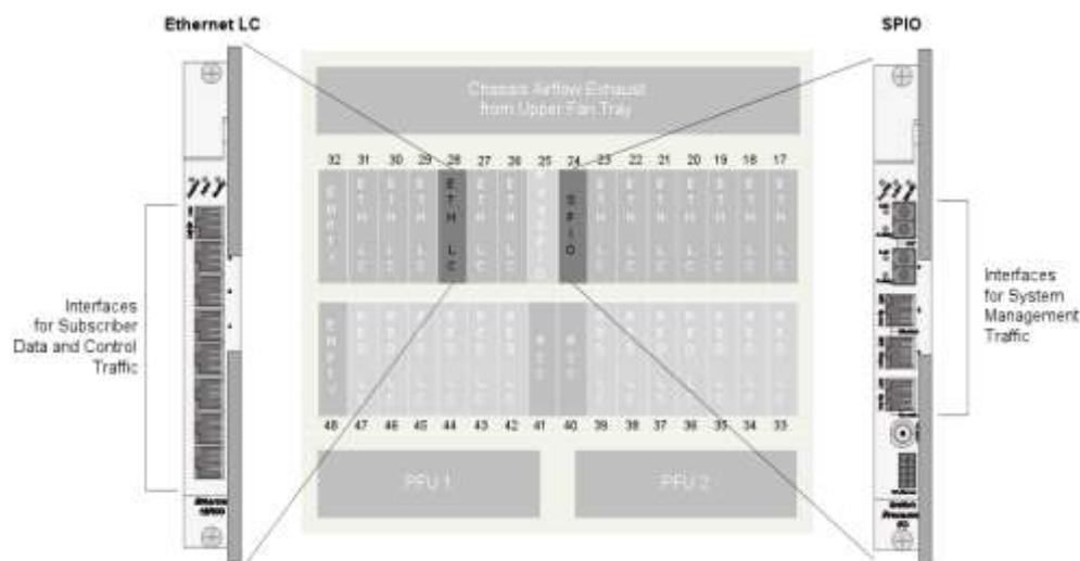
Figure 27. Separation of Management Data From User Data
