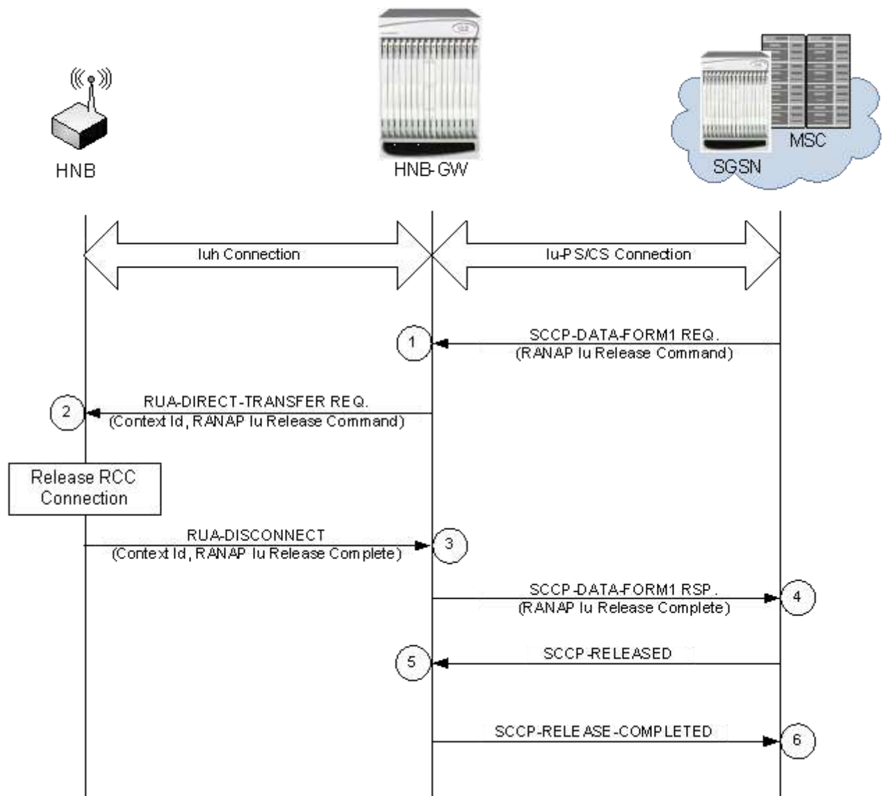
Figure 125. Network Initiated Iu Connection Release Call Flow
