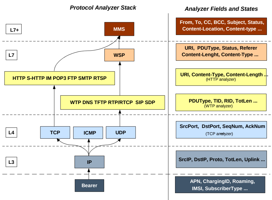
Figure 78. ECS Protocol Analyzer Stack
