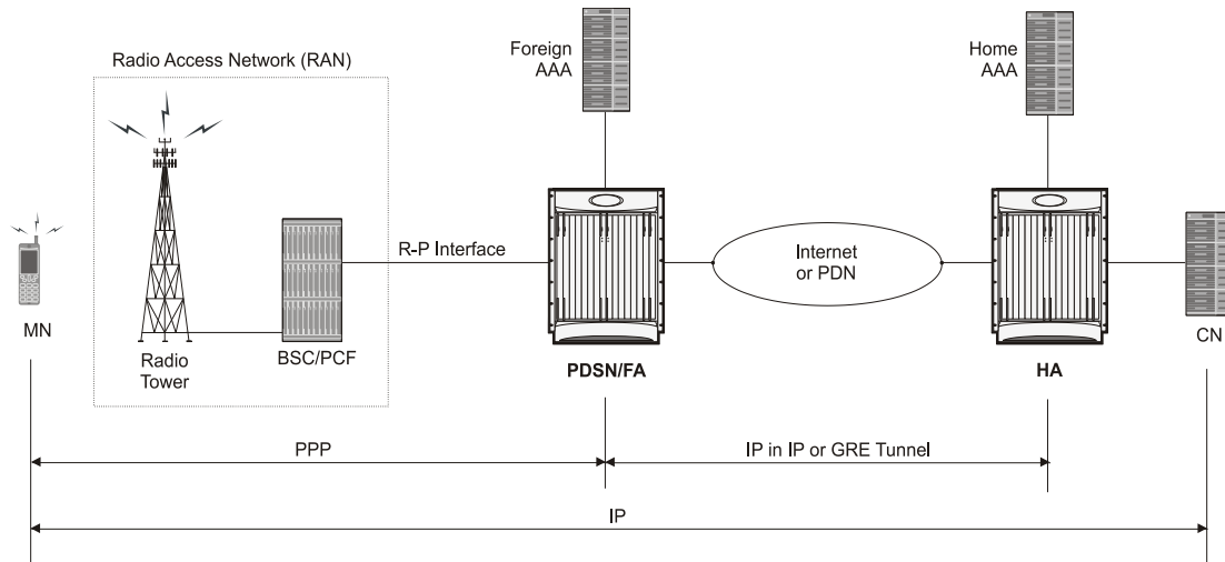
Figure 70. Mobile IP Protocol Usage
