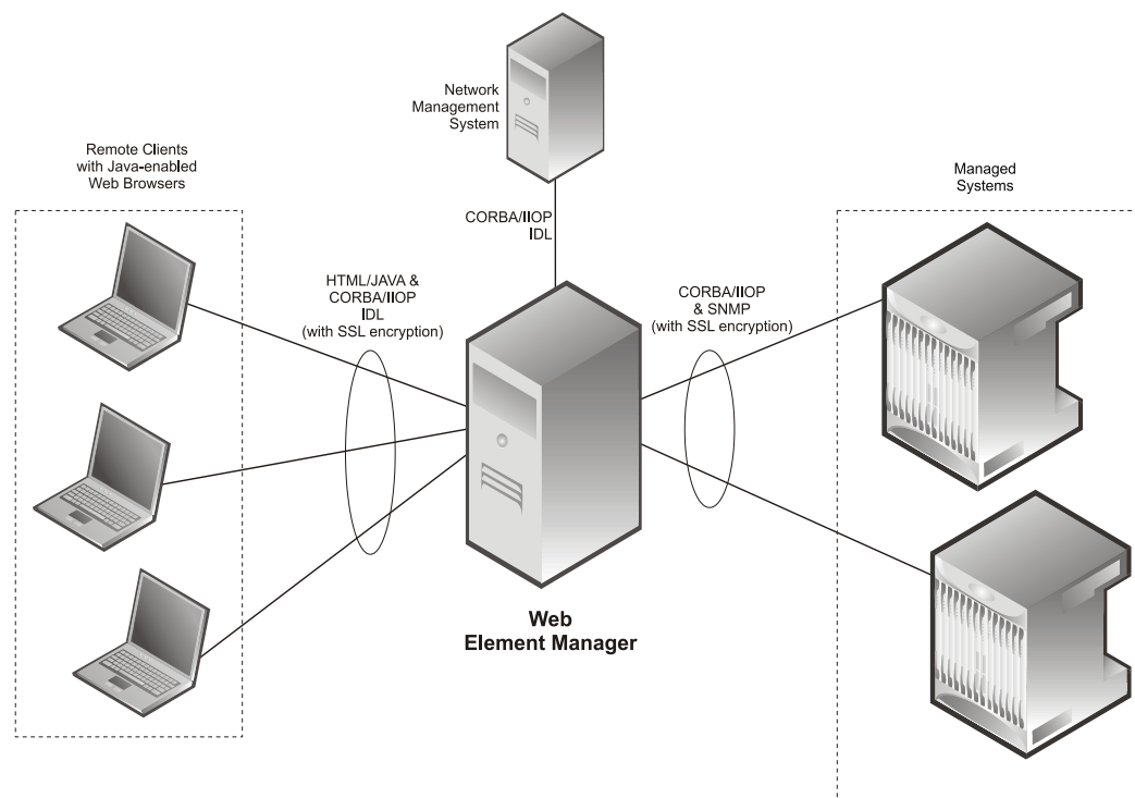
Figure 139. Element Management System
