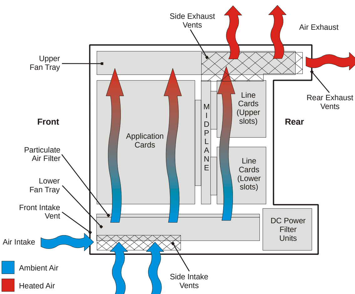
Figure 292. System Airflow and Ventilation
