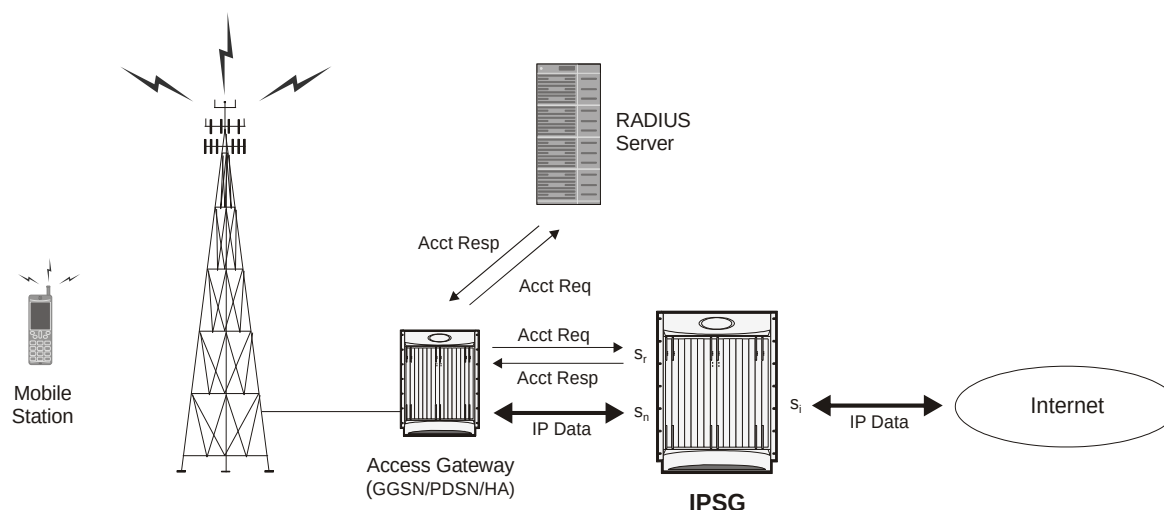
Figure 143. IPSG Message/Data Flow (RADIUS Server Mode)
