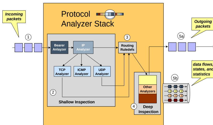
Figure 80. Routing Ruledefs and Packet Inspection
