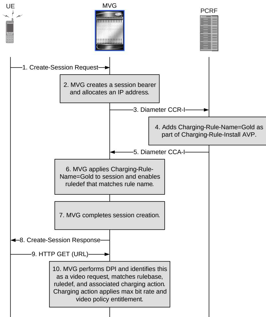
Figure 155. Mobile Video Gateway as a RADIUS Endpoint Obtaining the Video Policy via the PCRF
