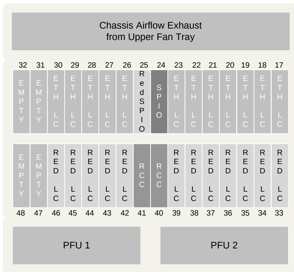
Figure 25. Recommended Redundant Configuration for Data Services - Rear View
