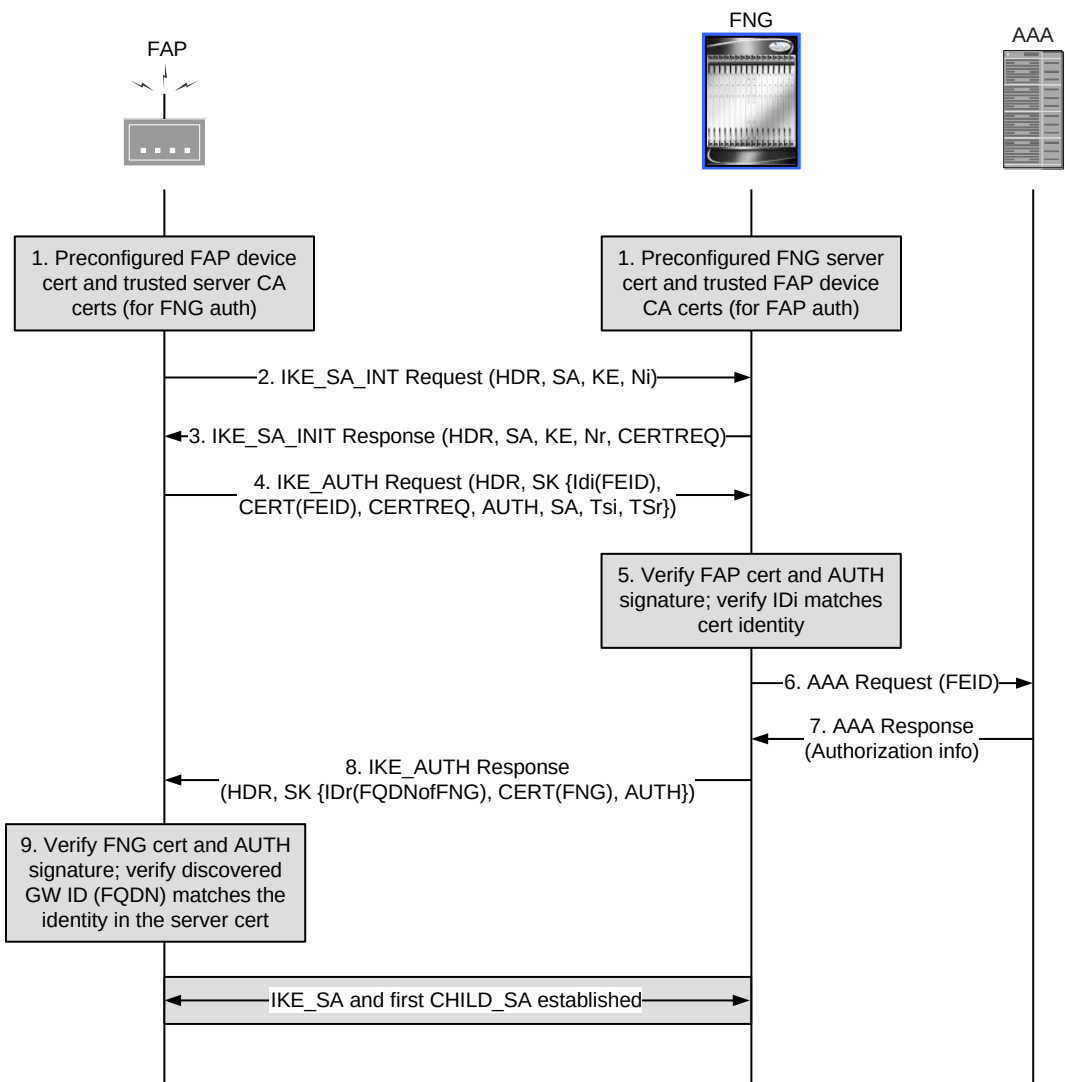
Figure 91. IPSec Tunnel Establishment
