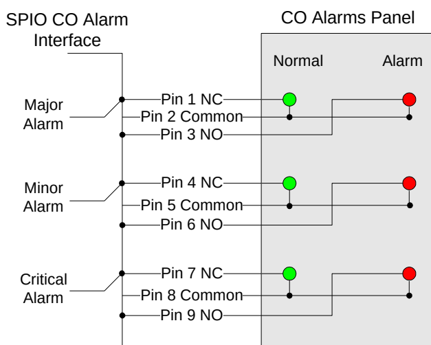
Figure 279. CO Alarm Wiring Example
