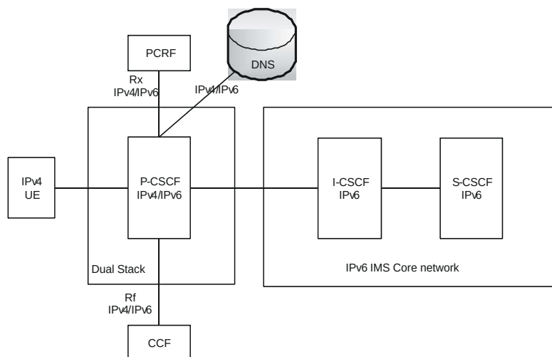
Figure 249. Interworking Between IPv4 UE and IPv6 IMS Core Network
