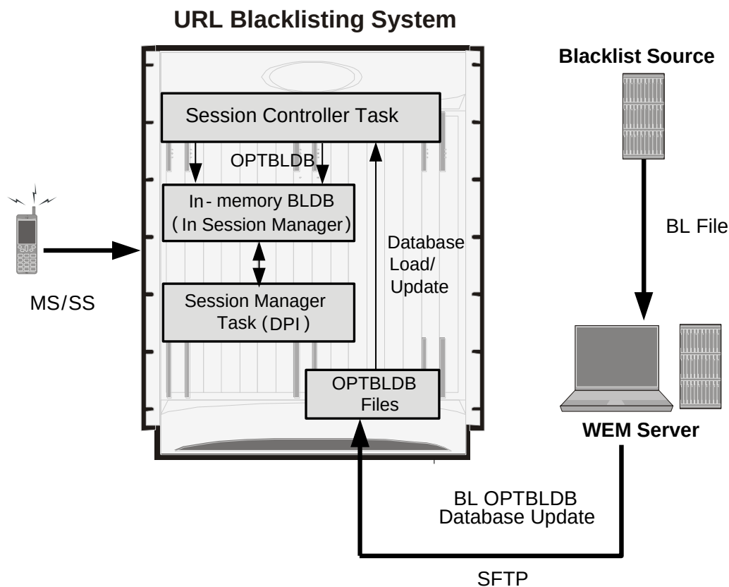
Figure 74. High-Level Architecture of URL Blacklisting with ECS
