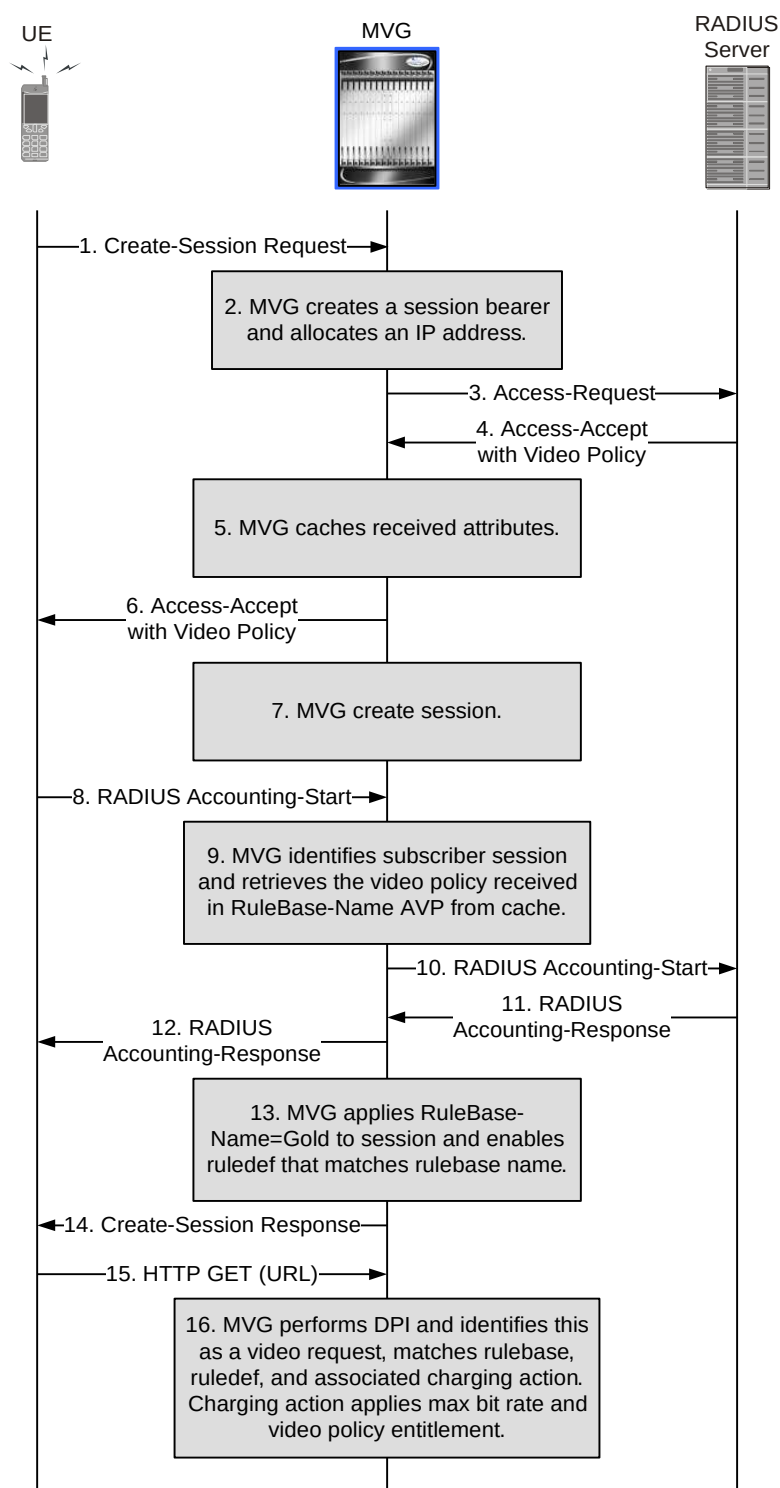
Figure 156. Mobile Video Gateway as a RADIUS Proxy Obtaining the Video Policy via the RADIUS Server
