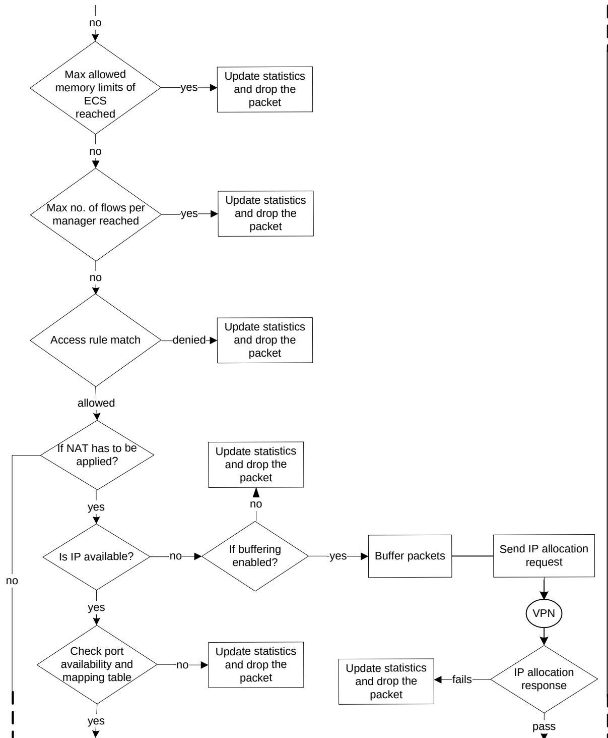
Figure 187. ... NAT Processing Flow
