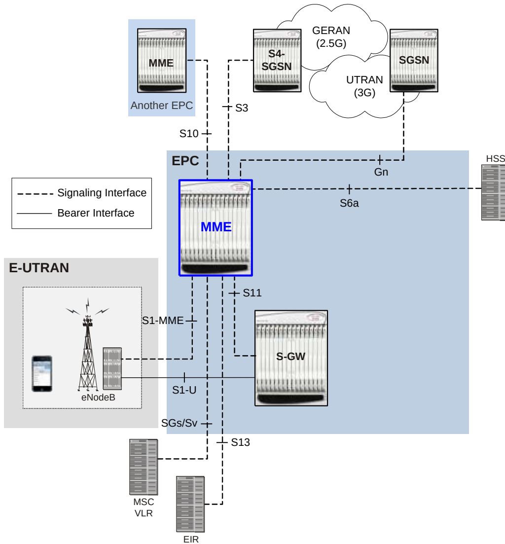
Figure 171. Supported MME Interfaces in the E-UTRAN/EPC Network
