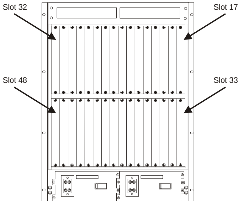
Figure 5. Rear Slot Numbering Scheme for Line Cards
