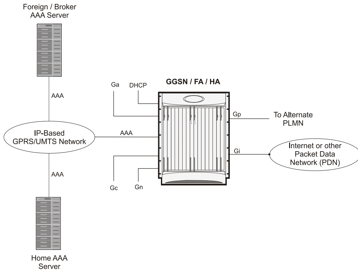
Figure 97. Combined GGSN/FA/HA Deployment for Mobile IP and/or Proxy Mobile IP Support
