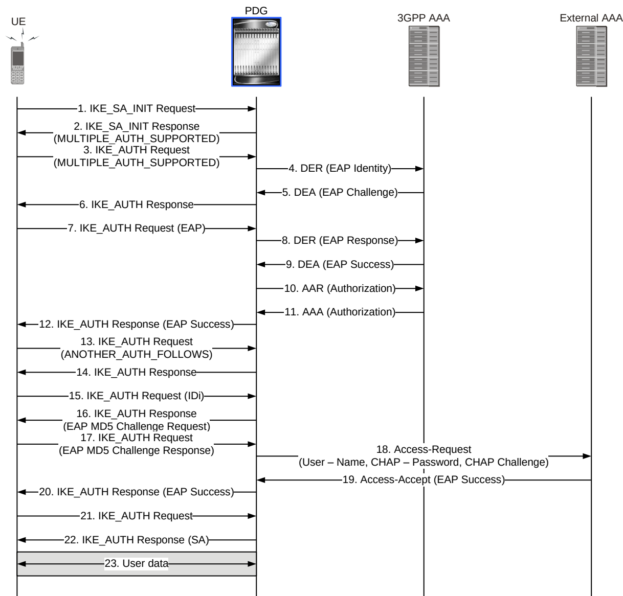
Figure 205. Multiple Authentication Using EAP and CHAP
