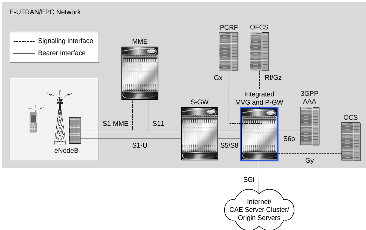
Figure 148. Mobile Video Gateway in an E-UTRAN/EPC Network
