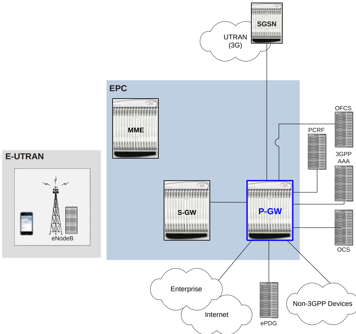
Figure 208. P-GW in the Basic E-UTRAN/EPC Network
