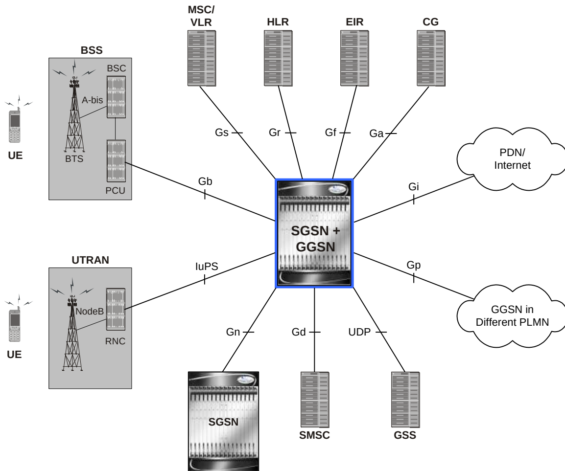
Figure 252. Co-located SGSN and GGSN
