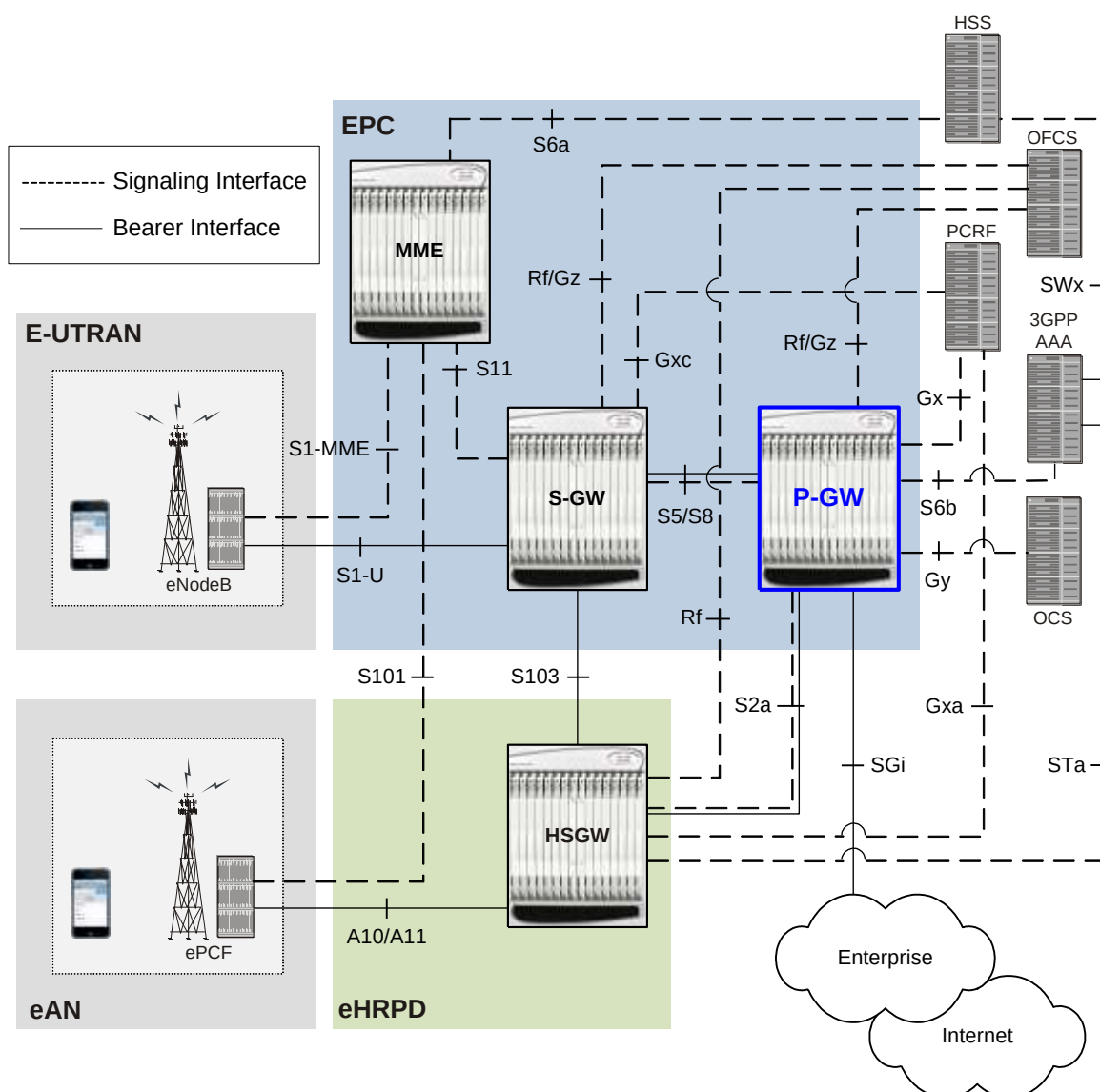
Figure 213. P-GW in the E-UTRAN/EPC Network Supporting the eHRPD Network
