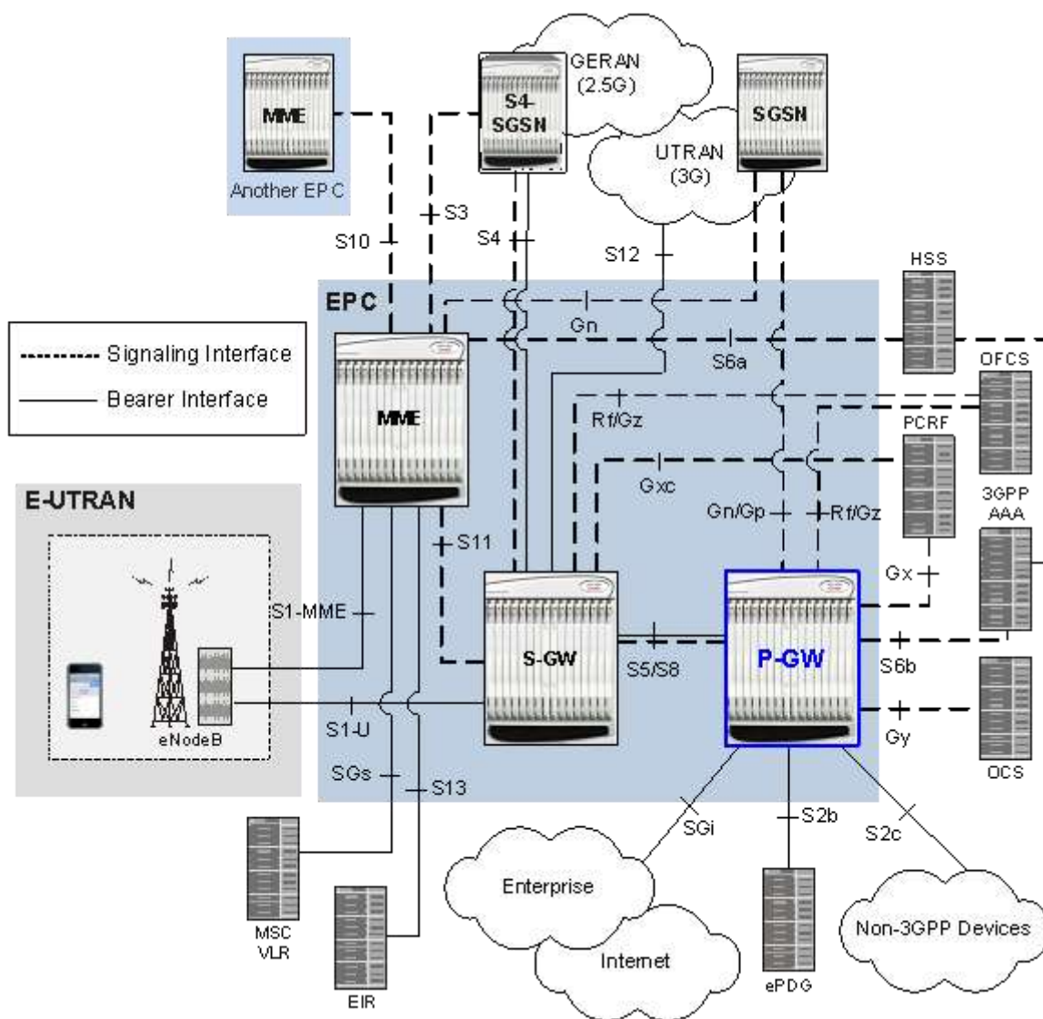
Figure 211. P-GW in the E-UTRAN/EPC Network
