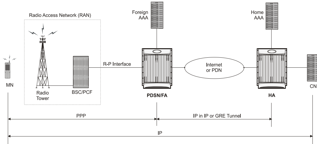
Figure 116. Mobile IP Protocol Usage.
