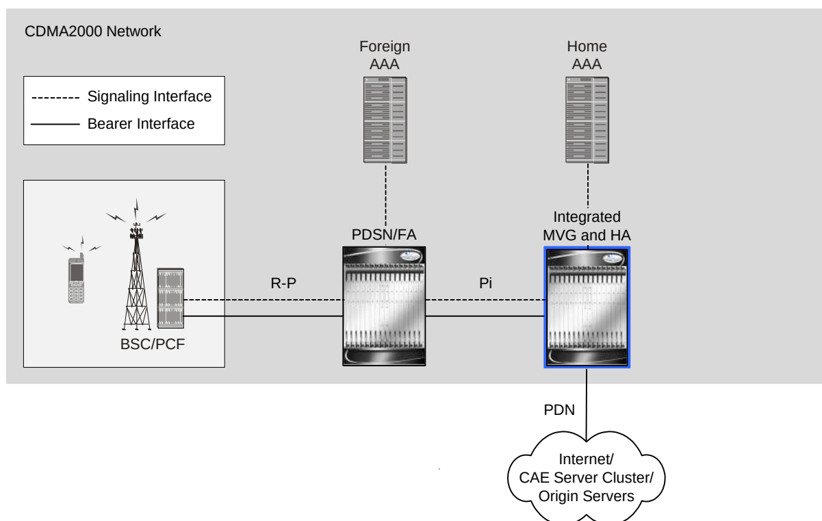
Figure 150. Mobile Video Gateway in a CDMA2000 Network
