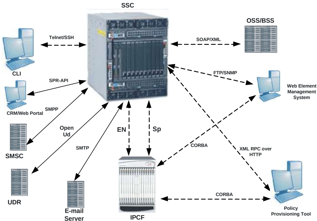
Figure 264. SSC Deployment Scenario
