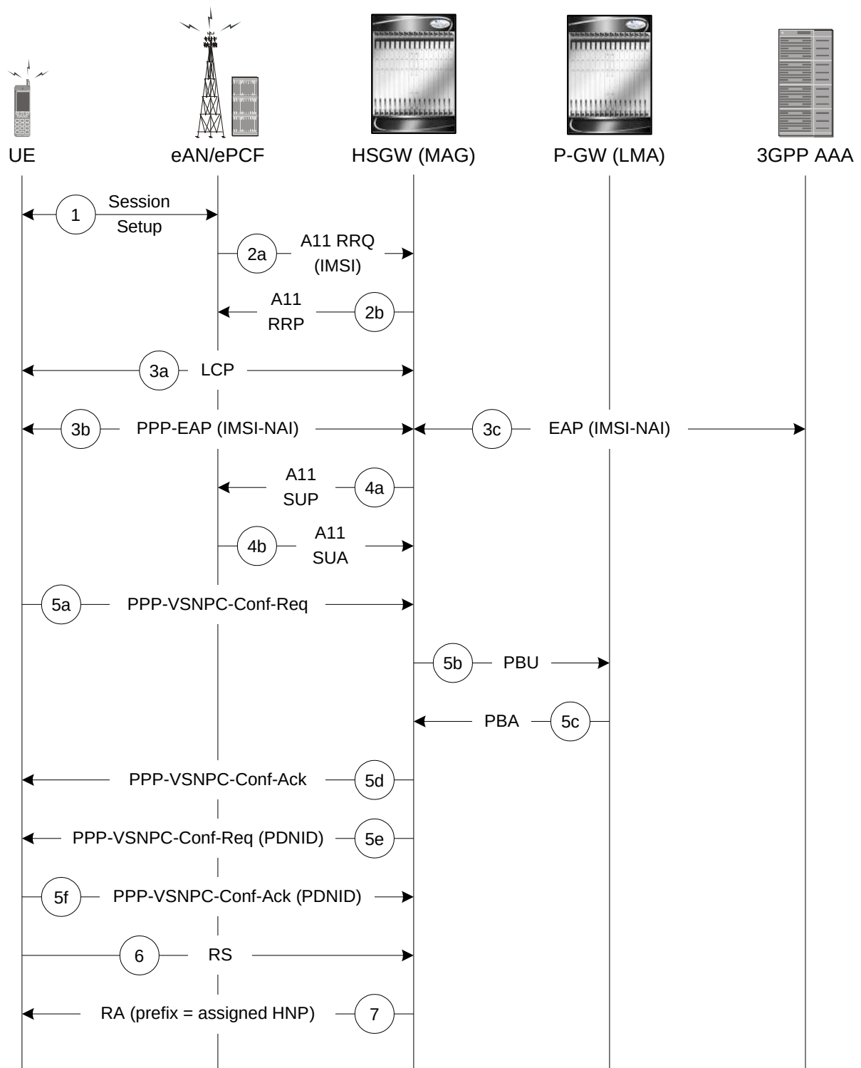
Figure 216. Initial Attach with IPv6/IPv4 Access Call Flow
