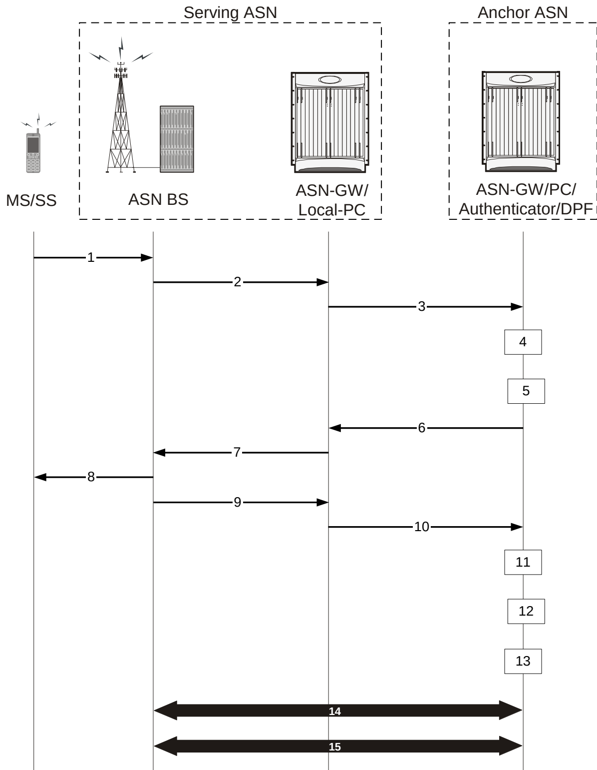
Figure 62. MS Initiated Idle Mode Entry Procedure Flow
