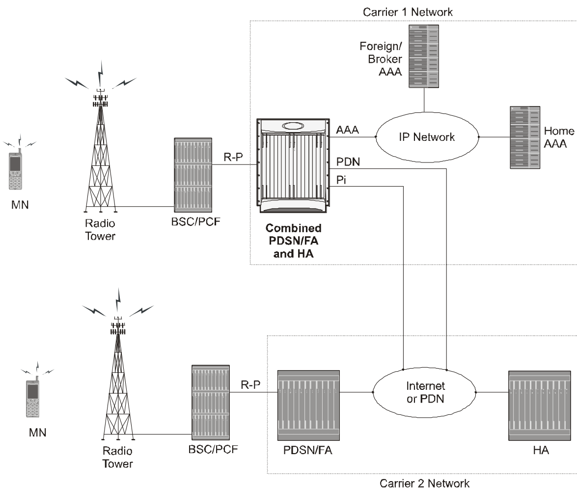
Figure 114. Co-located PDSN/FA and HA Configuration Example
