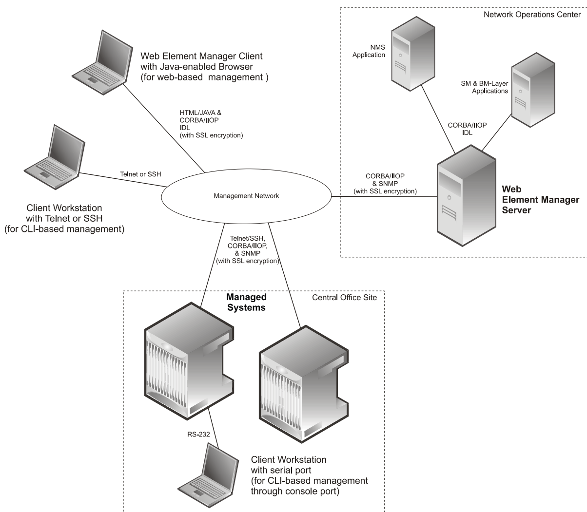
Figure 173. Element Management Methods
