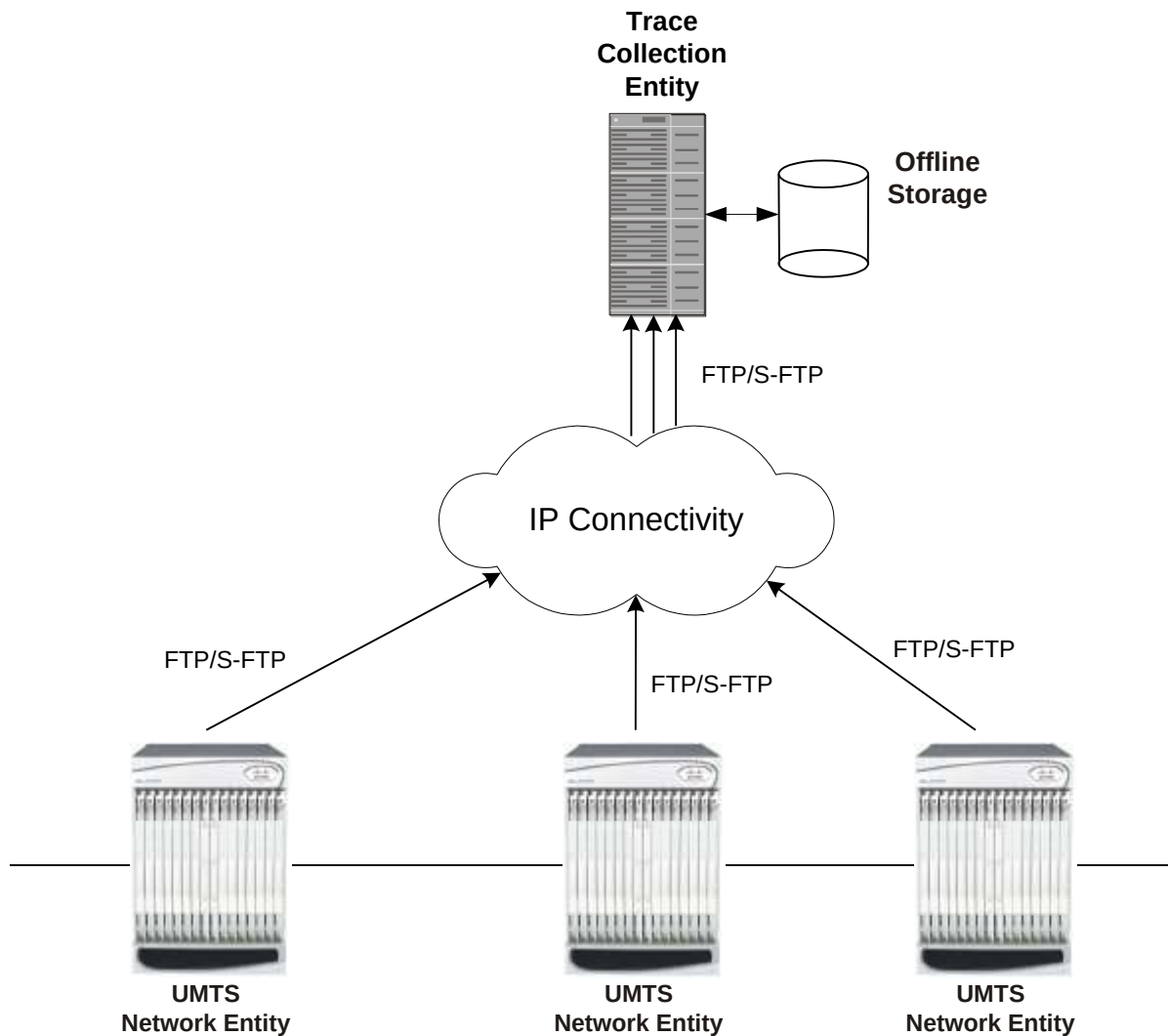
Figure 100. Session Trace Function and Interfaces
