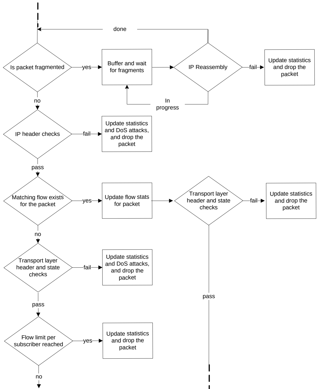
Figure 186. ... NAT Processing Flow
