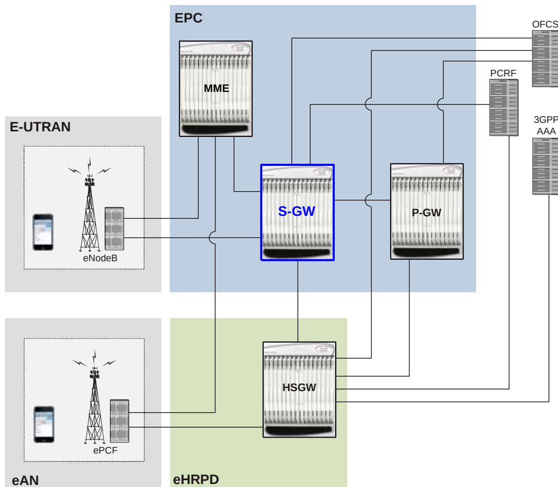
Figure 230. S-GW in the Basic E-UTRAN/EPC and eHRPD Network
