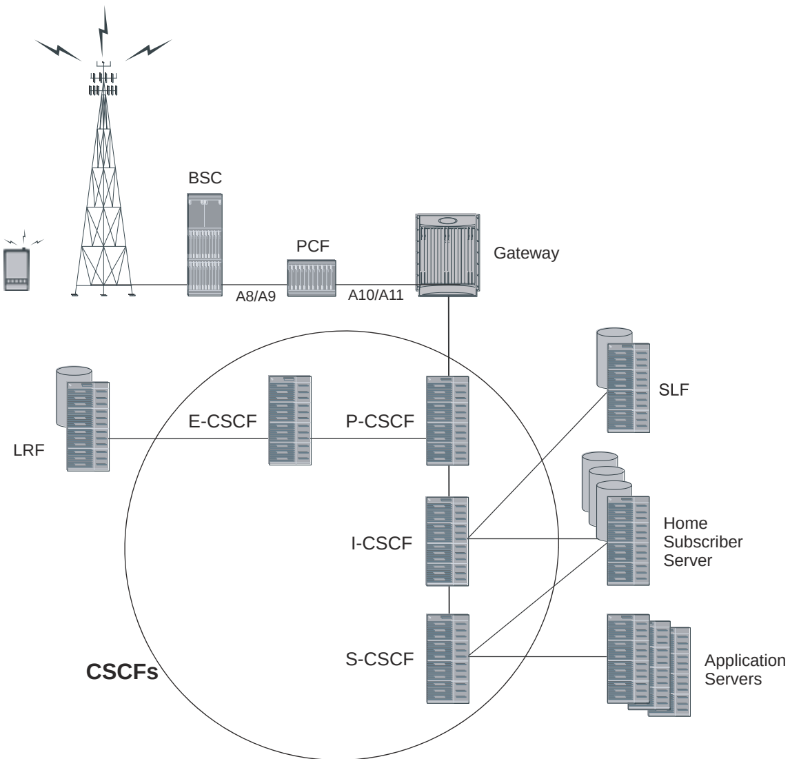
Figure 239. IMS CSCF Components
