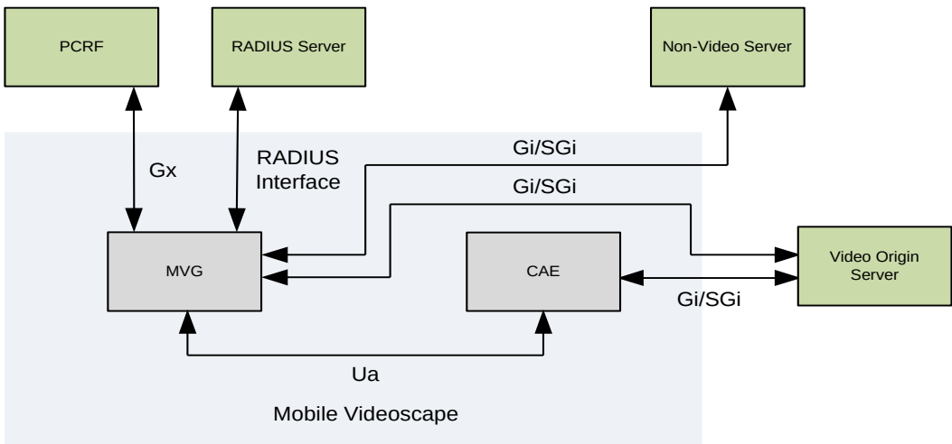
Figure 151. Logical Network Interfaces on the Mobile Video Gateway
