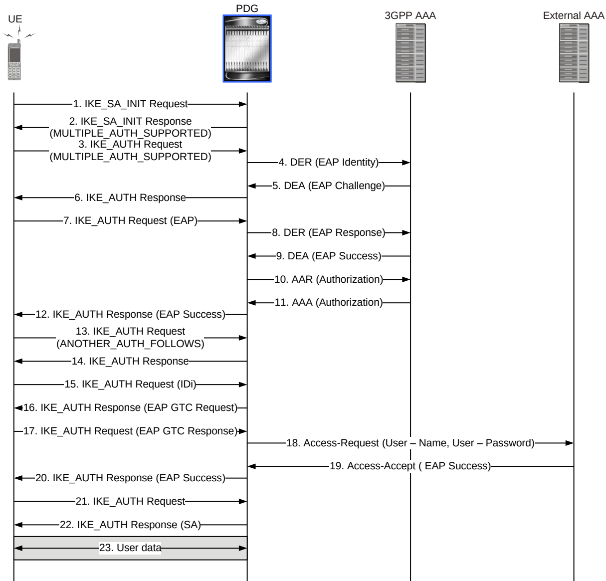
Figure 204. Multiple Authentication Using EAP and PAP
