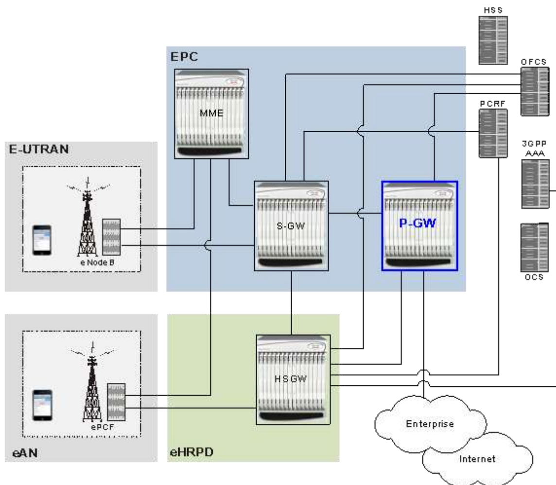
Figure 209. P-GW in the Basic E-UTRAN/EPC and eHRPD Network
