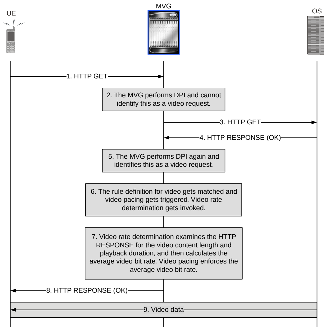
Figure 160. DPI of HTTP RESPONSE Identifying a Video Request
