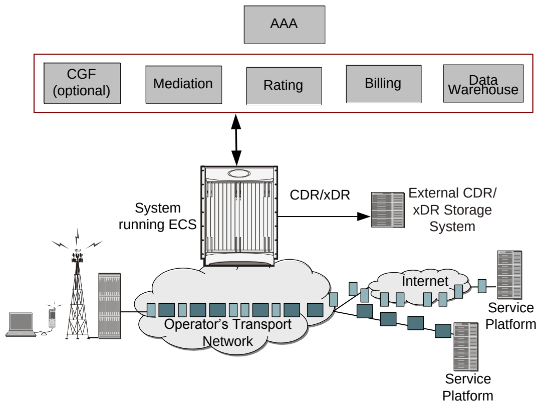
Figure 86. Postpaid Billing System Scenario with ECS
