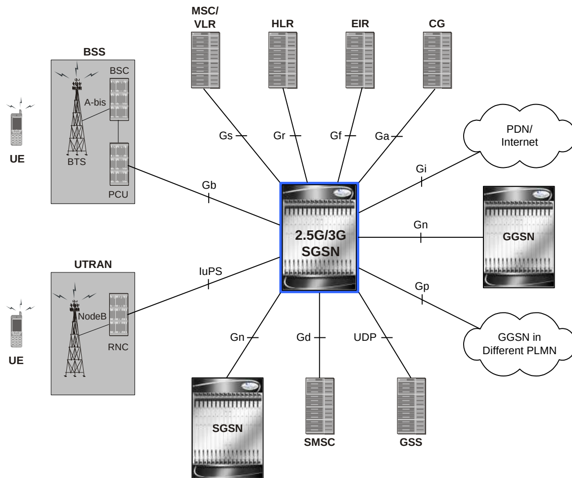
Figure 251. Dual Access 2.5/3G SGSNs
