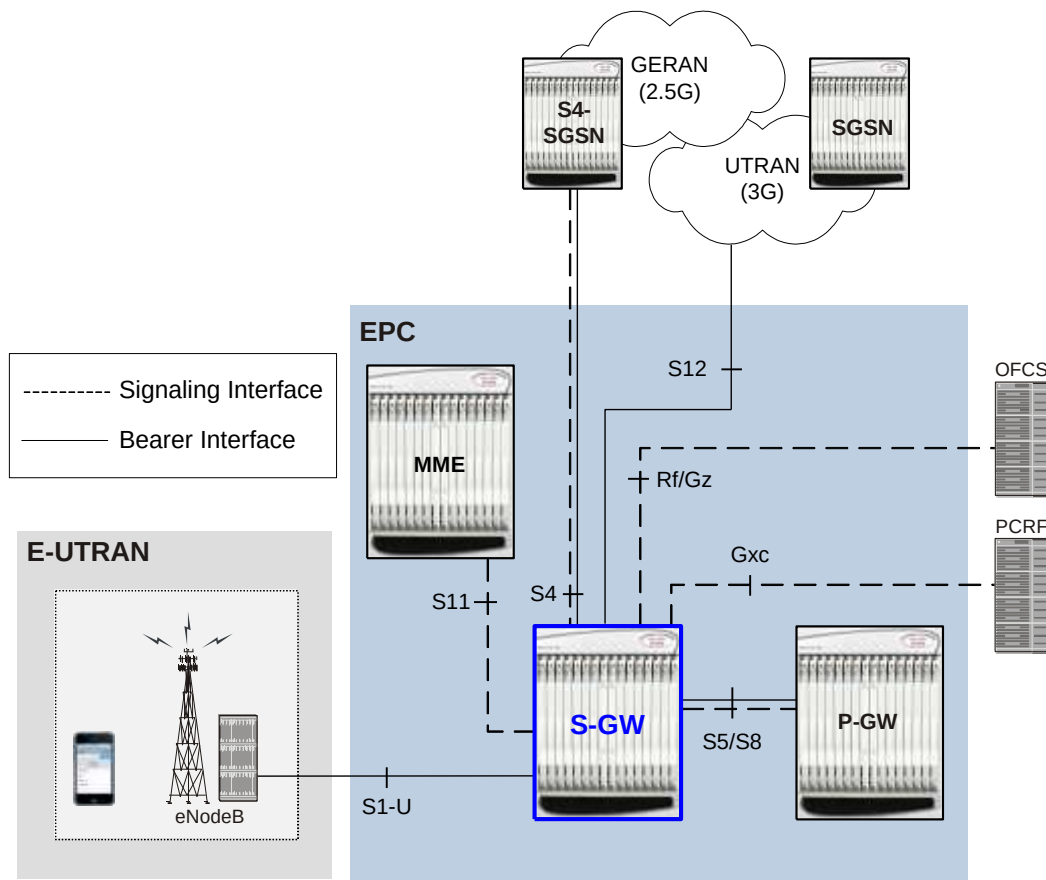
Figure 231. Supported S-GW Interfaces in the E-UTRAN/EPC Network
