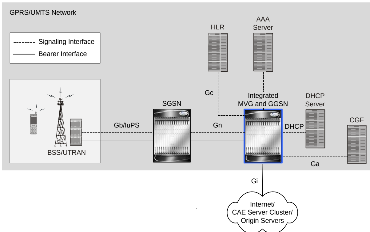
Figure 149. Mobile Video Gateway in a GPRS/UMTS Network
