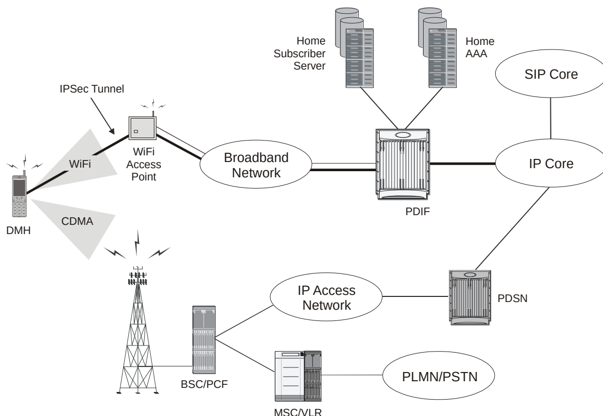
Figure 189. PDIF/FA Mobile IP Interfaces
