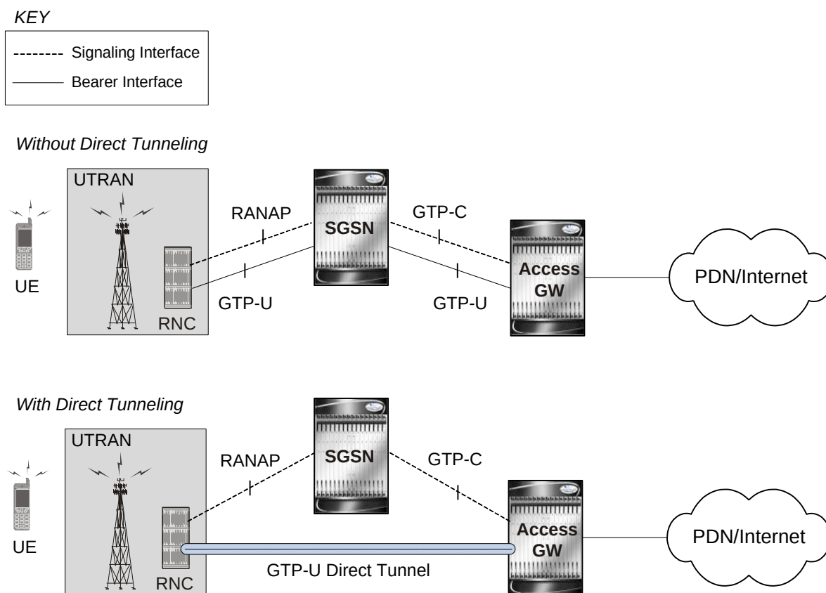
Figure 235. GTP-U with Direct Tunnel
