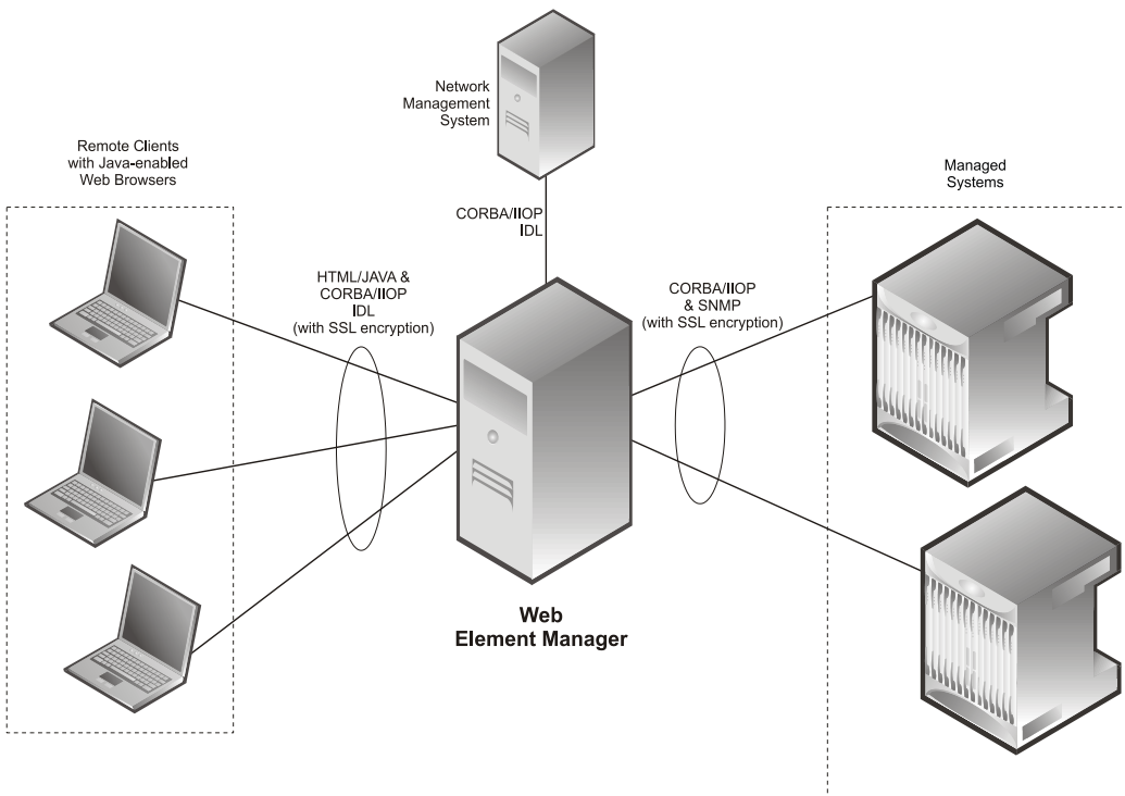
Figure 140. Web Element Manager Network Interfaces
