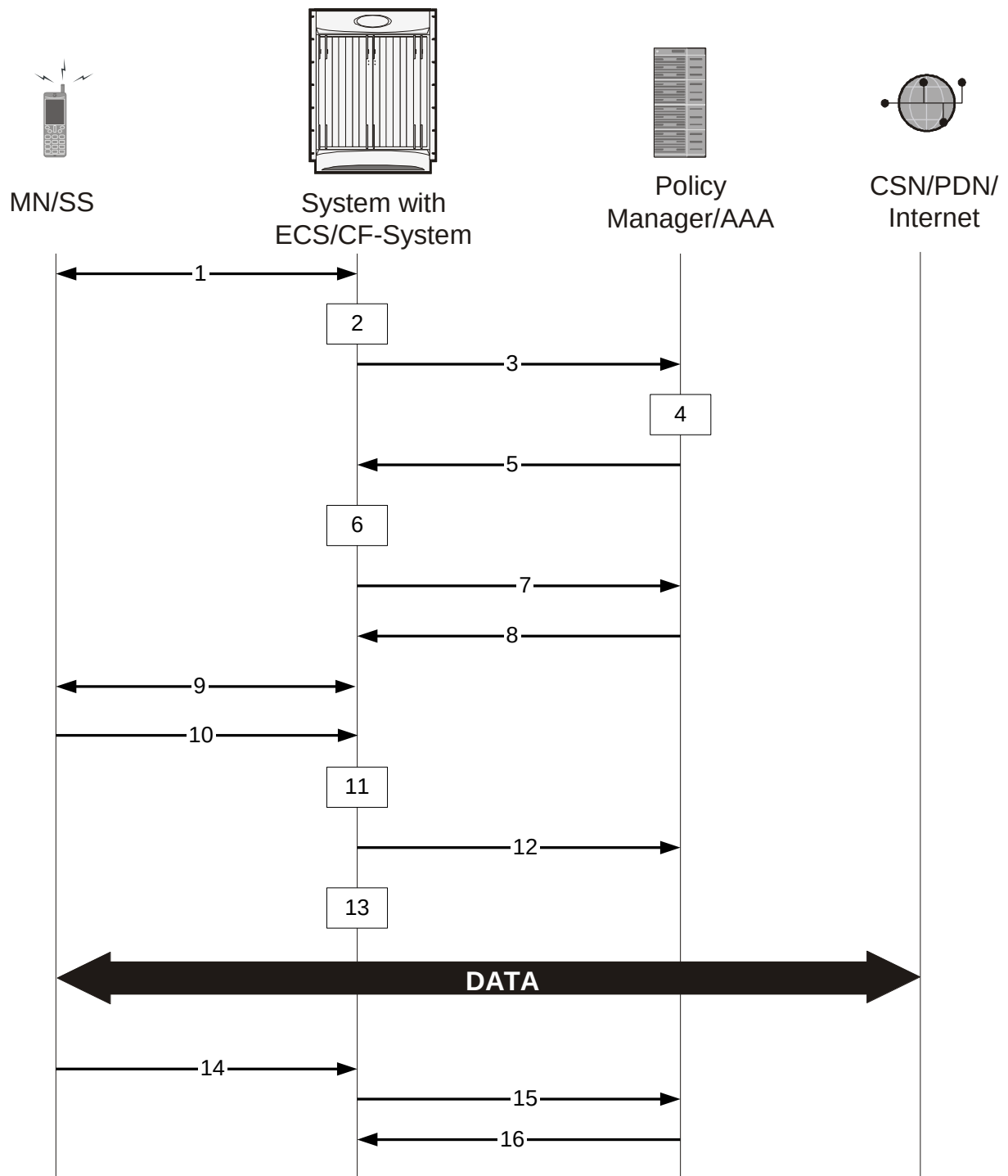
Figure 76. Content Filtering Call Flow
