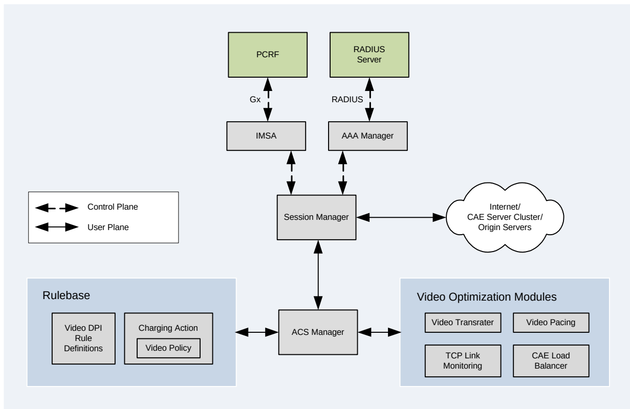
Figure 154. Video Optimization Policy Control System Flow
