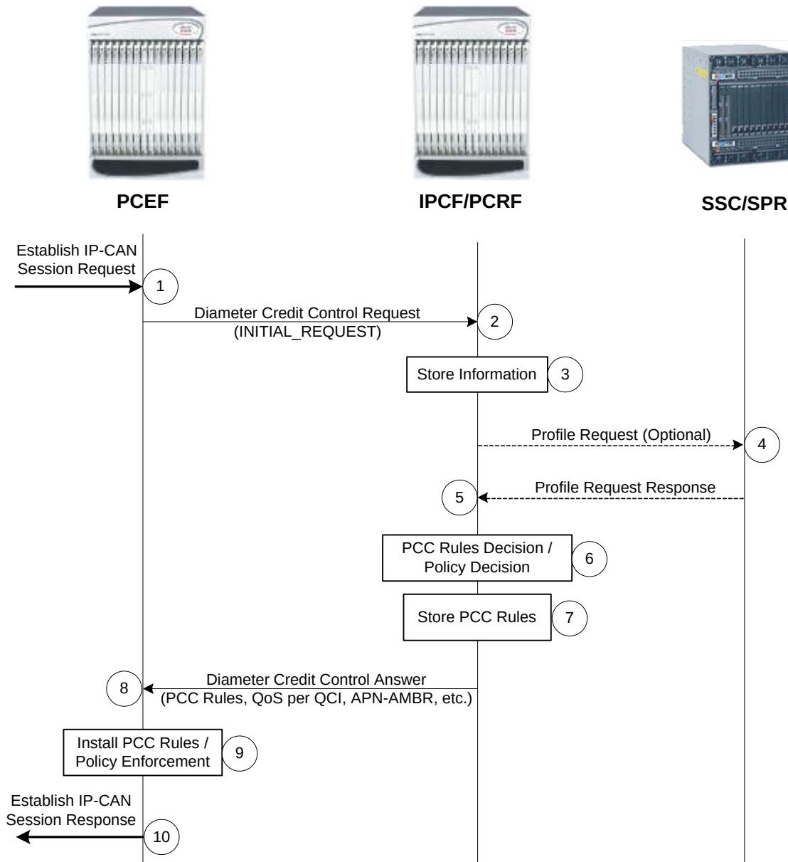
Figure 141. IP-CAN Session Setup Procedure Call Flow
