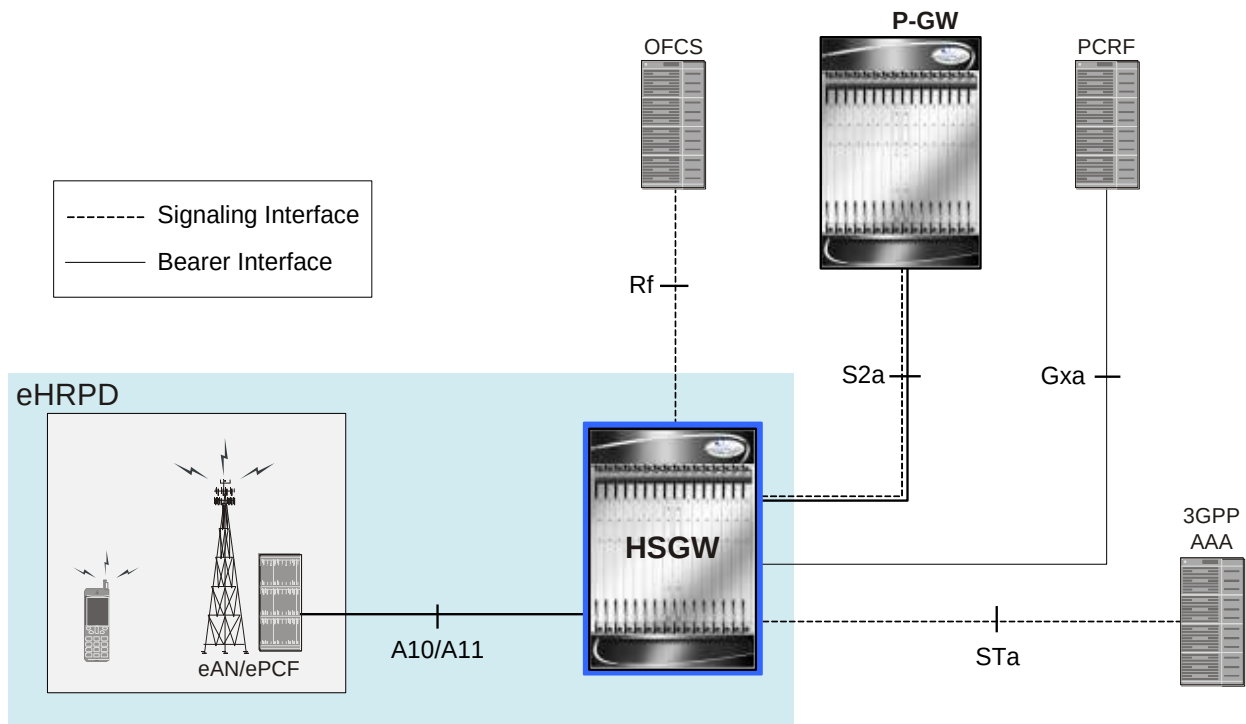
Figure 128. HSGW Supported Network Interfaces
