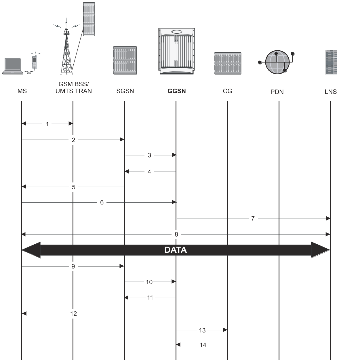
Figure 108. Virtual Dialup Access Call Flow
