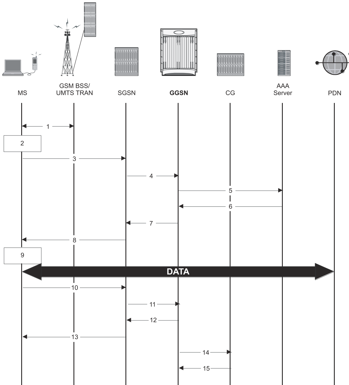
Figure 105. Non-Transparent IP Session Call Flow
