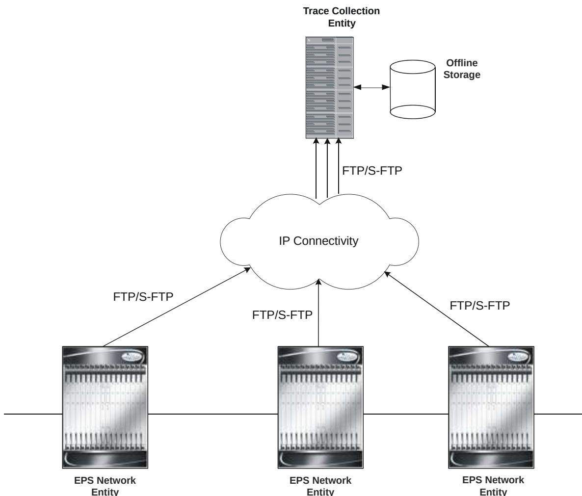
Figure 174. Session Trace Function and Interfaces
