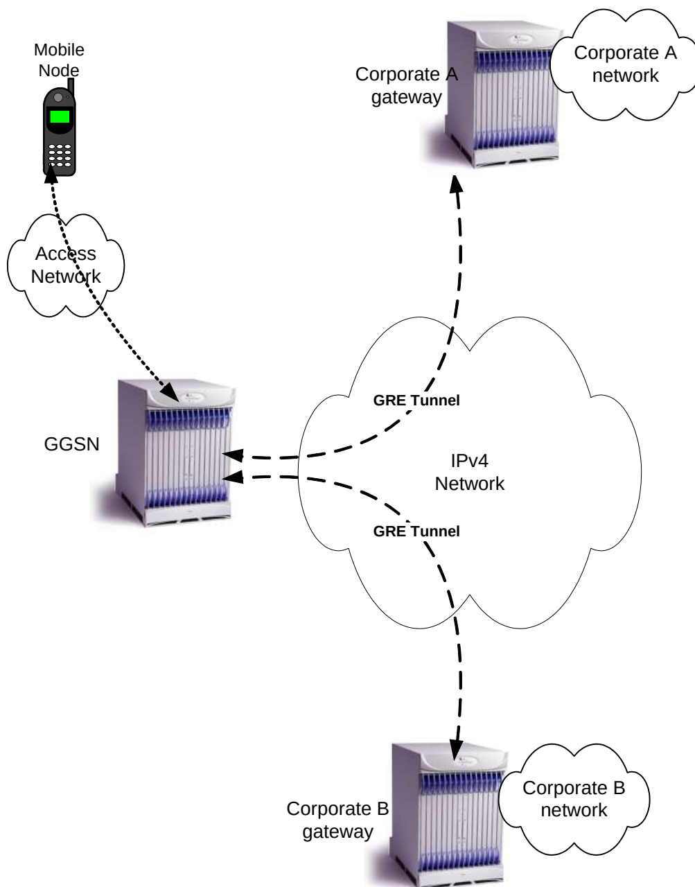
Figure 101. GRE Deployment Scenario
