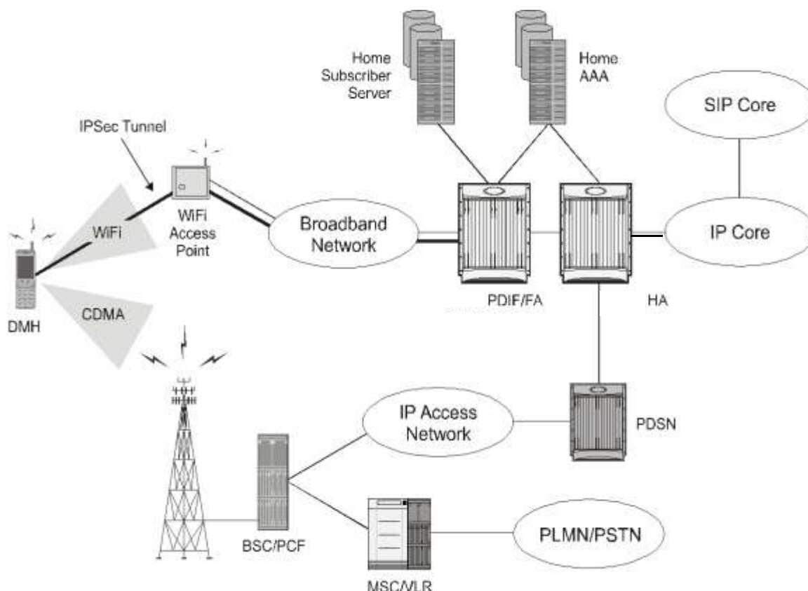
Figure 190. PDIF/FA Mobile IP Implementation
