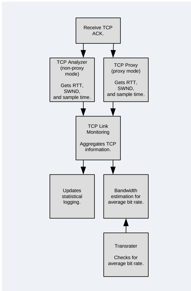
Figure 161. TCP Link Monitoring System Flow
