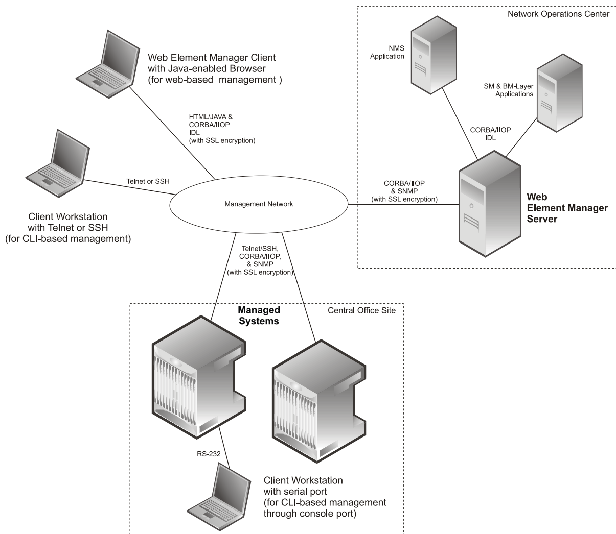
Figure 233. Element Management Methods
