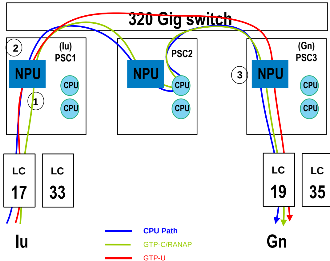
Figure 257. SGSN NPU FastPath
