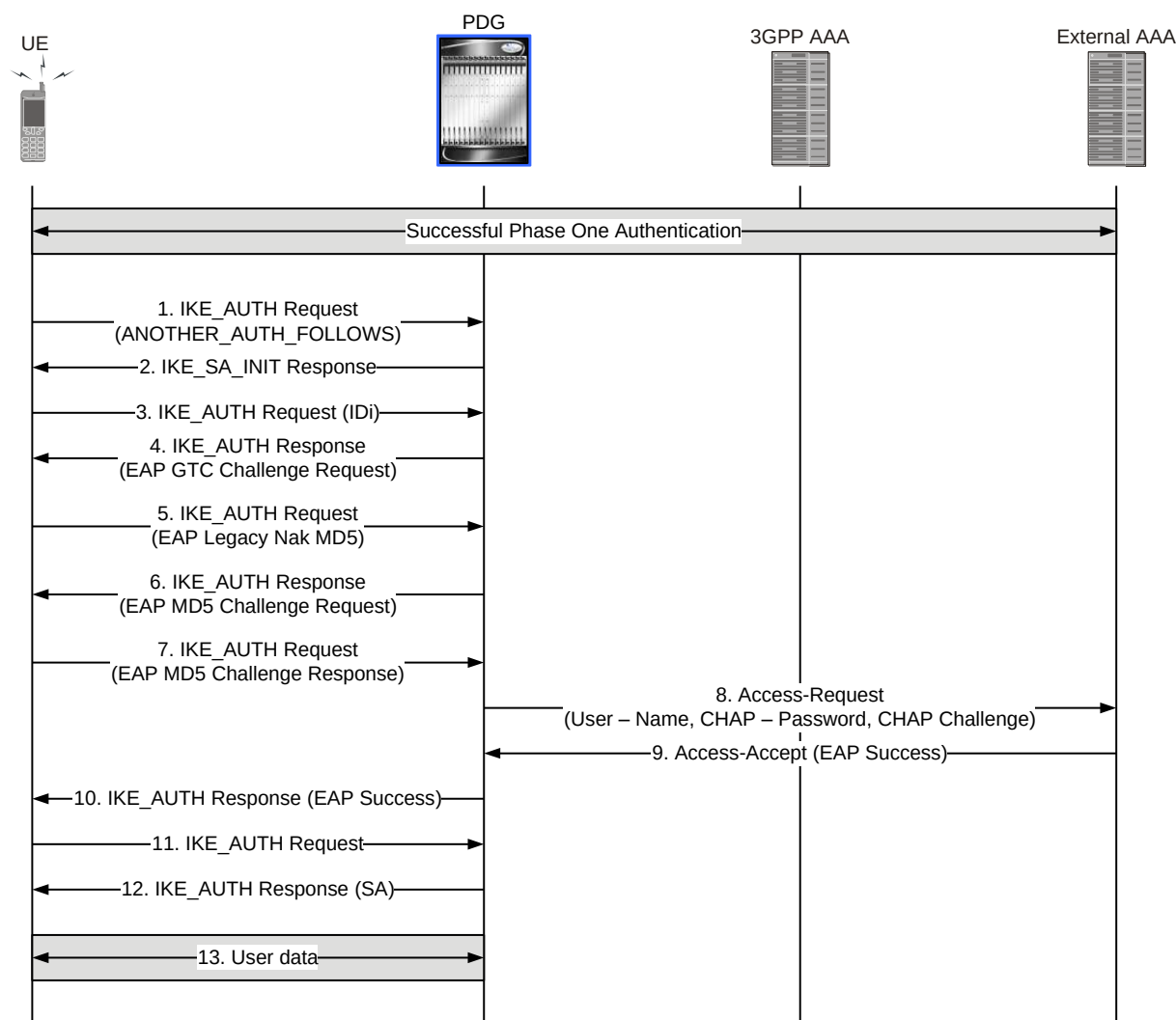
Figure 207. Multiple Authentication with Request from UE for Change of Second Phase Protocol
