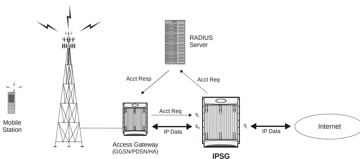
Figure 145. IPSG Message/Data Flow (RADIUS Snoop Mode)
