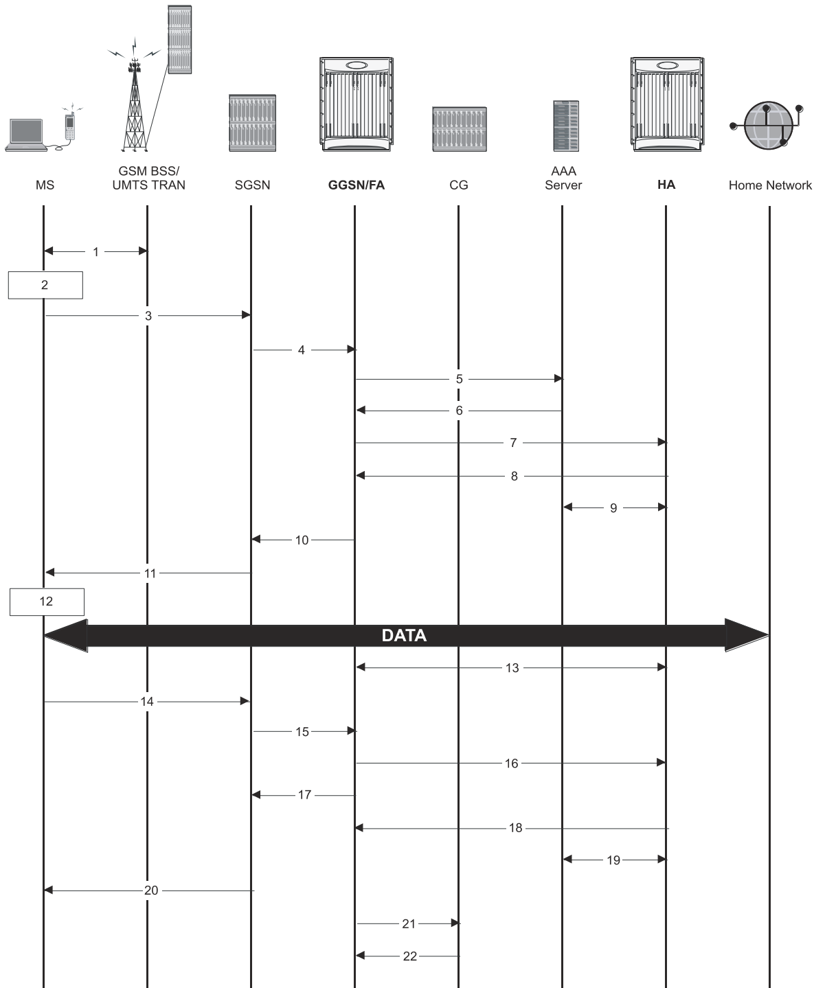
Figure 111. HA Assigned IP Address Proxy Mobile IP Call Flow
