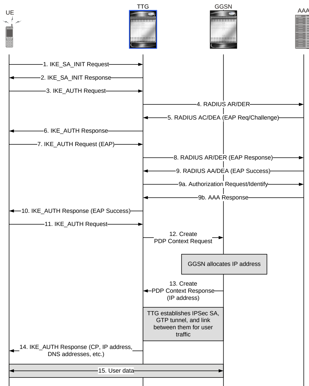
Figure 203. TTG Connection Establishment
