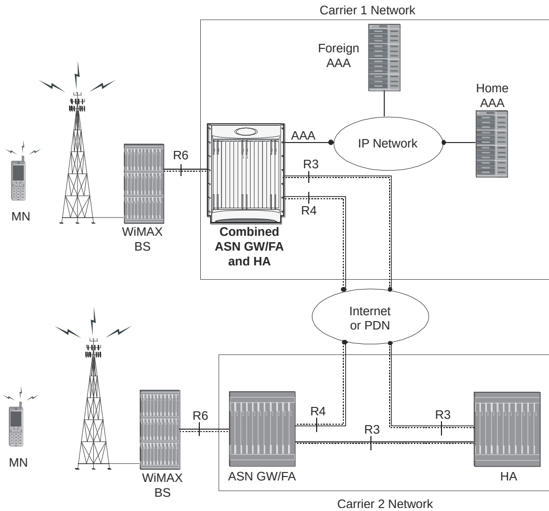
Figure 37. Co-located ASN Gateway/FA and HA Network Deployment Configuration Example
