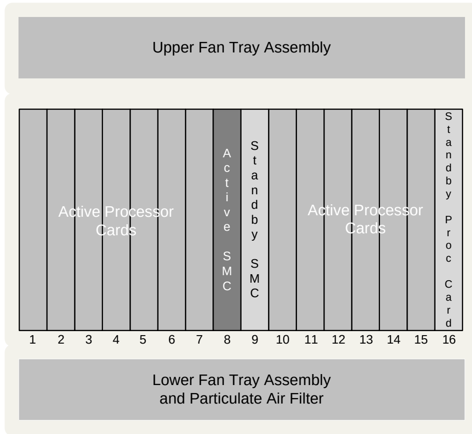
Figure 24. Recommended Redundant Configuration for Data Services - Front View
