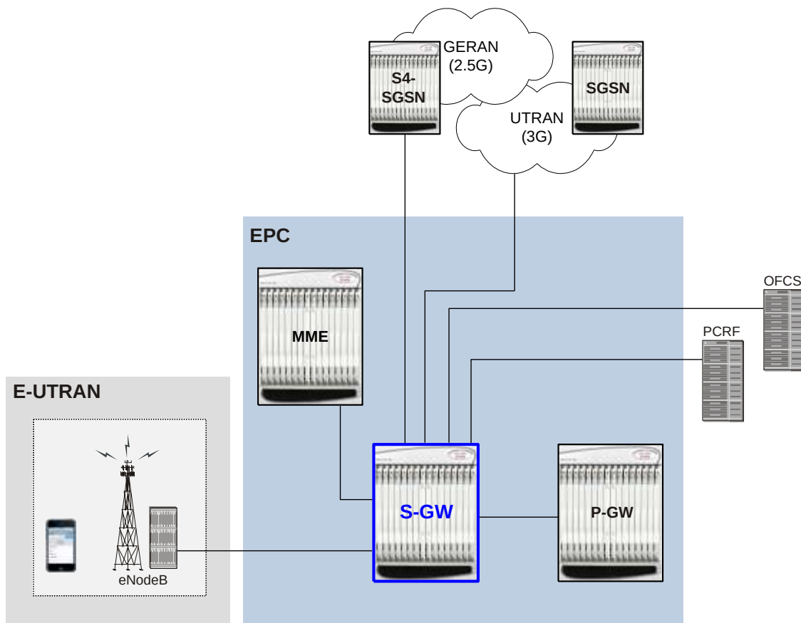
Figure 229. S-GW in the Basic E-UTRAN/EPC Network
