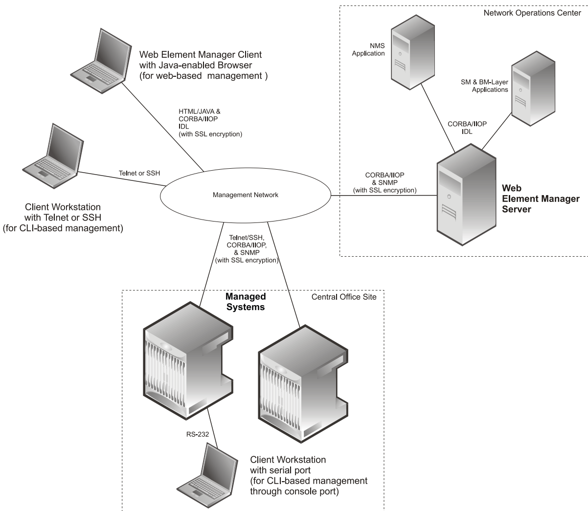
Figure 254. Element Management Methods
