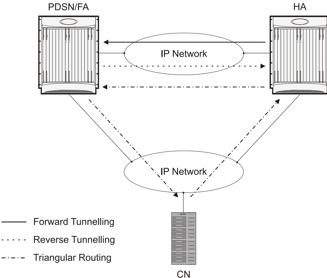
Figure 69. Mobile IP, FA and HA Tunneling/Transport Methods
