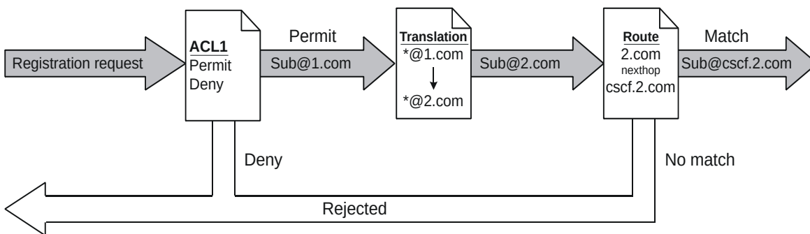
Figure 250. Admission and Routing Method
