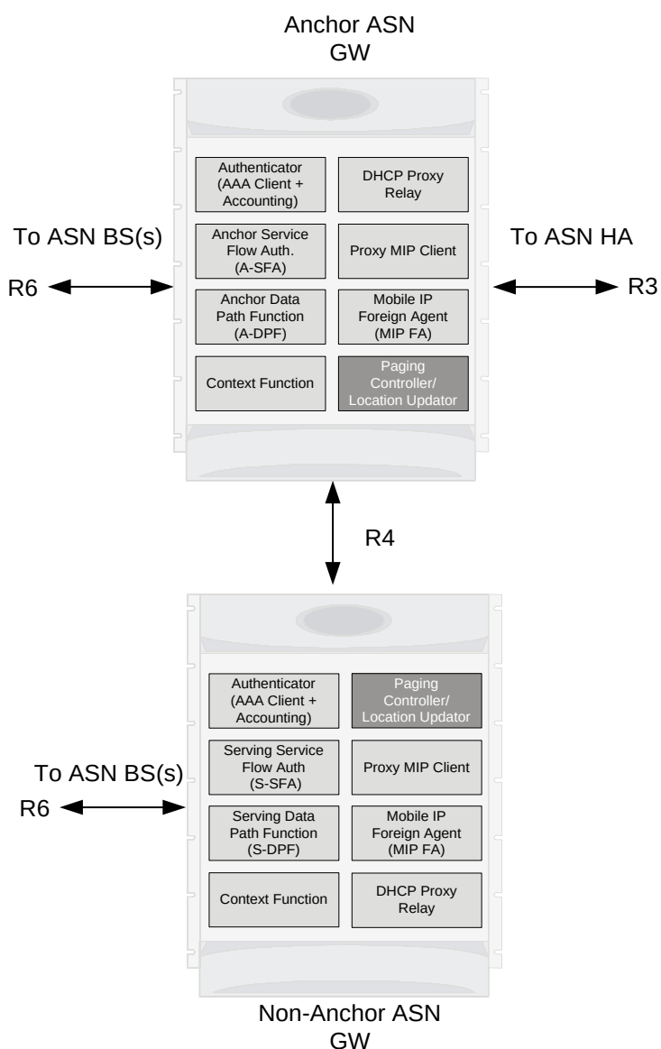
Figure 47. Distribution of Components and Function in ASN Gateway for Handover
