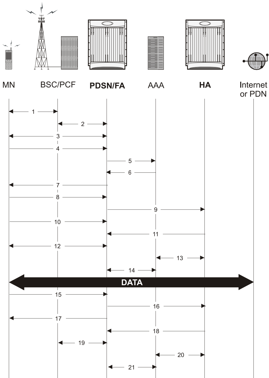
Figure 72. AAA/PDSN Assigned IP Address Proxy Mobile IP Call Flow
