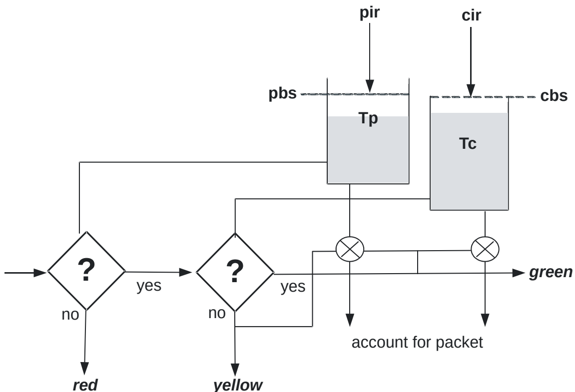
Figure 258. TCM Algorithm Logic for Traffic Policing
