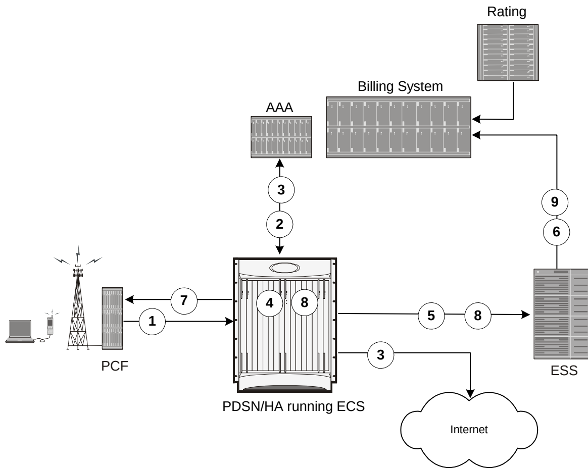
Figure 88. Postpaid Billing with ECS in CDMA-2000 Network
