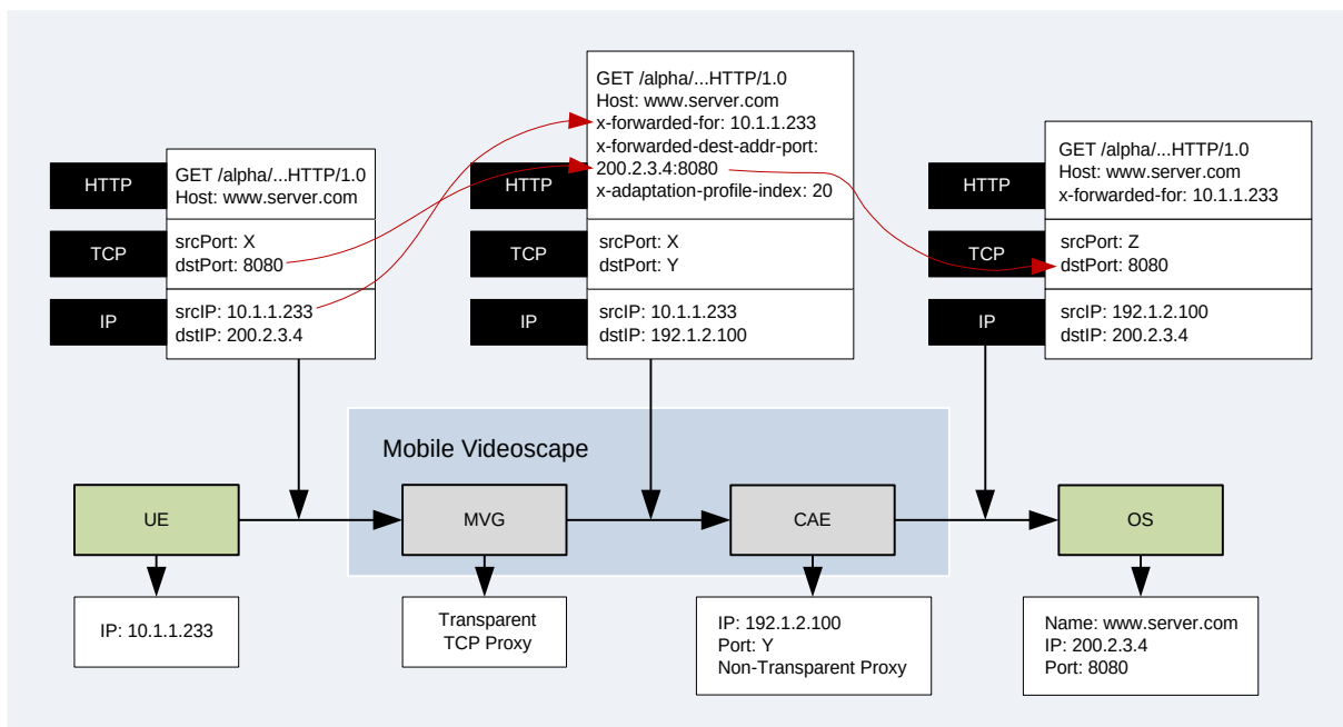
Figure 152. HTTP X-Header Use in Transparent Video Re-addressing
