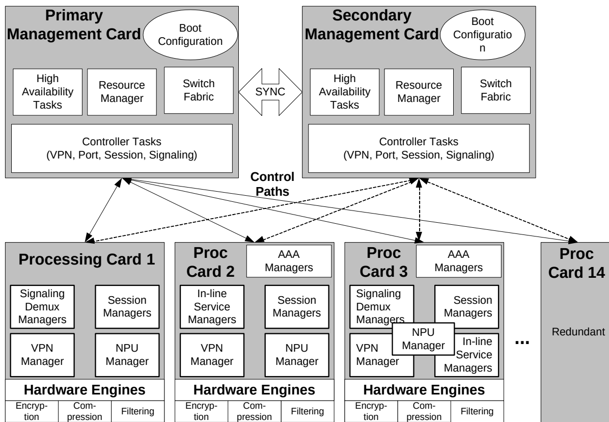
Figure 23. Software Architecture Block Diagram
