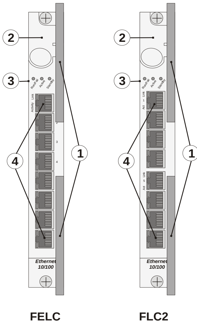
Figure 16. Fast Ethernet Line Card (FELC/FLC2)
