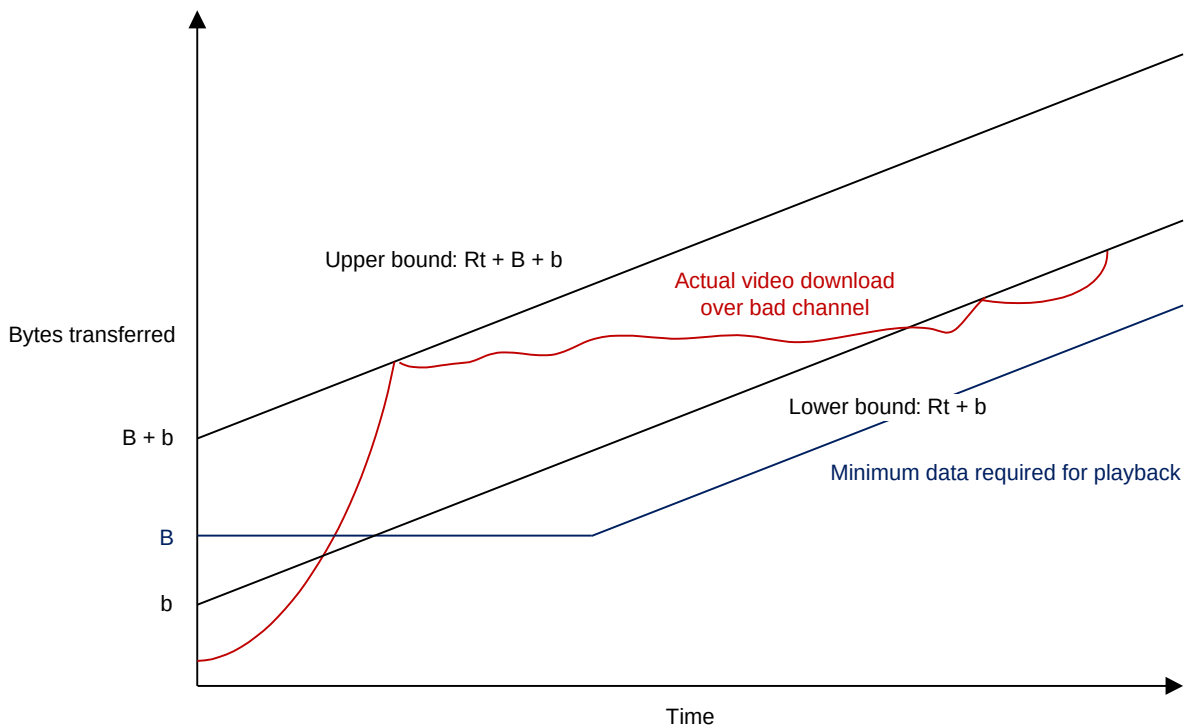
Figure 158. Video Pacing During Bad Channel Conditions
