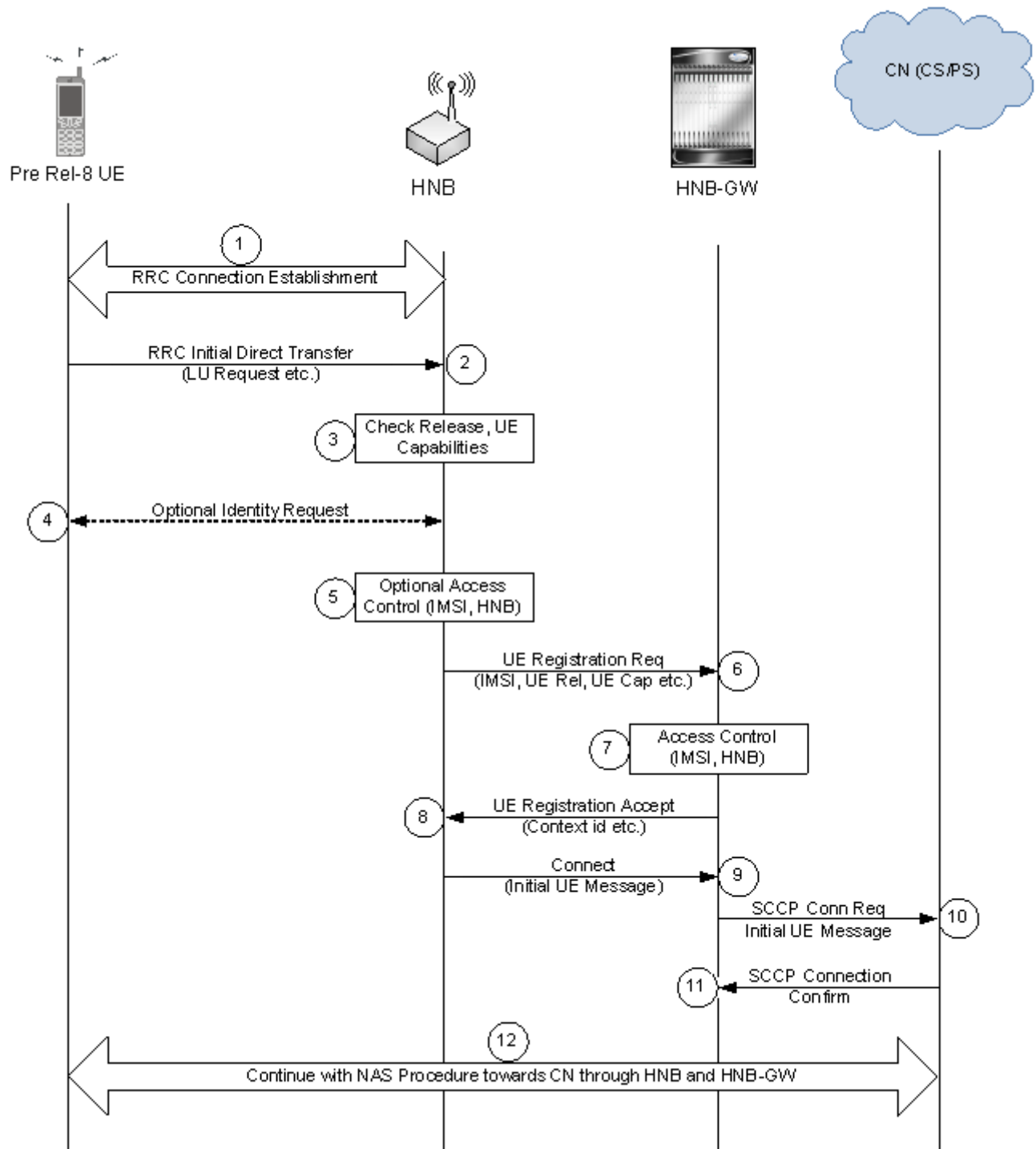
Figure 123. UE Registration Call Flow for Non-CSG UEs or Non-CSG HNBs
