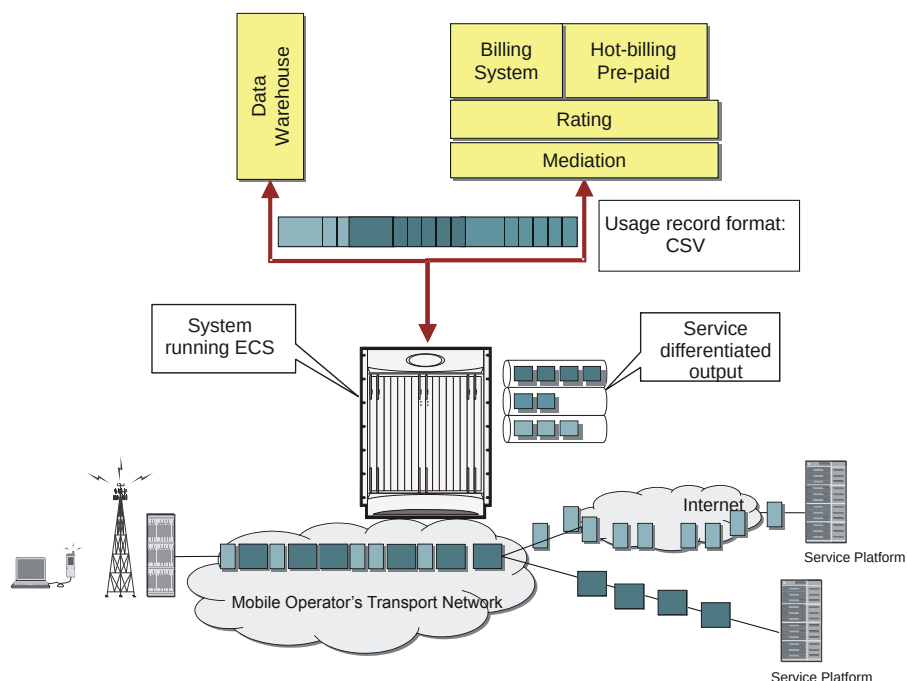
Figure 82. Deployment of ECS in a Mobile Data Network
