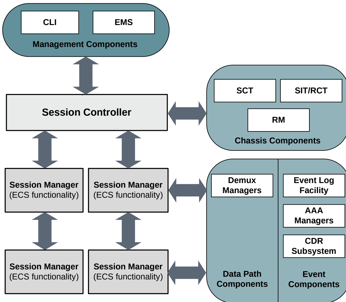
Figure 83. ECS Architecture
