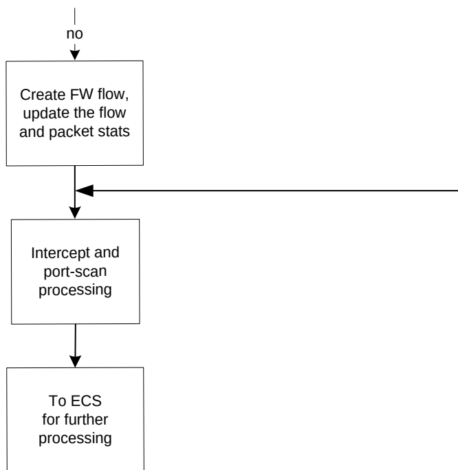
Figure 225. Continued... Stateful Firewall Processing
