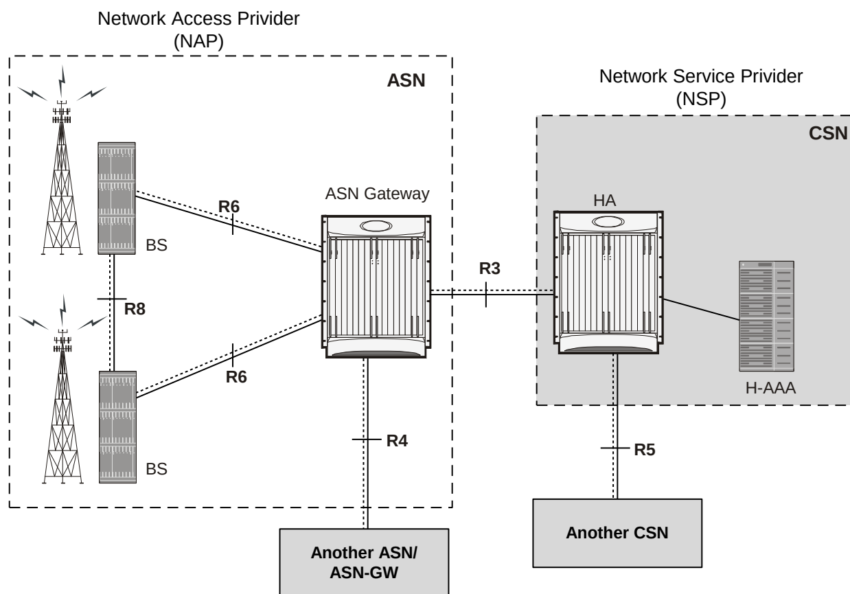
Figure 34. ASN Network Reference Model with ASN Gateway
