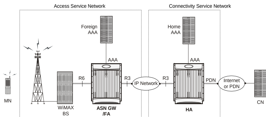
Figure 36. ASN Gateway/FA and HA Network Deployment Configuration Example
