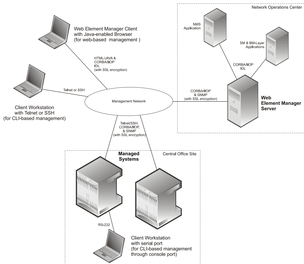
Figure 26. Element Management Methods
