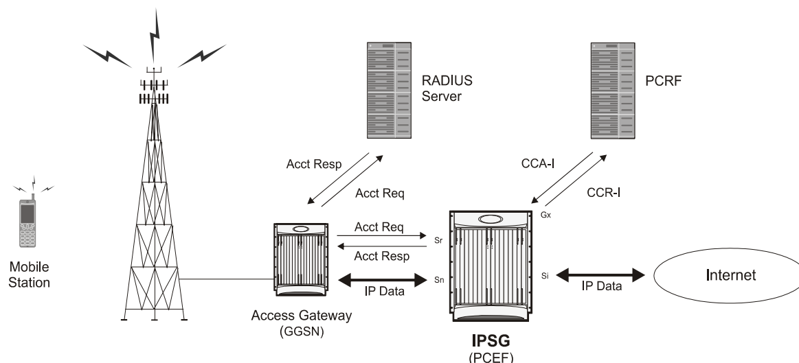
Figure 146. IPSG Message/Data Flow (RADIUS Server Mode - IMS Auth Service)
