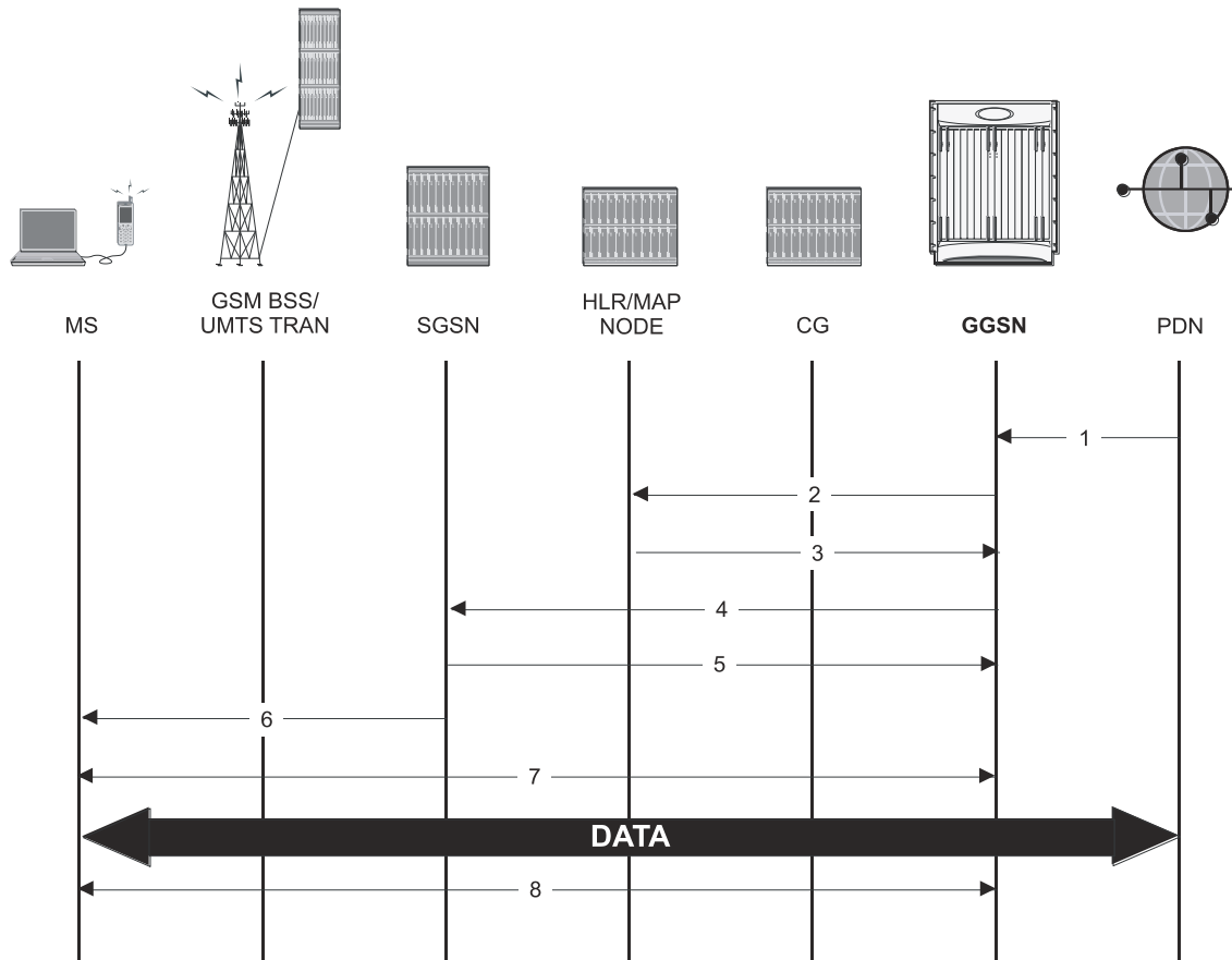
Figure 106. Network-initiated Session Call Flow
