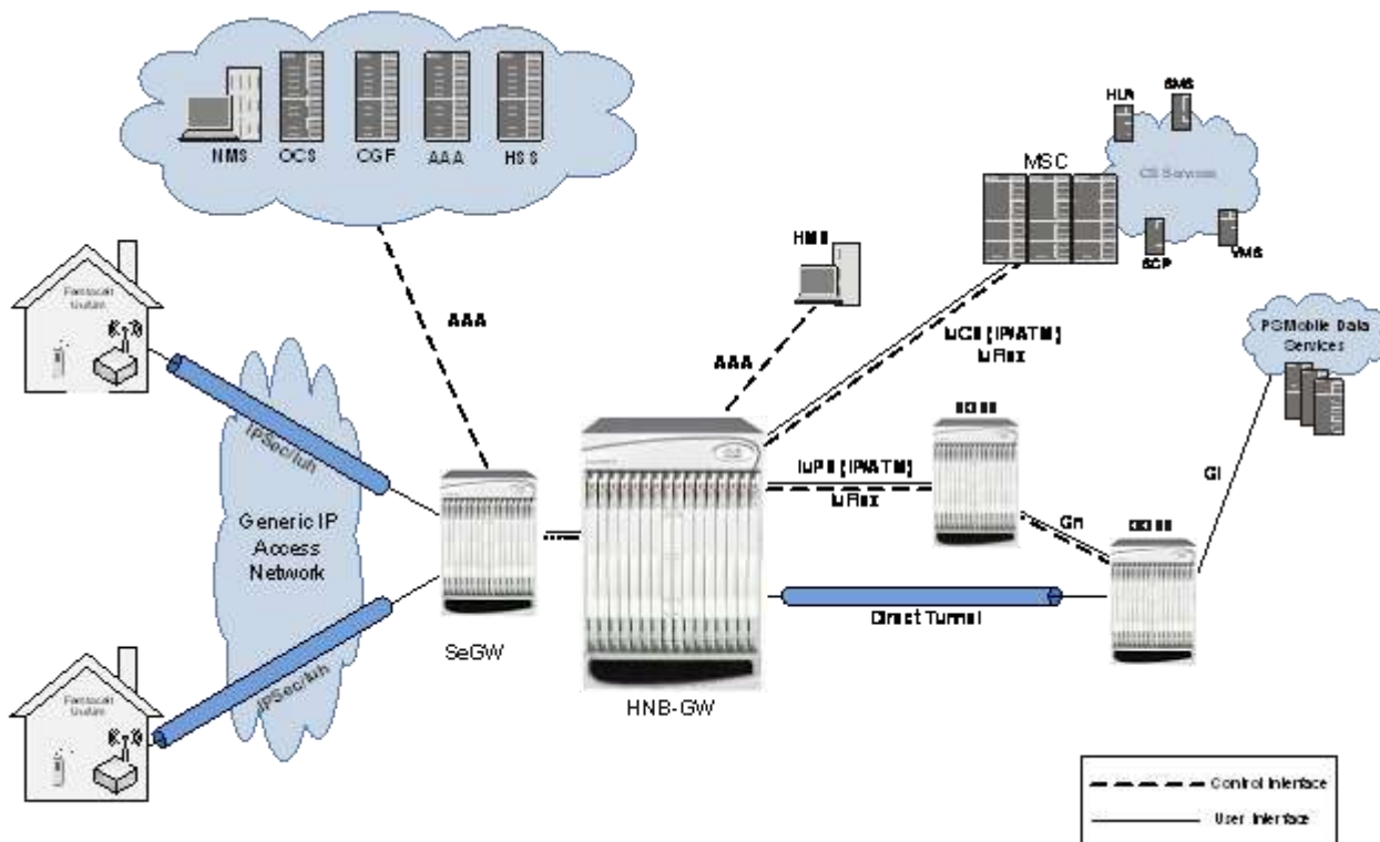
Figure 118. HNB-GW Deployment in 3G UMTS Network
