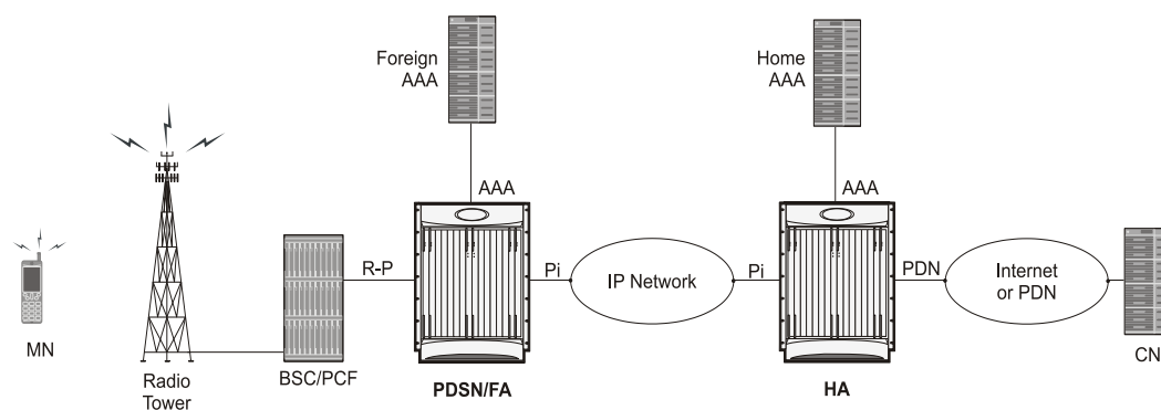
Figure 113. PDSN/FA and HA Network Deployment Configuration Example
