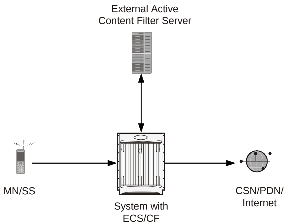
Figure 77. High-Level View of Streamlined ICAP Interface with External ACF
