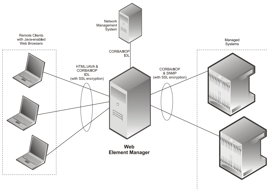
Figure 121. Web Element Manager Network Interfaces
