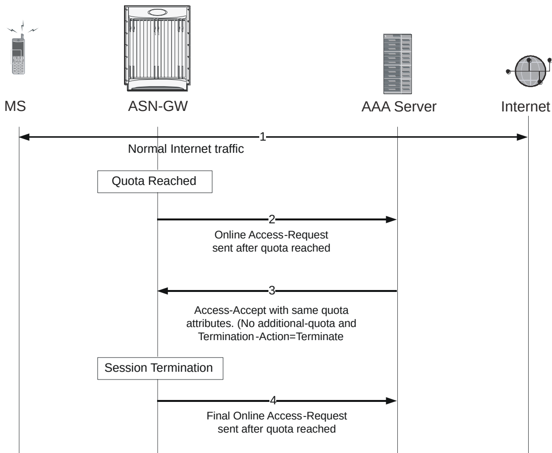
Figure 54. Call Flow for Terminating the Call on Quota-Reach
