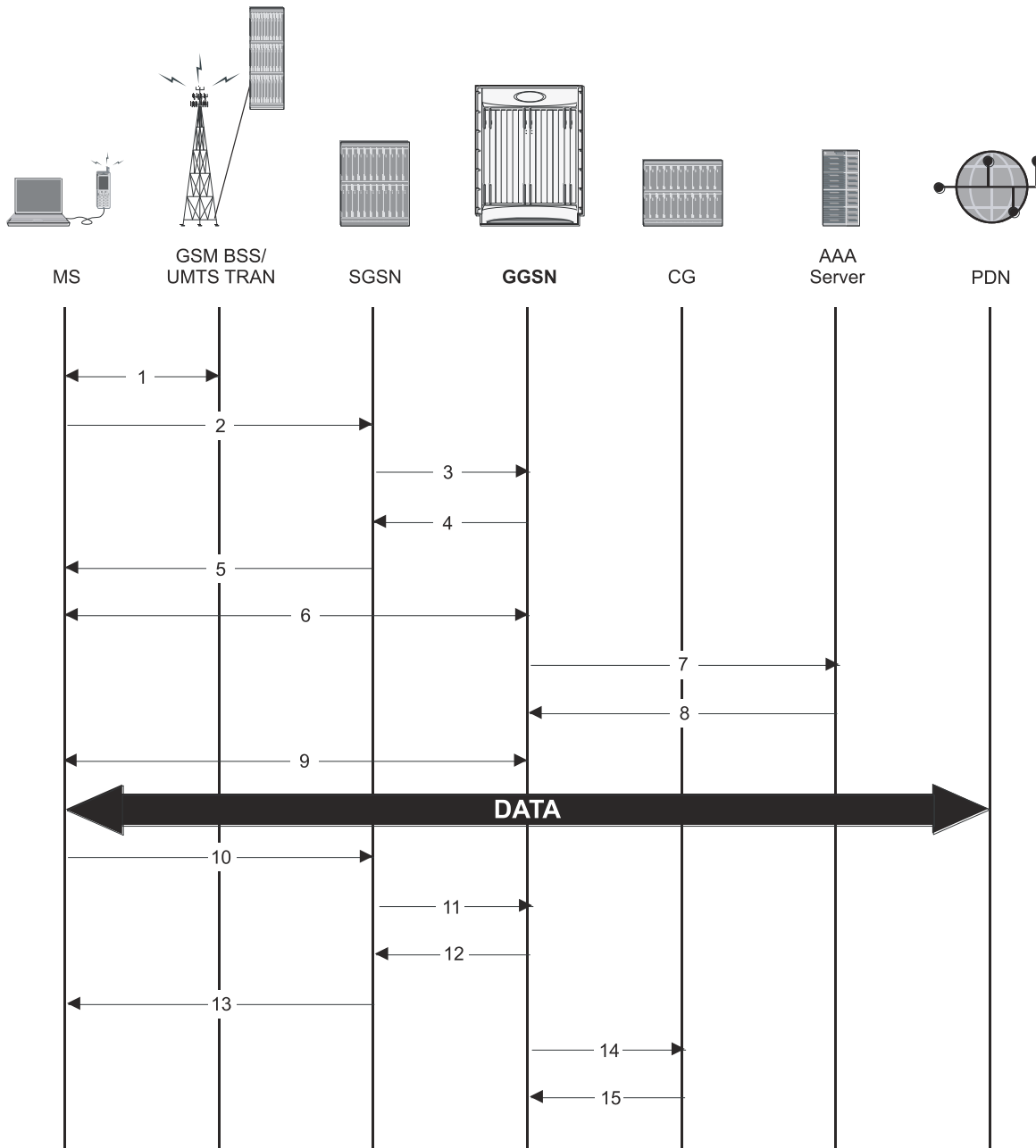
Figure 107. PPP Direct Access Call Flow
