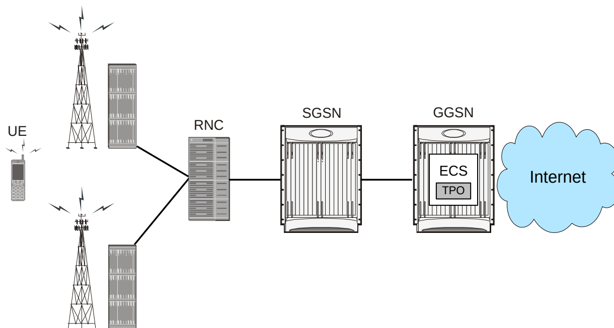
Figure 266. TPO Deployment
