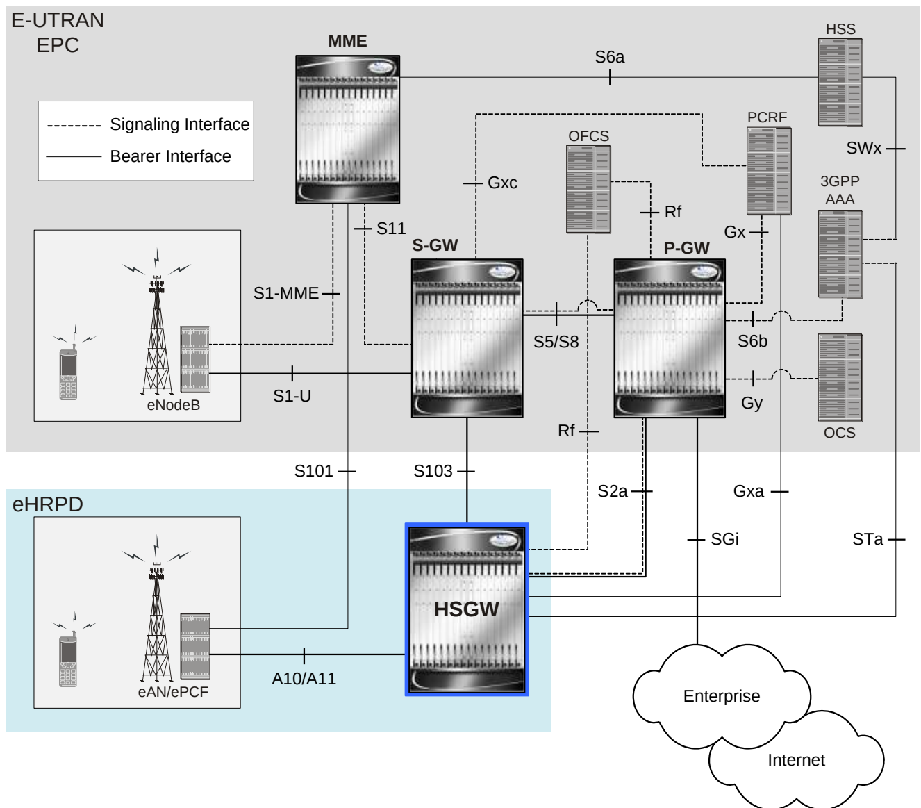
Figure 127. HSGW in an eHRPD Network Architecture
