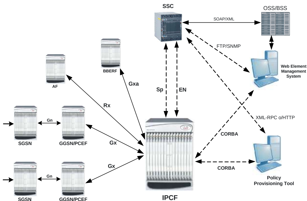
Figure 137. Co-located PCEF and IPCF in UTRAN/E-UTRAN Networks
