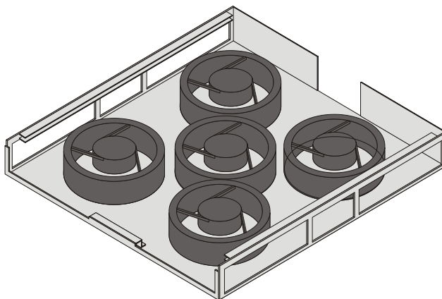
Figure 9. Lower Fan Tray
