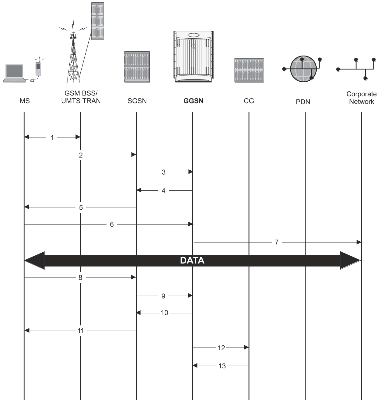
Figure 109. Corporate IP VPN Connectivity Call Flow
