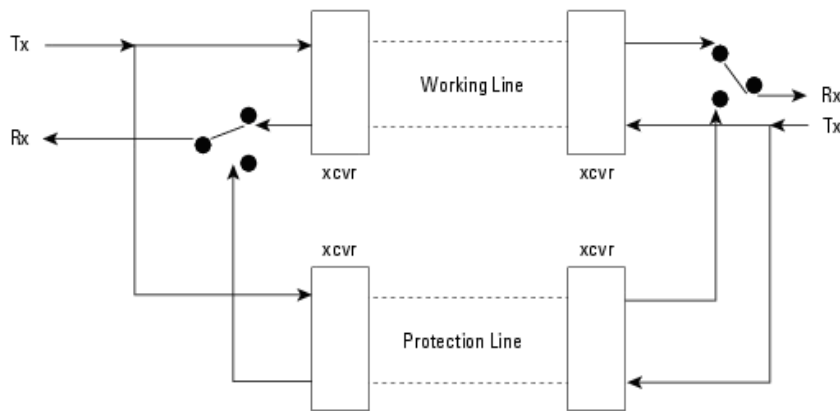
Figure 253. SONET APS 1+1
