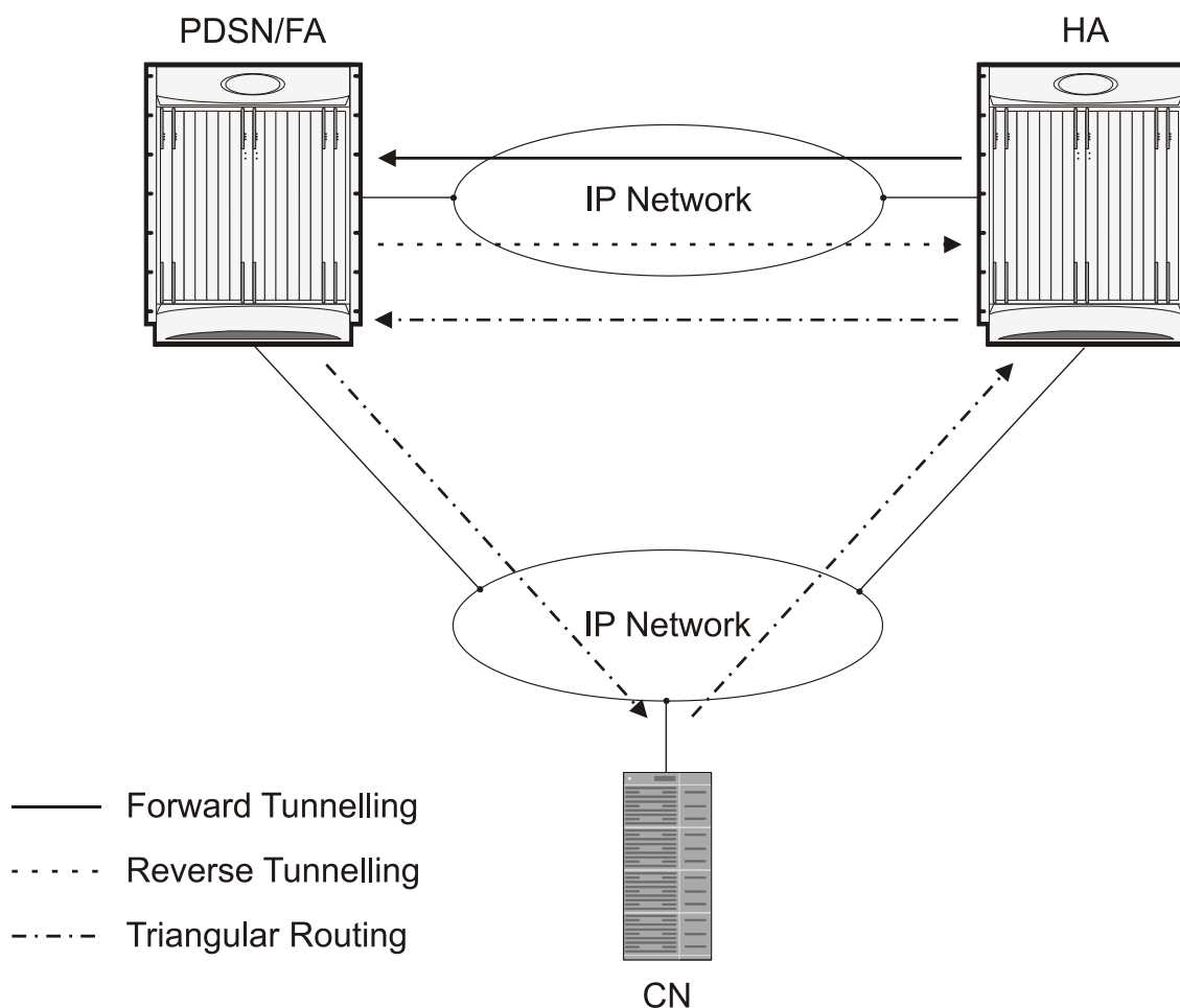
Figure 115. Mobile IP, FA and HA Tunneling/Transport Methods.
