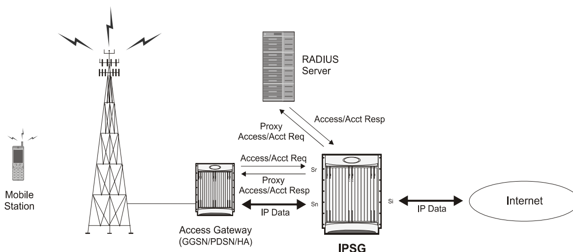
Figure 144. IPSG Message/Data Flow (RADIUS Server Mode - RADIUS Proxy)
