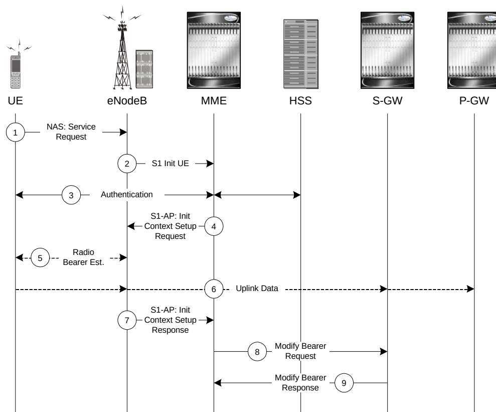
Figure 179. UE-initiated Service Request Message Flow
