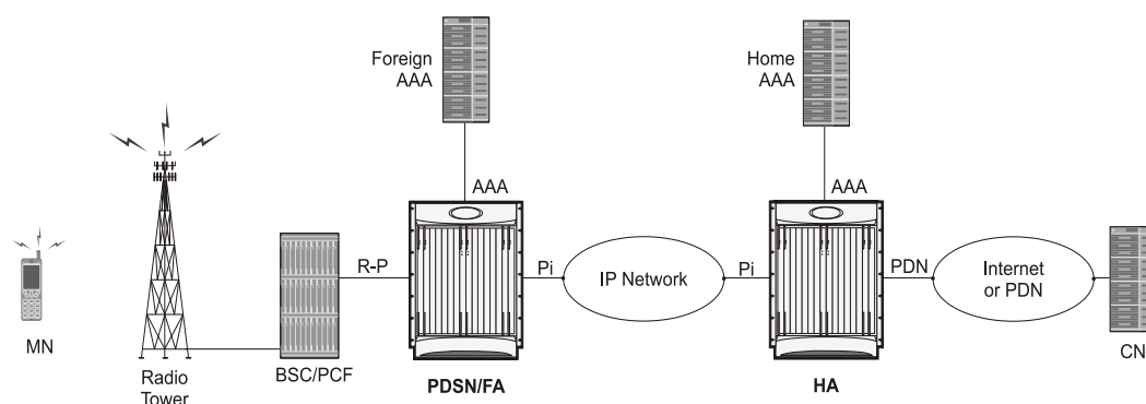
Figure 65. PDSN/FA and HA Network Deployment Configuration Example
