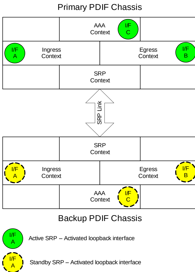
Figure 197. Loopback Interface Configuration
