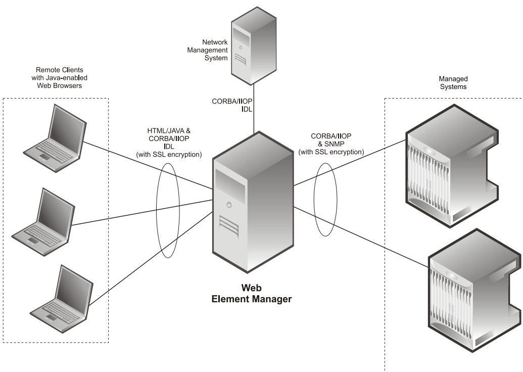
Figure 215. Web Element Manager Network Interfaces
