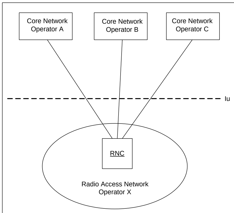
Figure 256. MOCN-type Network Sharing
