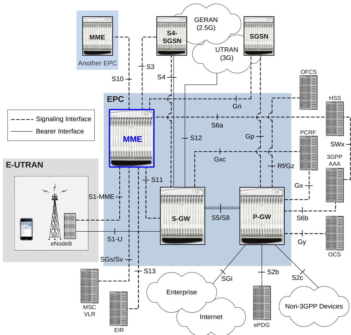
Figure 172. E-UTRAN/EPC Network Scenario
