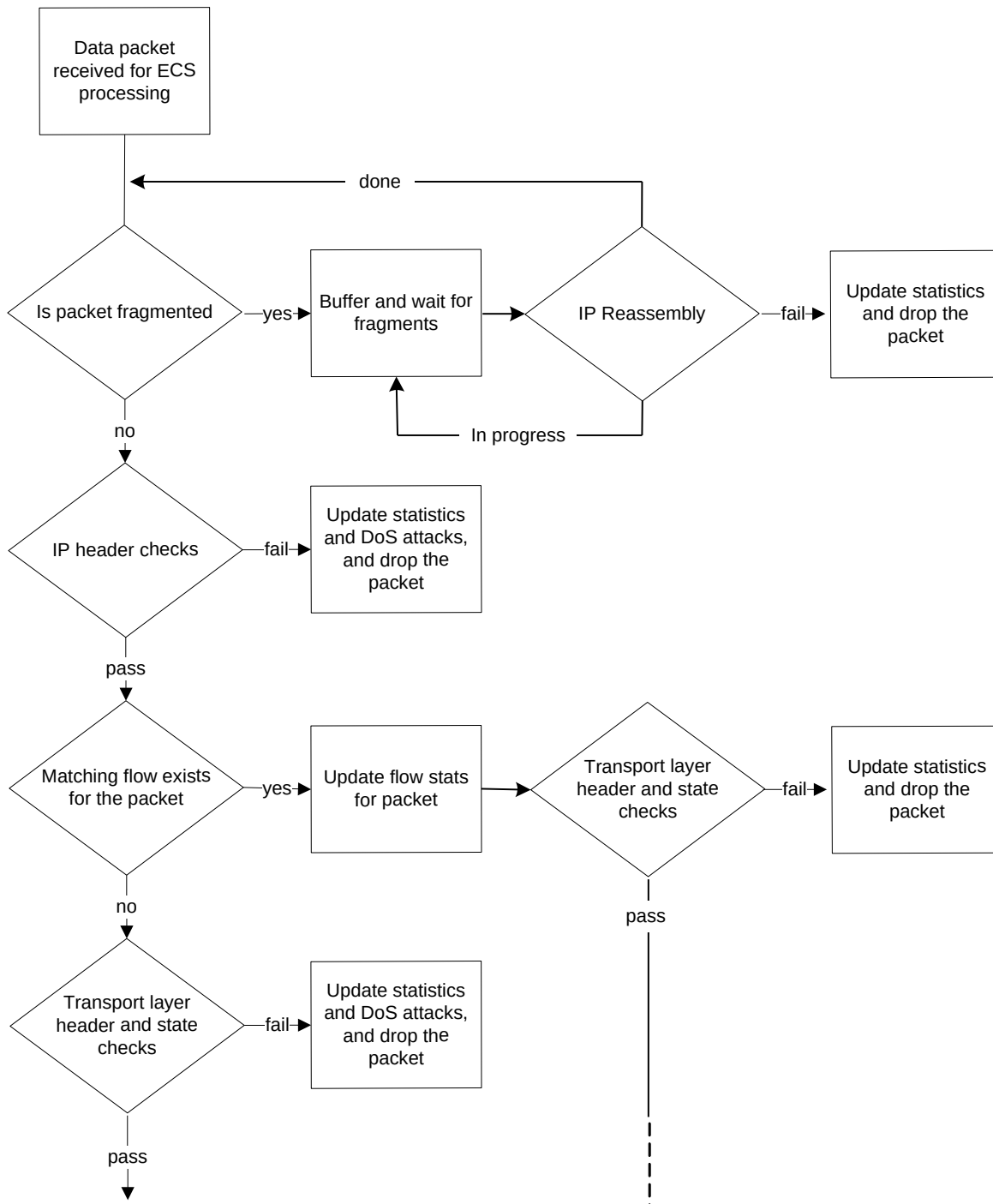
Figure 223. Stateful Firewall Processing
