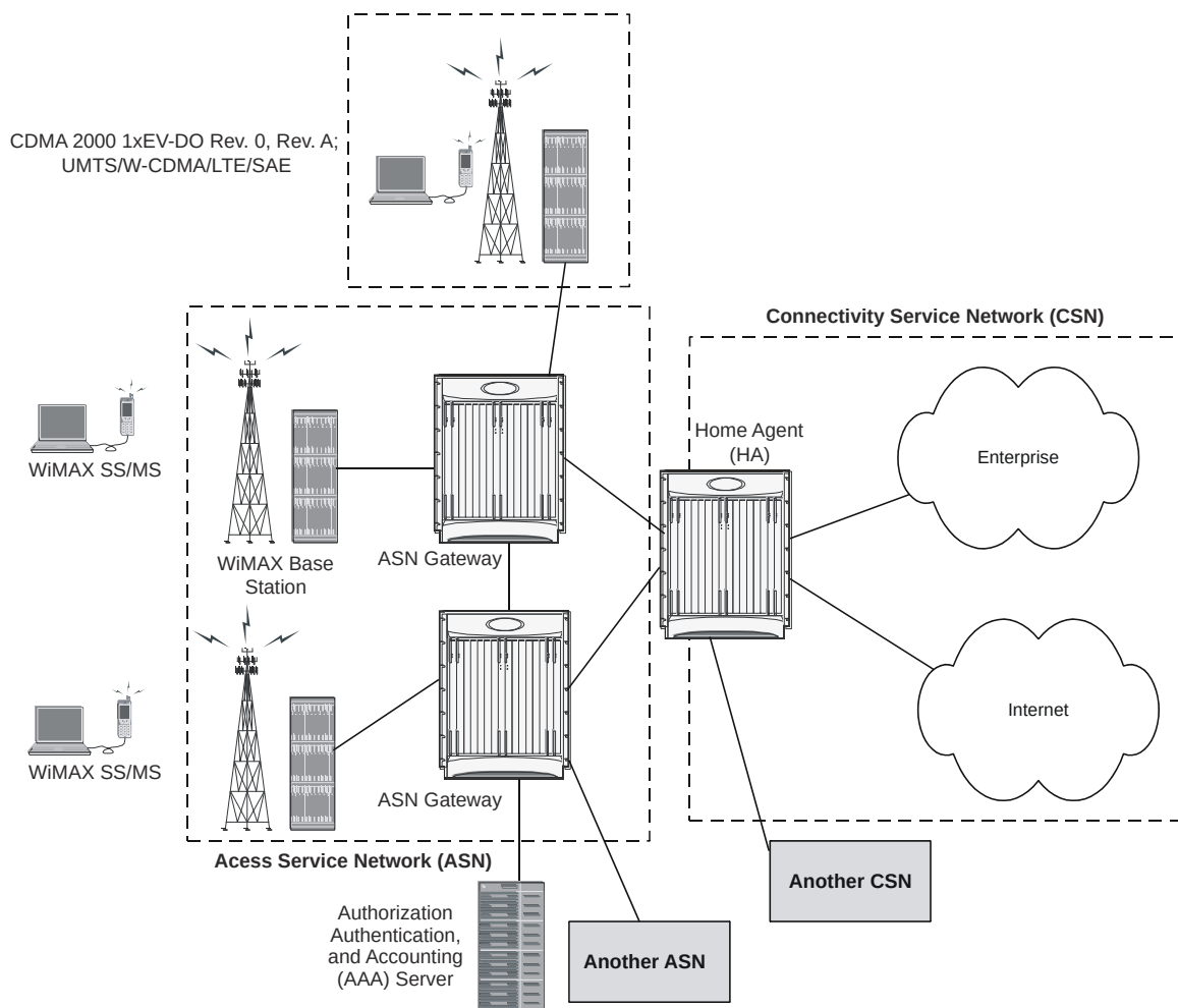
Figure 33. WiMAX Network Architecture
