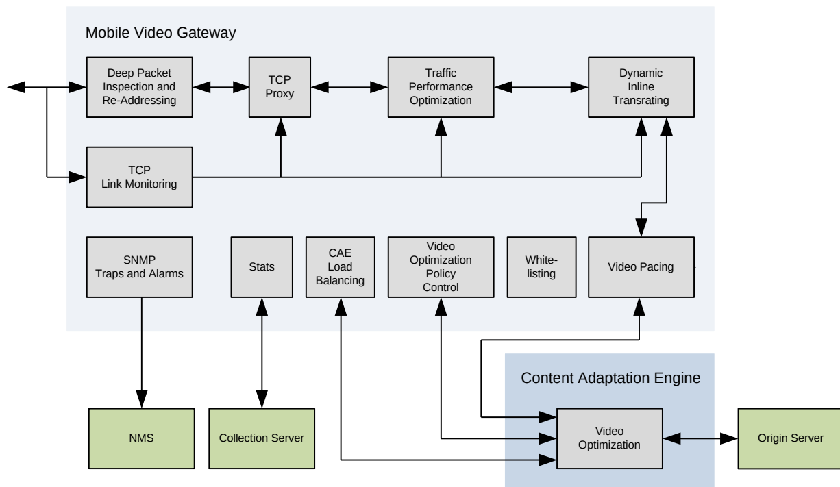
Figure 147. Mobile Video Gateway Features and Functions
