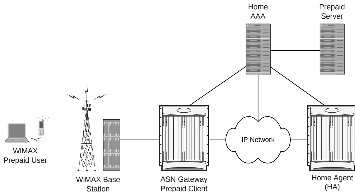
Figure 31. Prepaid Network Topology
