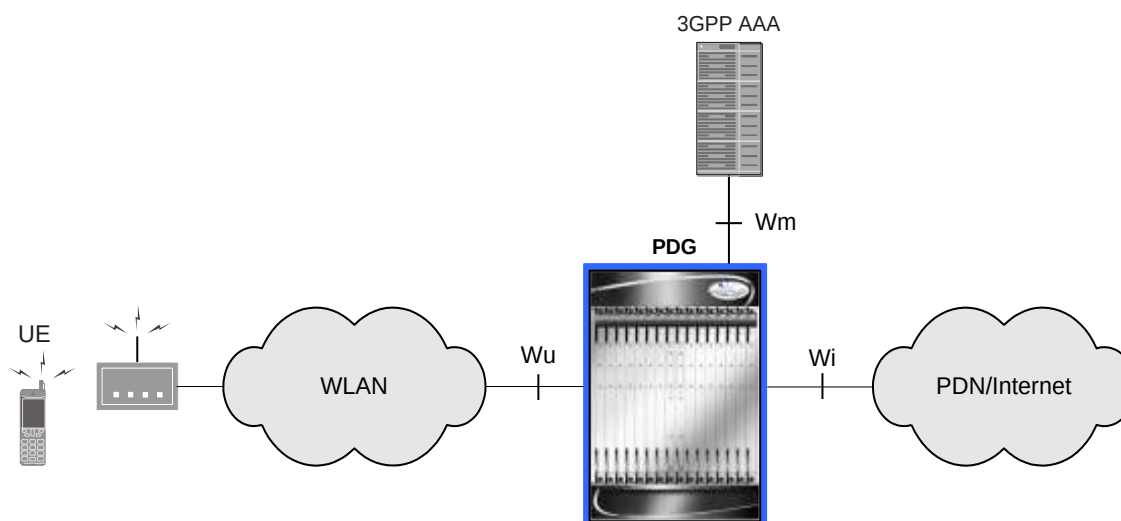
Figure 200. Sample PDG Implementation
