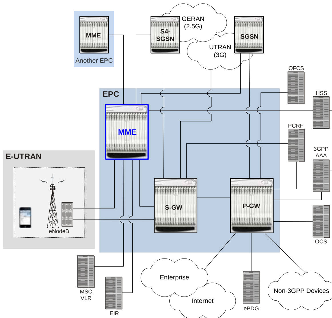
Figure 170. MME in the E-UTRAN/EPC Network Topology
