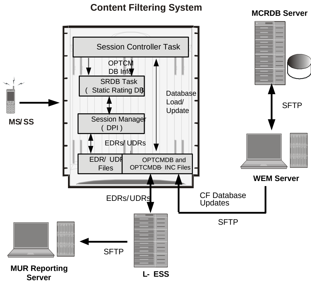
Figure 75. High-Level Architecture of Category-based Content Filtering
