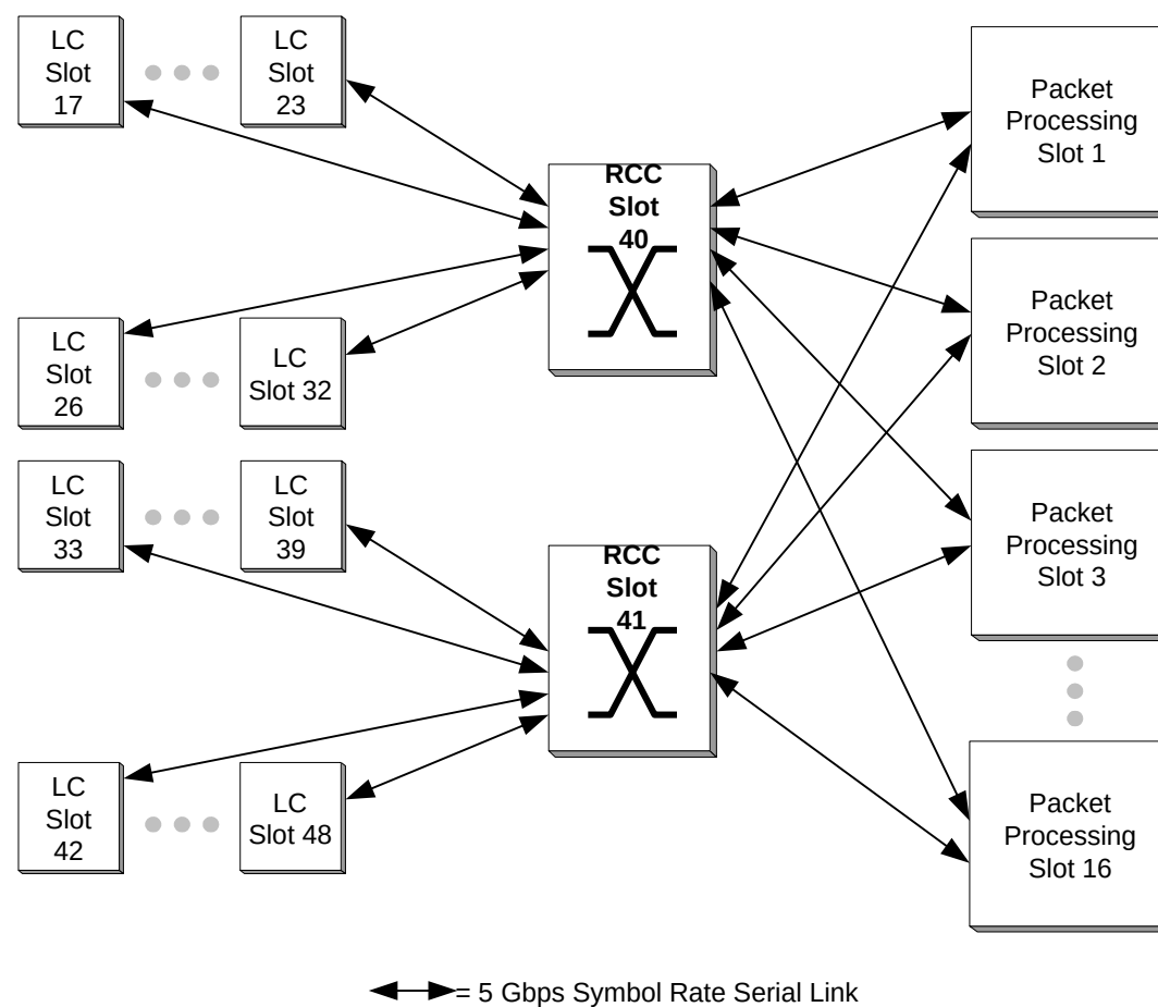
Figure 7. RCC Logical View
