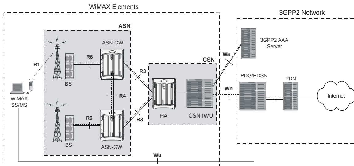
Figure 58. ASN Gateway with 3GPP2 Overlay
