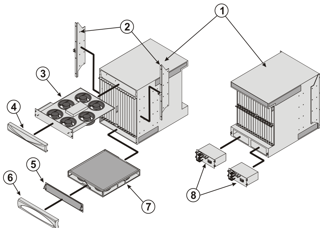
Figure 3. Chassis Components (front and rear views)
