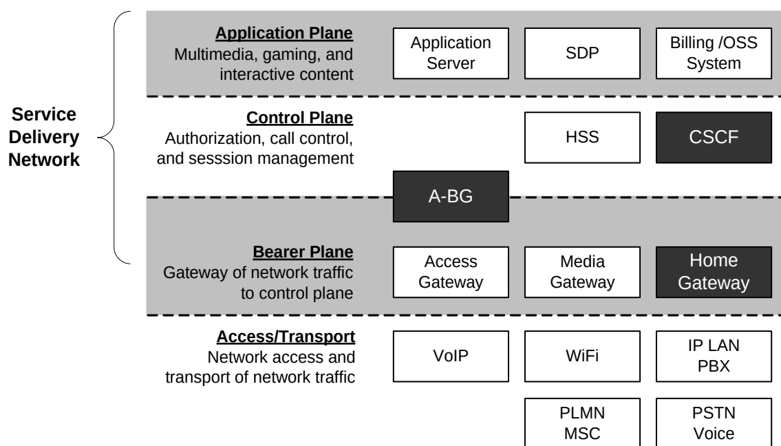
Figure 238. IMS Service Delivery Networks Components
