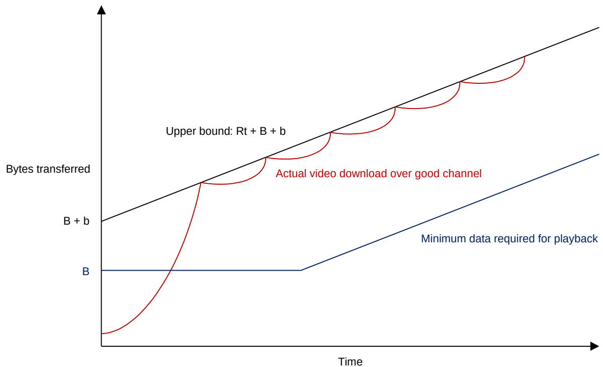
Figure 157. Video Pacing During Good Channel Conditions
