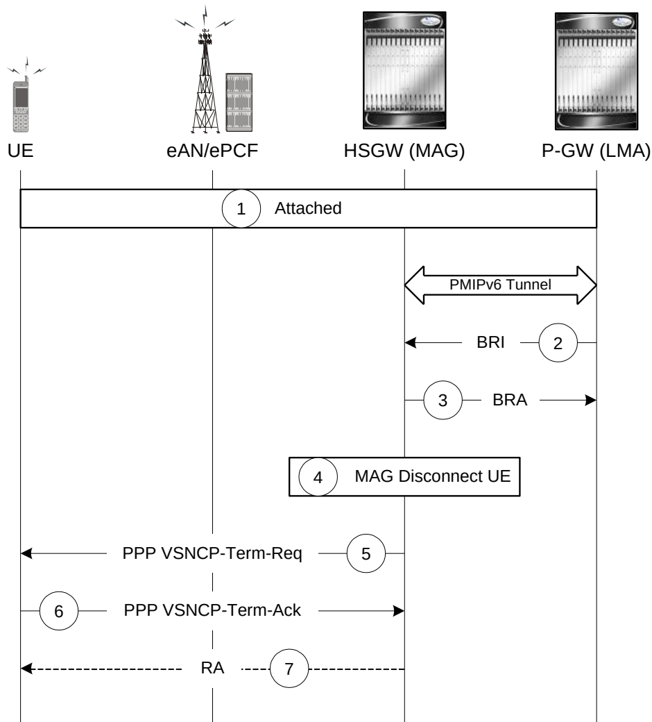
Figure 220. PDN Connection Release by the P-GW Call Flow
