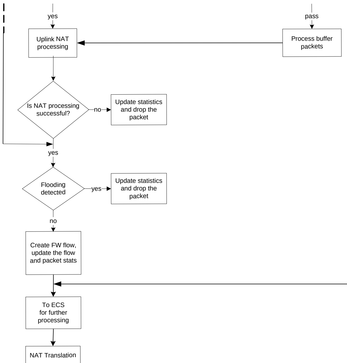
Figure 188. ... NAT Processing Flow
