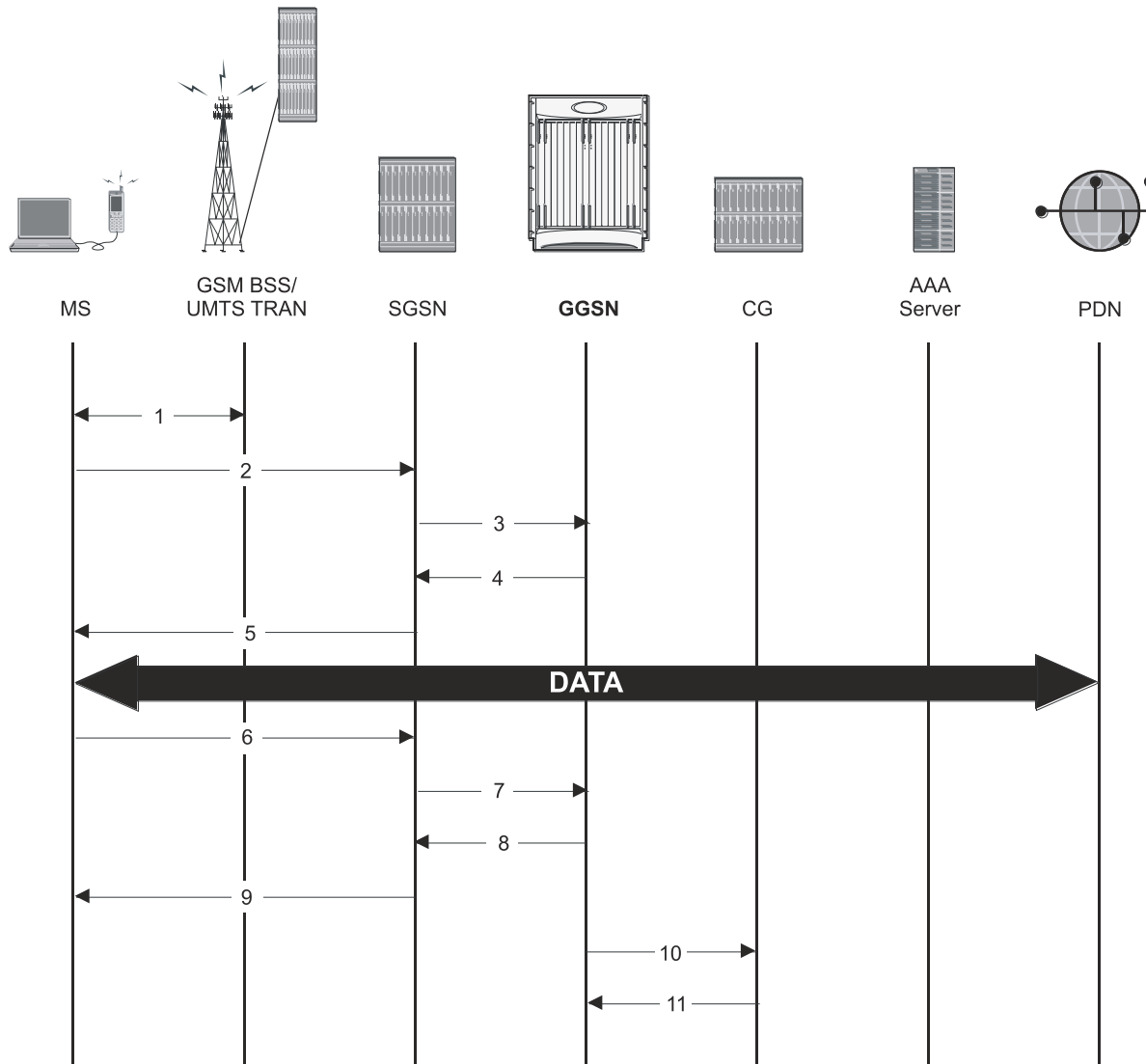
Figure 104. Transparent IP Session Call Flow
