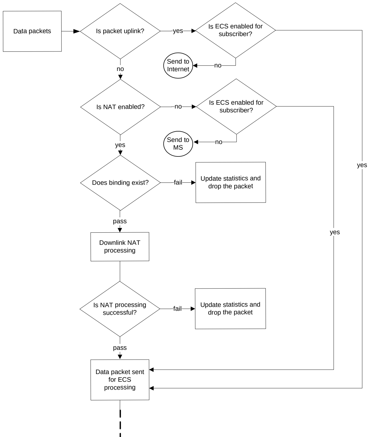
Figure 185. NAT Processing Flow
