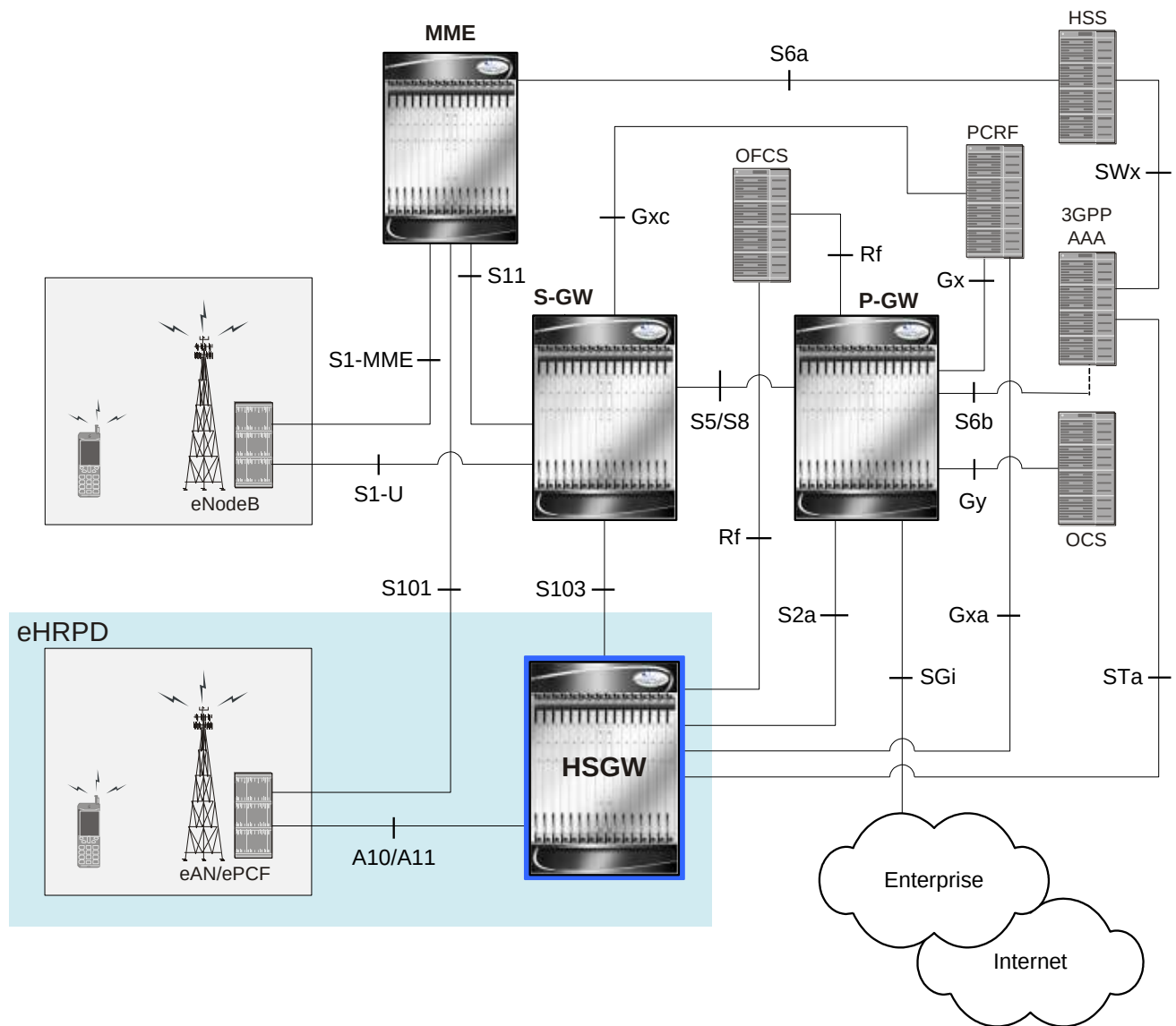
Figure 126. eHRPD Basic Network Topology
