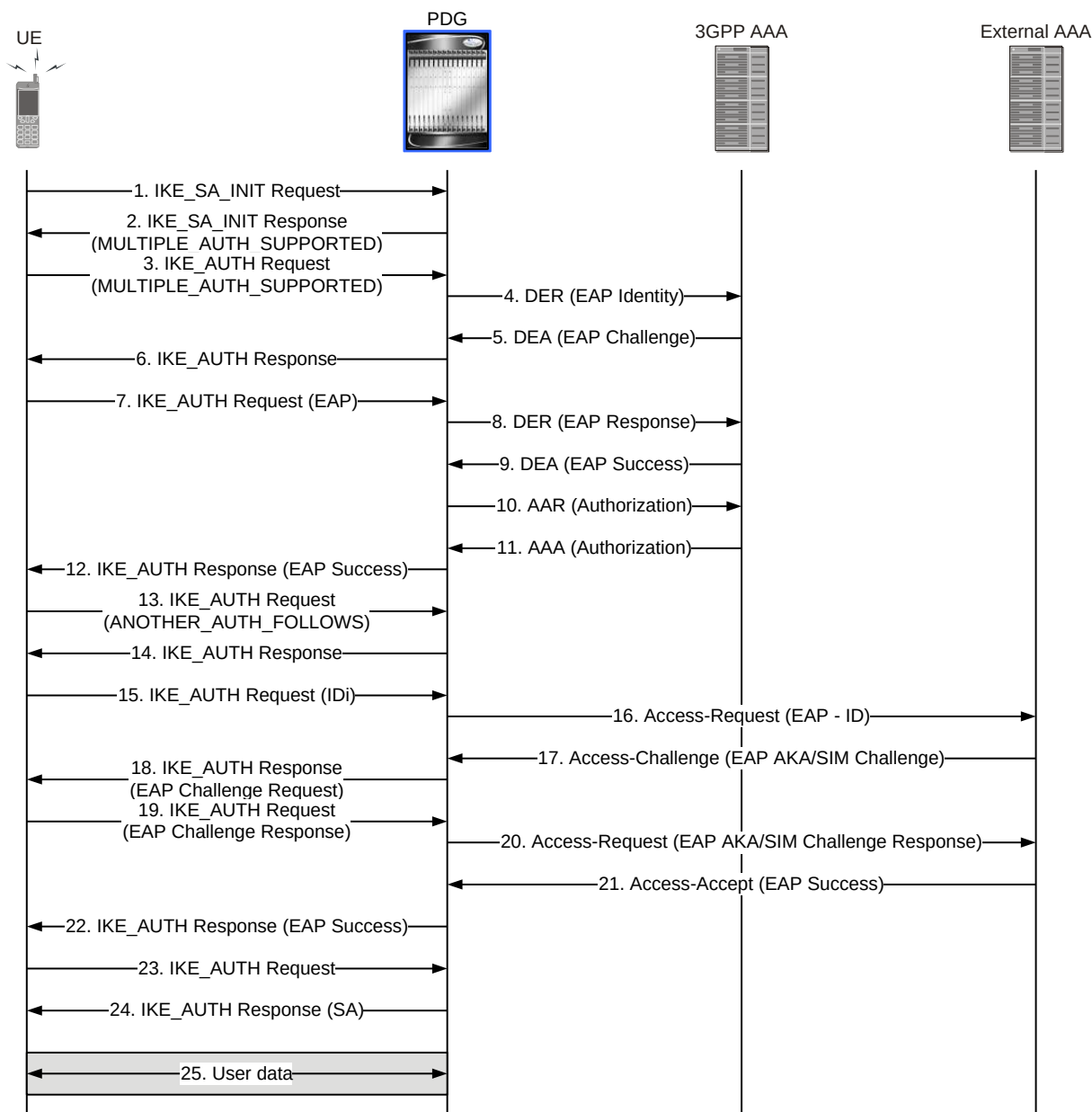
Figure 206. Multiple Authentication Using EAP and EAP
