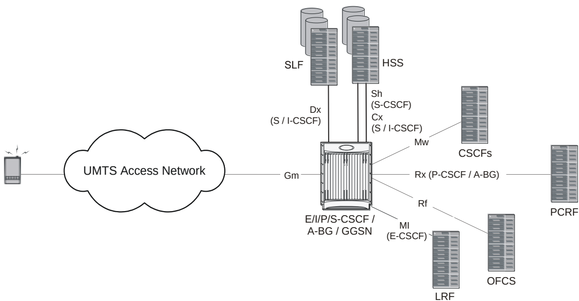
Figure 242. GSM/UMTS CSCF/A-BG/GGSN SCM Deployment Example
