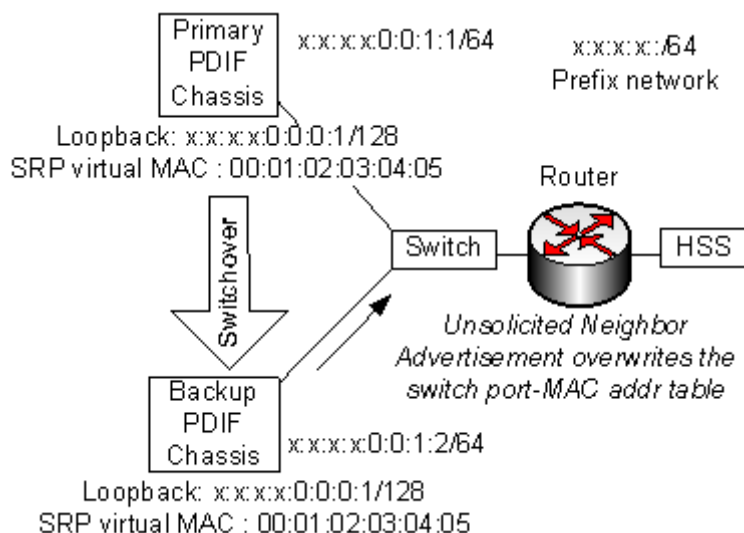
Figure 199. Switchover Example for a Common IPv6 Subnet
