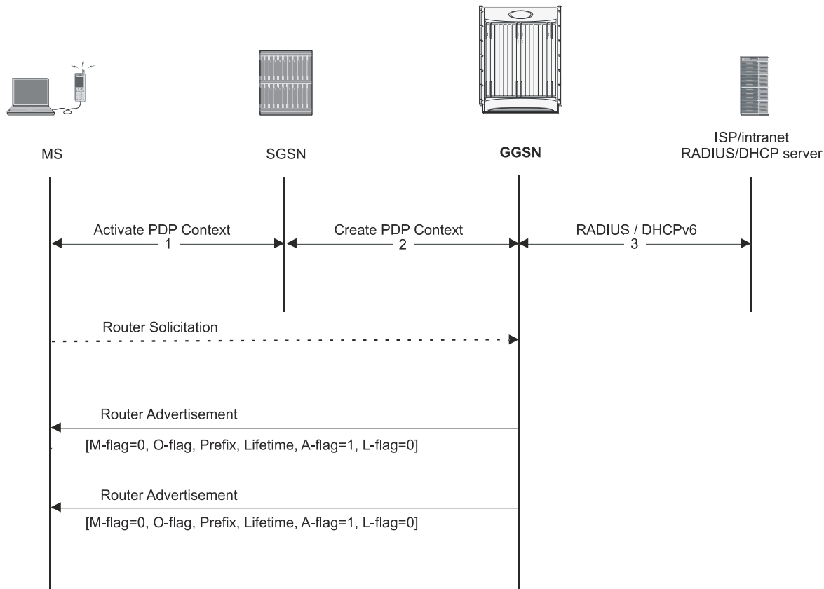
Figure 112. IPv6 Stateless Address Auto Configuration Flow
