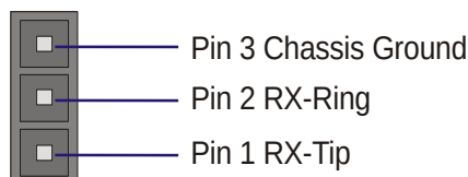
Figure 281. SPIO T1 BITS Timing Wire-Wrap Pin-out
