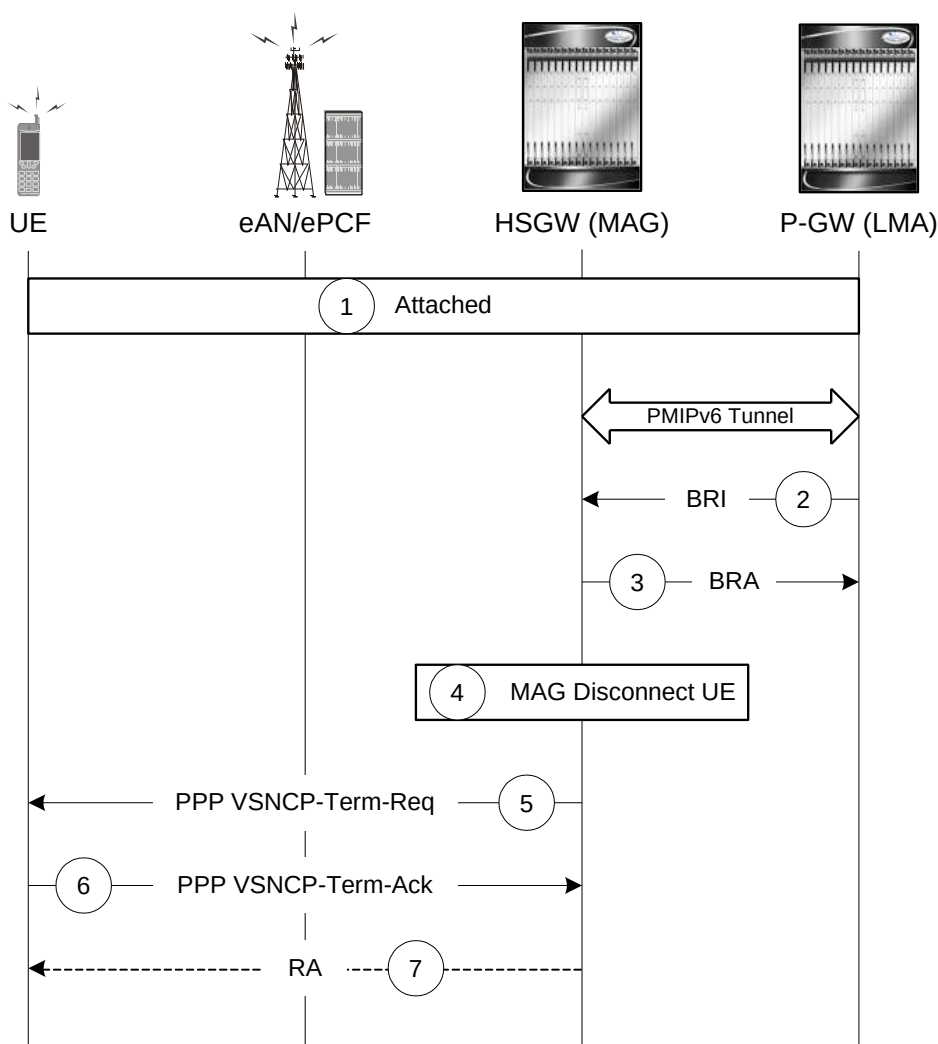
Figure 135. PDN Connection Release by the HSGW Call Flow
