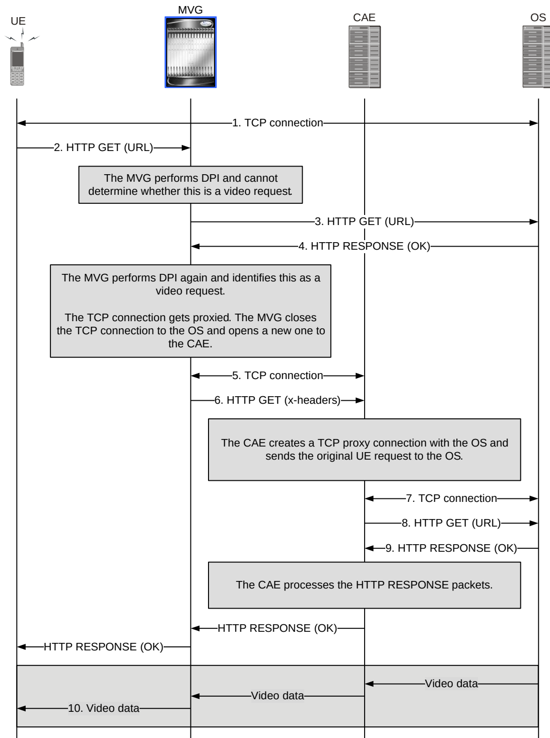
Figure 165. DPI of HTTP RESPONSE Identifying a Video Request
