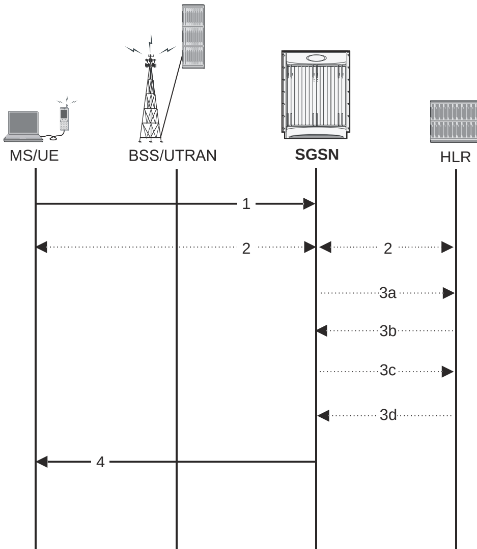
Figure 259. Simple First-Time GPRS Attach
