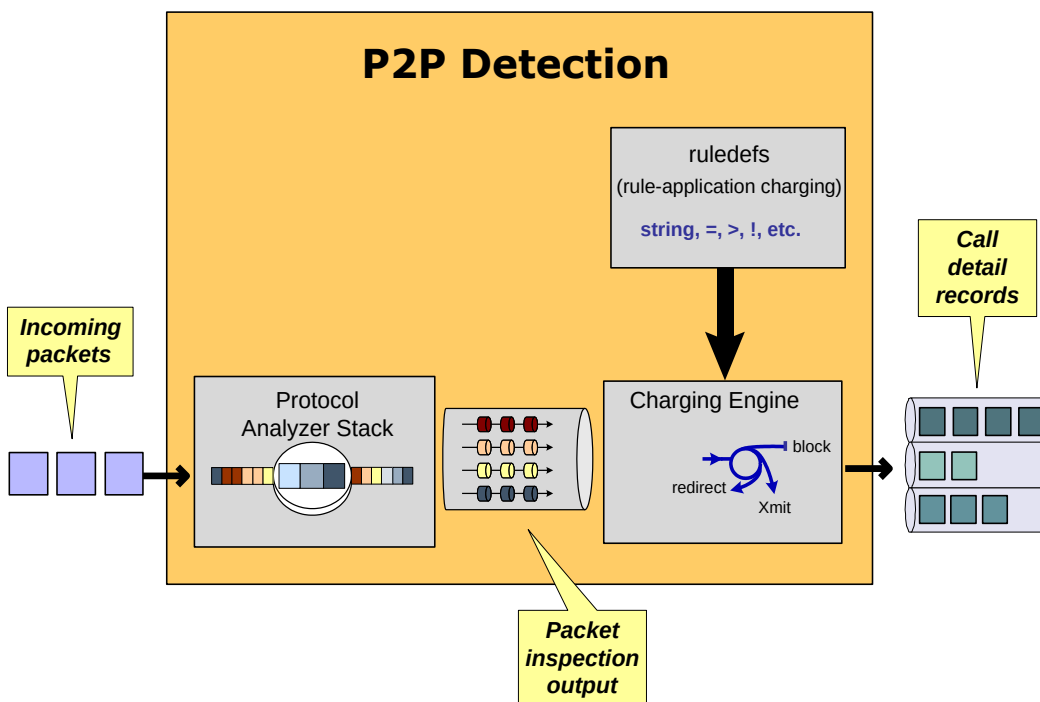
Figure 28. Overview of Packet Processing in ECSv2
