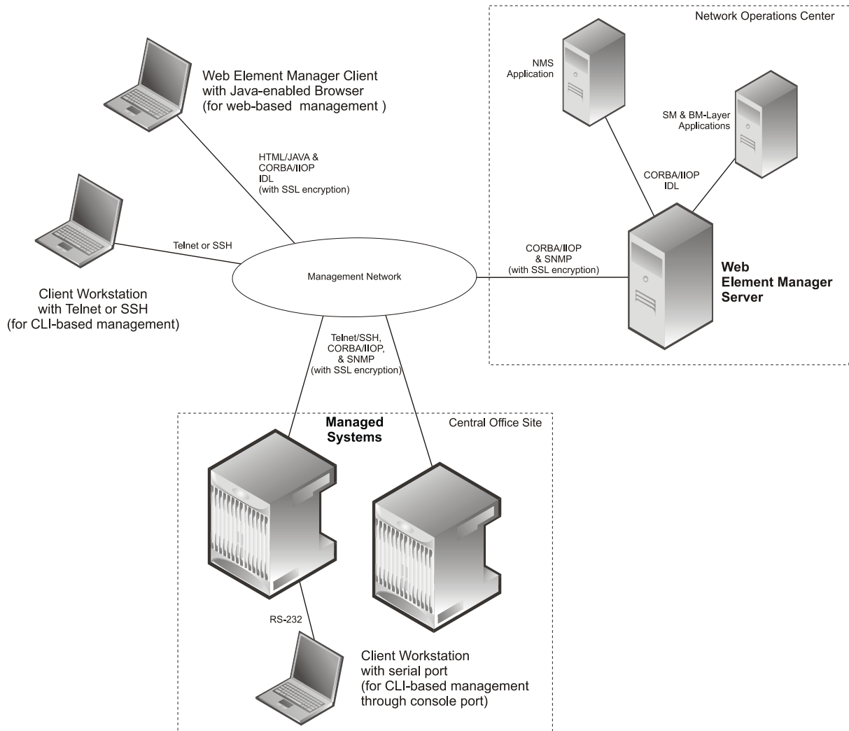
Figure 214. Element Management Methods
