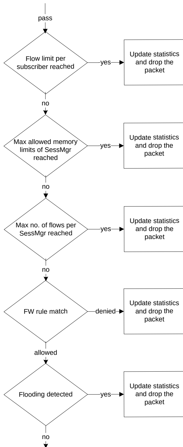
Figure 224. Continued... Stateful Firewall Processing
