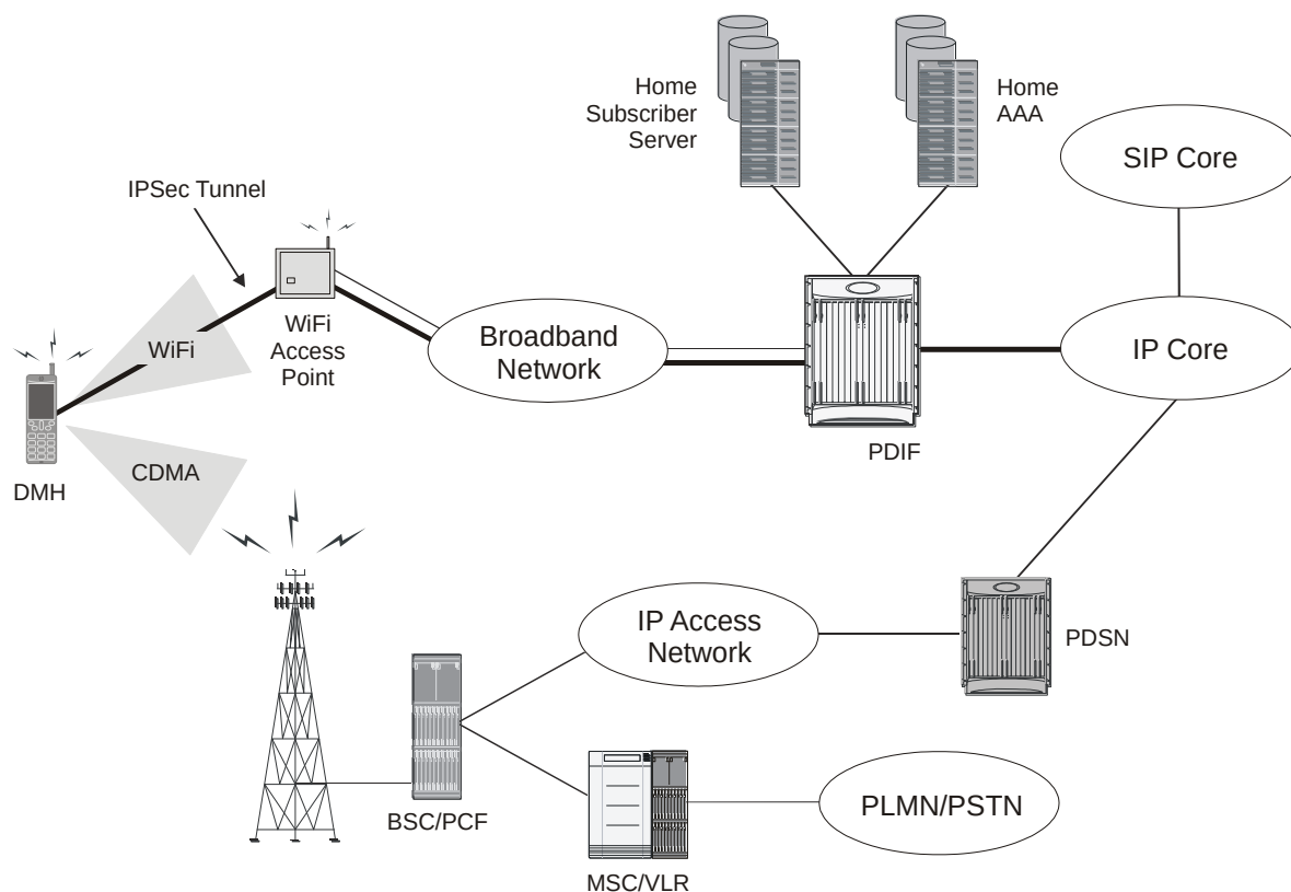
Figure 192. PDIF Simple IP Implementation
