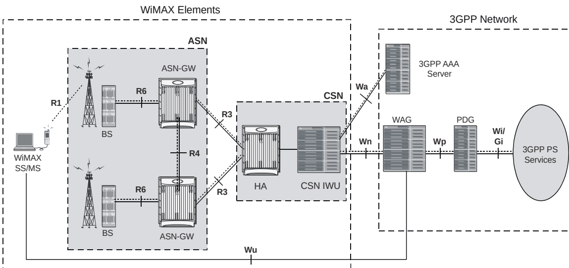
Figure 57. ASN Gateway with 3GPP Overlay
