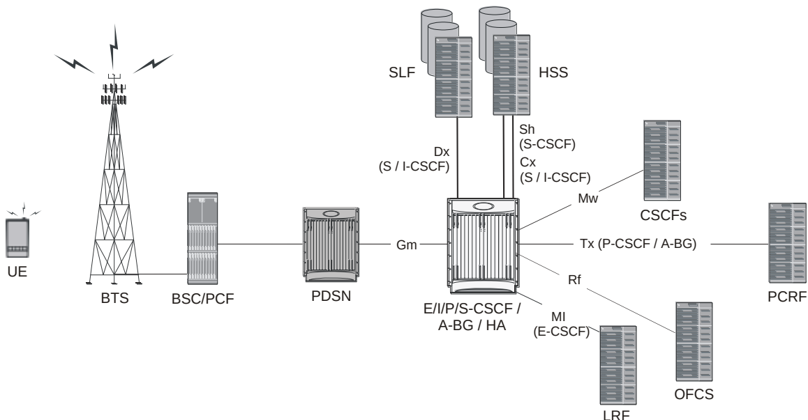
Figure 241. CDMA2000 CSCF/A-BG/HA SCM Deployment Example
