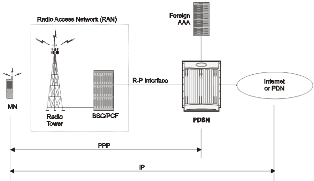
Figure 67. Simple IP Protocol Usage
