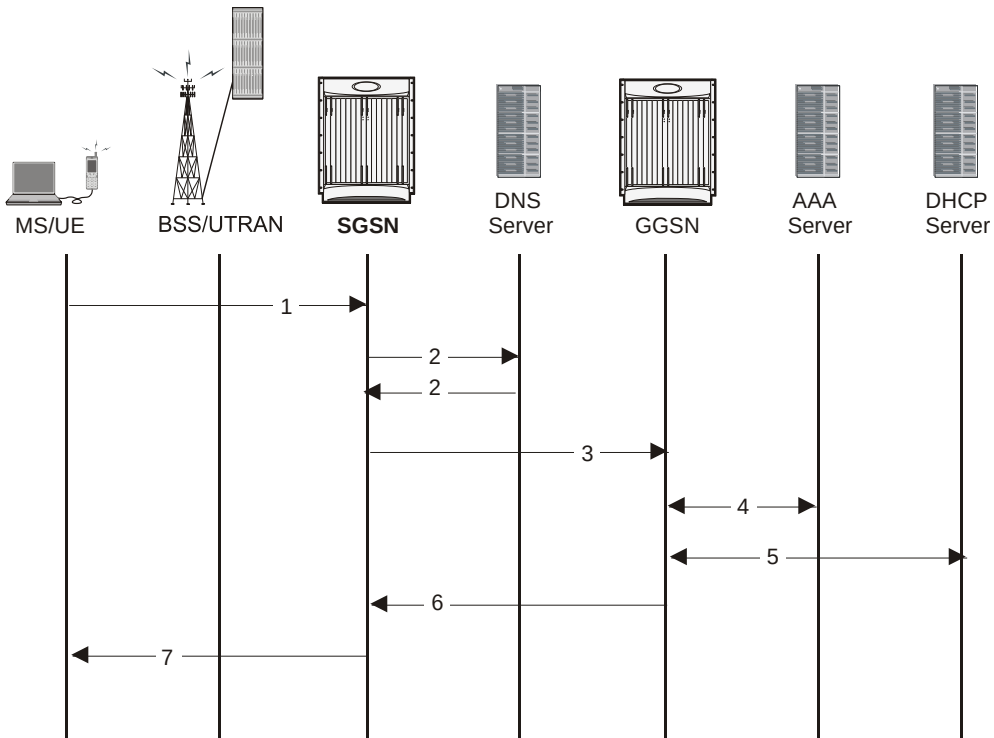
Figure 260. Call Flow for PDP Context Activation
