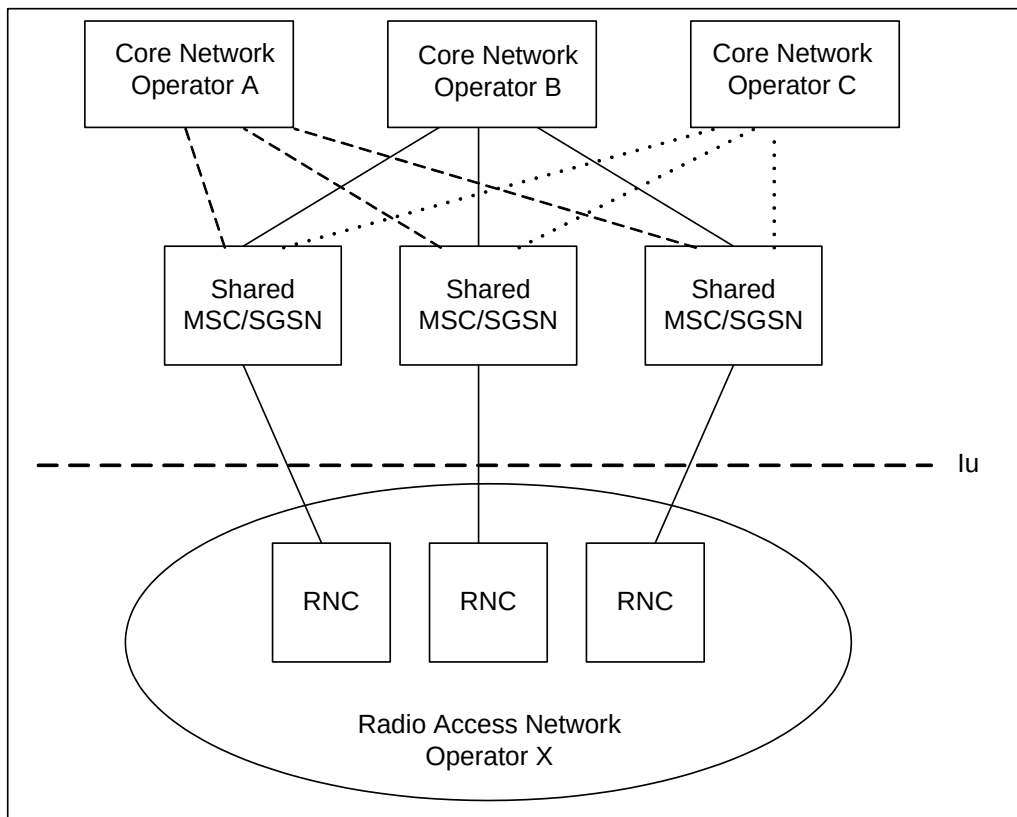
Figure 255. GWCN-type Network Sharing
