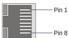
Figure 276. SPIO RJ-45 Ethernet Interface Pin-outs
