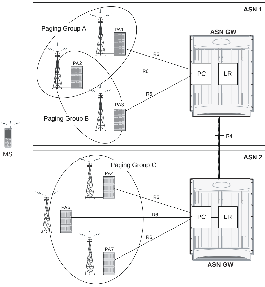
Figure 59. ASN Paging Controller and Location Registry in WiMAX Networks
