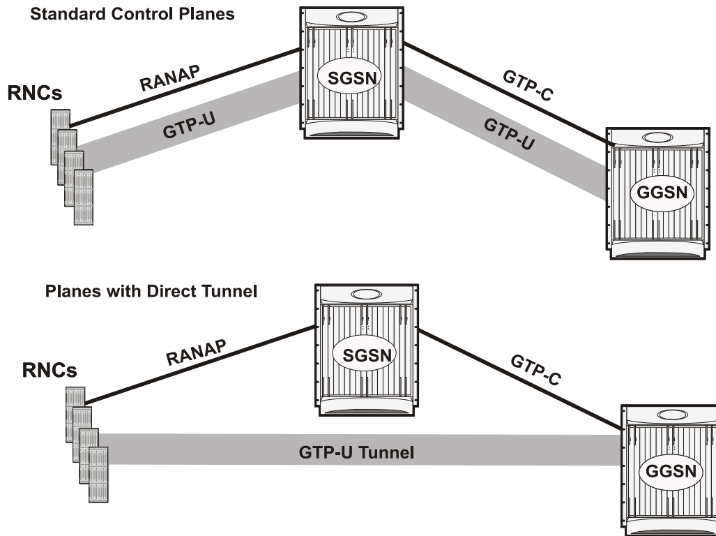
Figure 98. Direct Tunnel Support in GGSN
