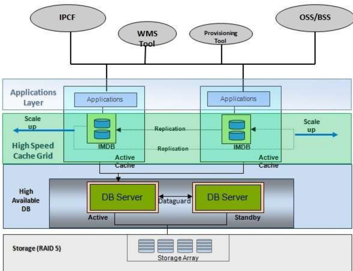
Figure 265. SSC Architecture
