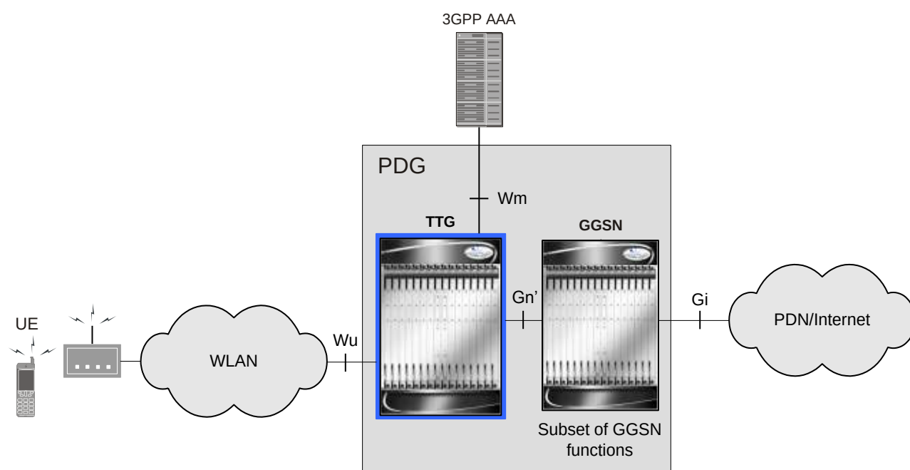
Figure 201. The TTG and GGSN in a PDG Implementation
