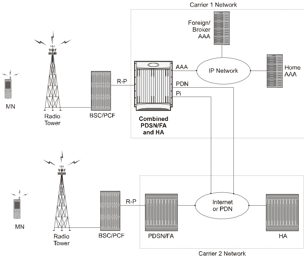
Figure 66. Co-located PDSN/FA and HA Configuration Example
