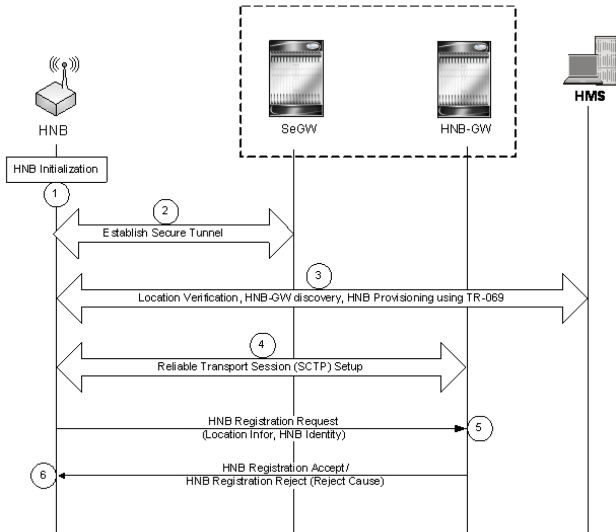
Figure 122. HNB Provisioning and Registration Setup Call Flow
