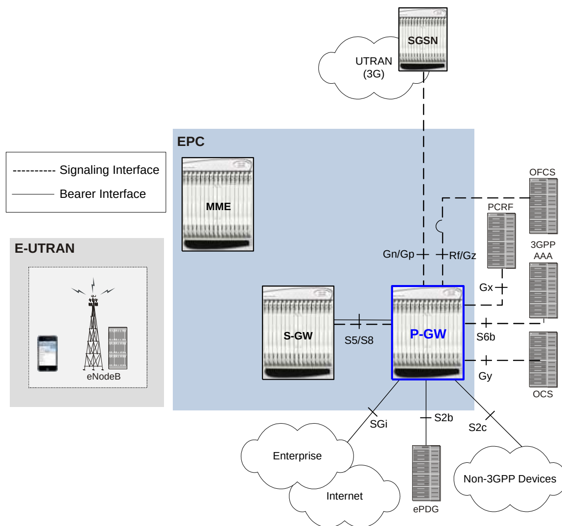
Figure 210. Supported P-GW Interfaces in the E-UTRAN/EPC Network
