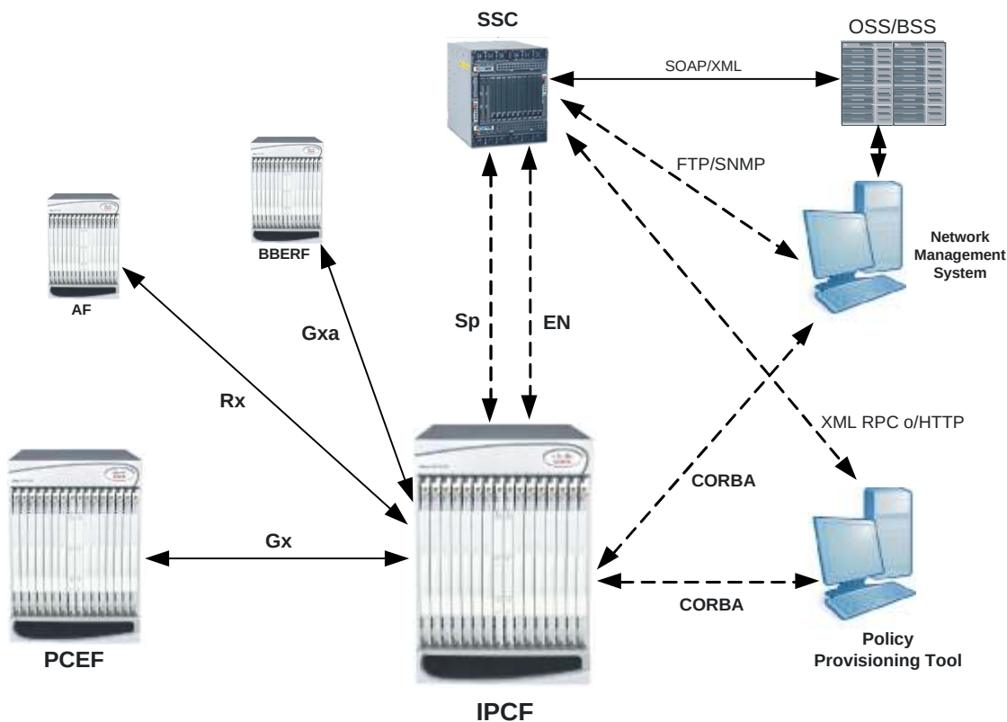
Figure 136. PCC Elements in UTRAN/E-UTRAN/cdma2000-1x/HRPD Networks
