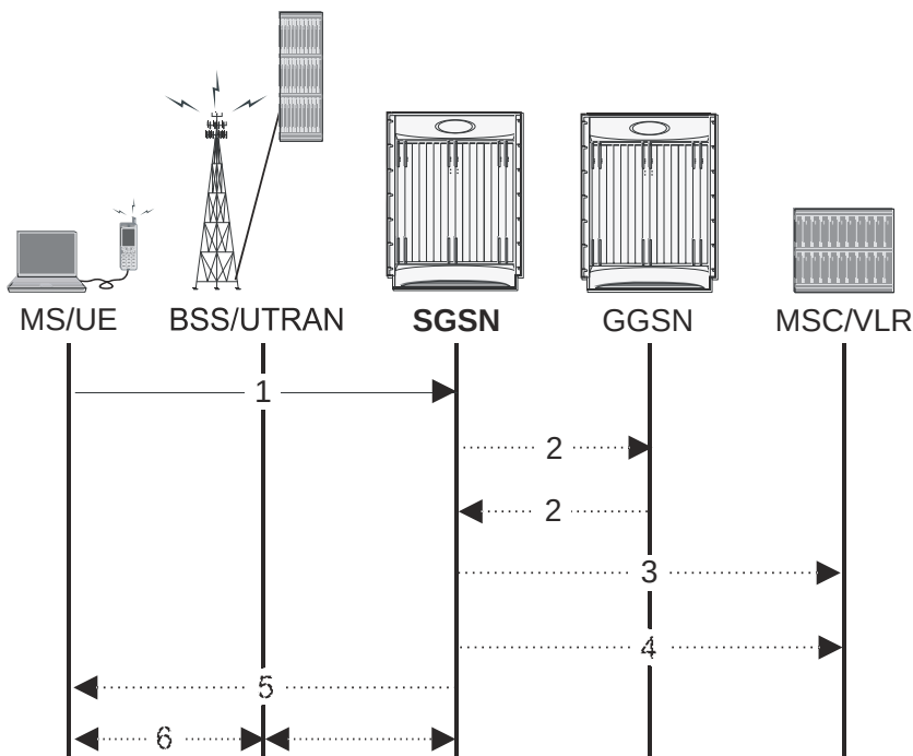
Figure 262. MS-Initiated Combined GPRS/IMSI Detach
