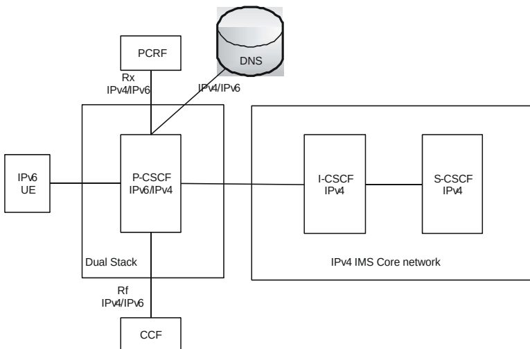
Figure 248. Interworking Between IPv6 UE and IPv4 IMS Core Network
