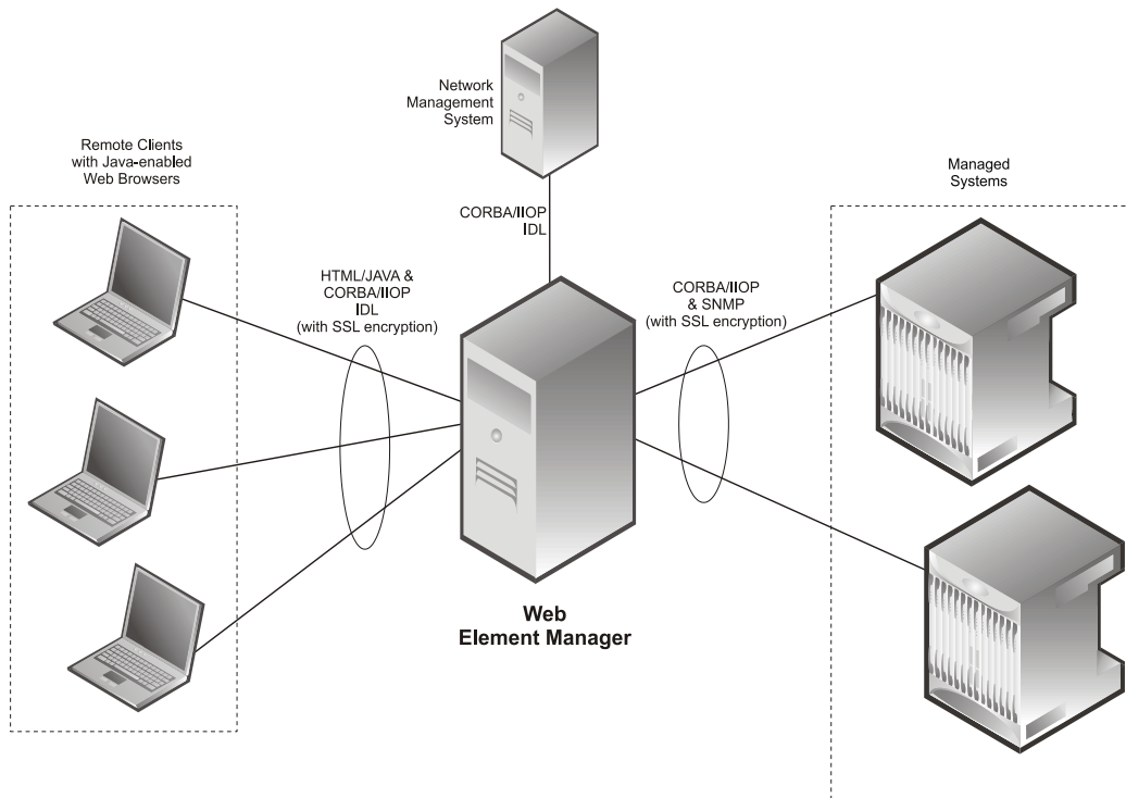
Figure 103. Web Element Manager Network Interfaces
