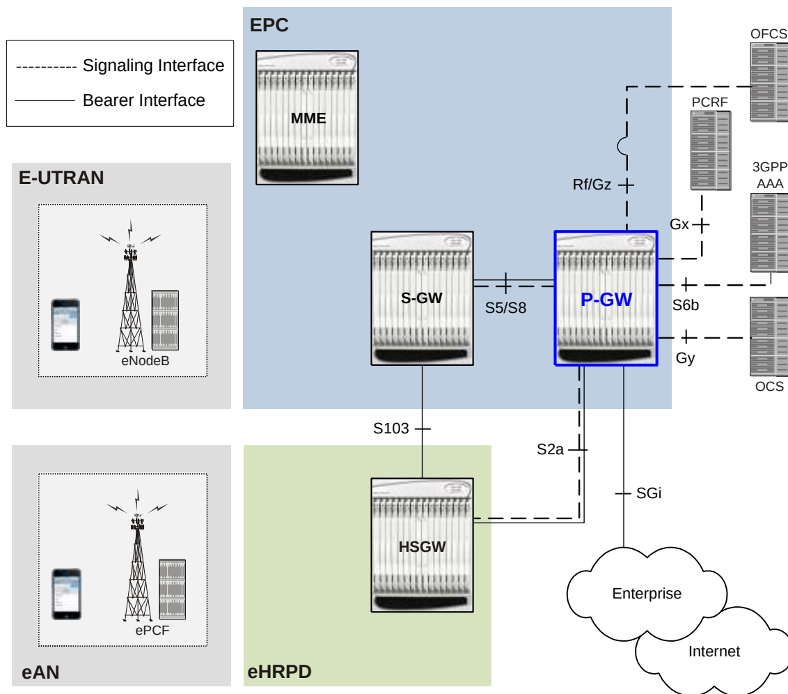
Figure 212. P-GW Interfaces Supporting eHRPD to E-UTRAN/EPC Connectivity
