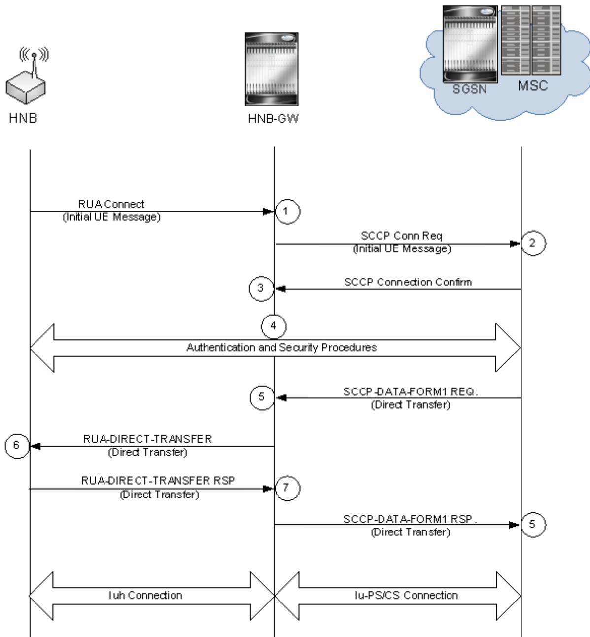
Figure 124. Iu Connection Establishment Call Flow
