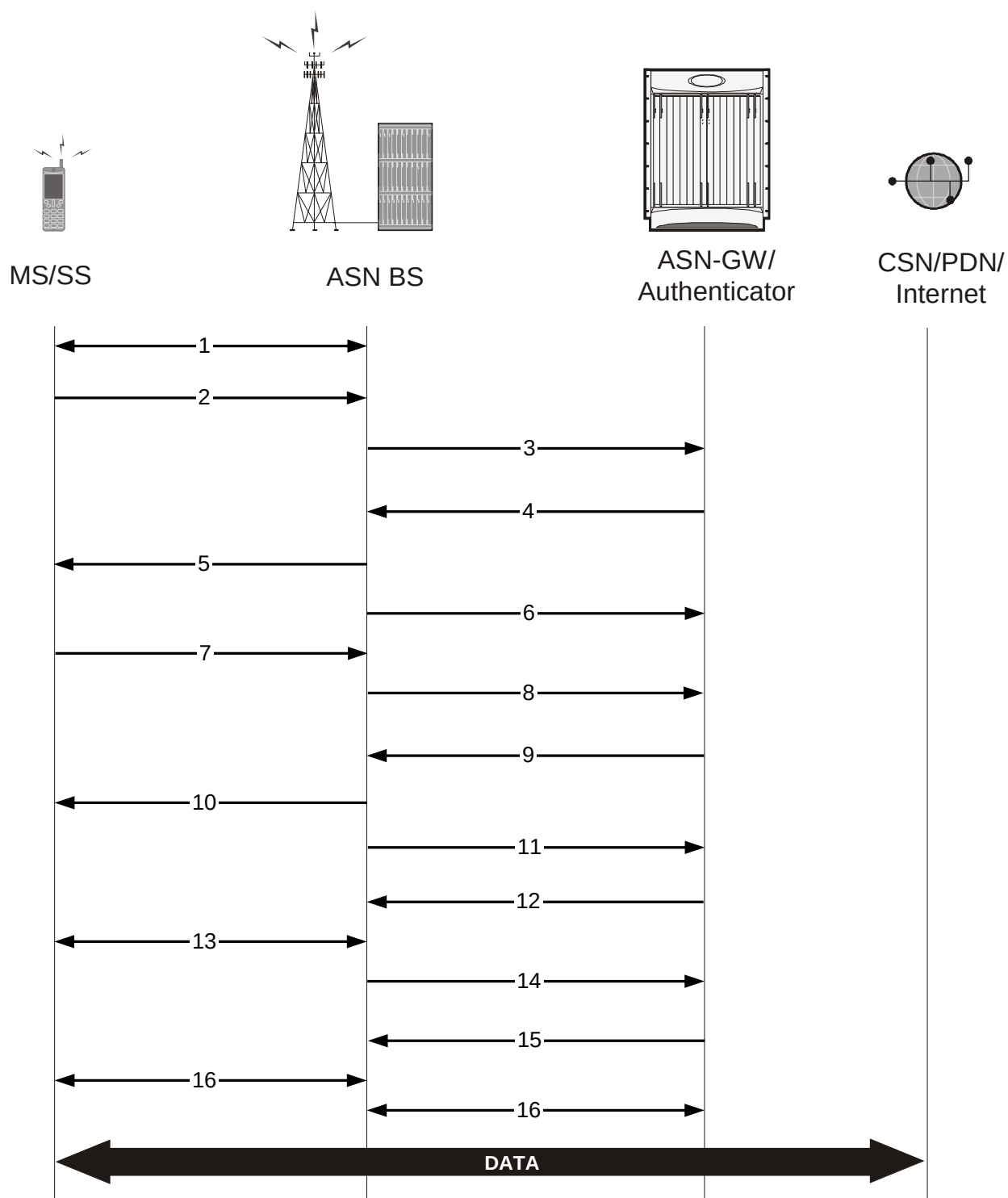
Figure 38. Initial Network Entry and Data Session Establishment without Authentication Call Flow
