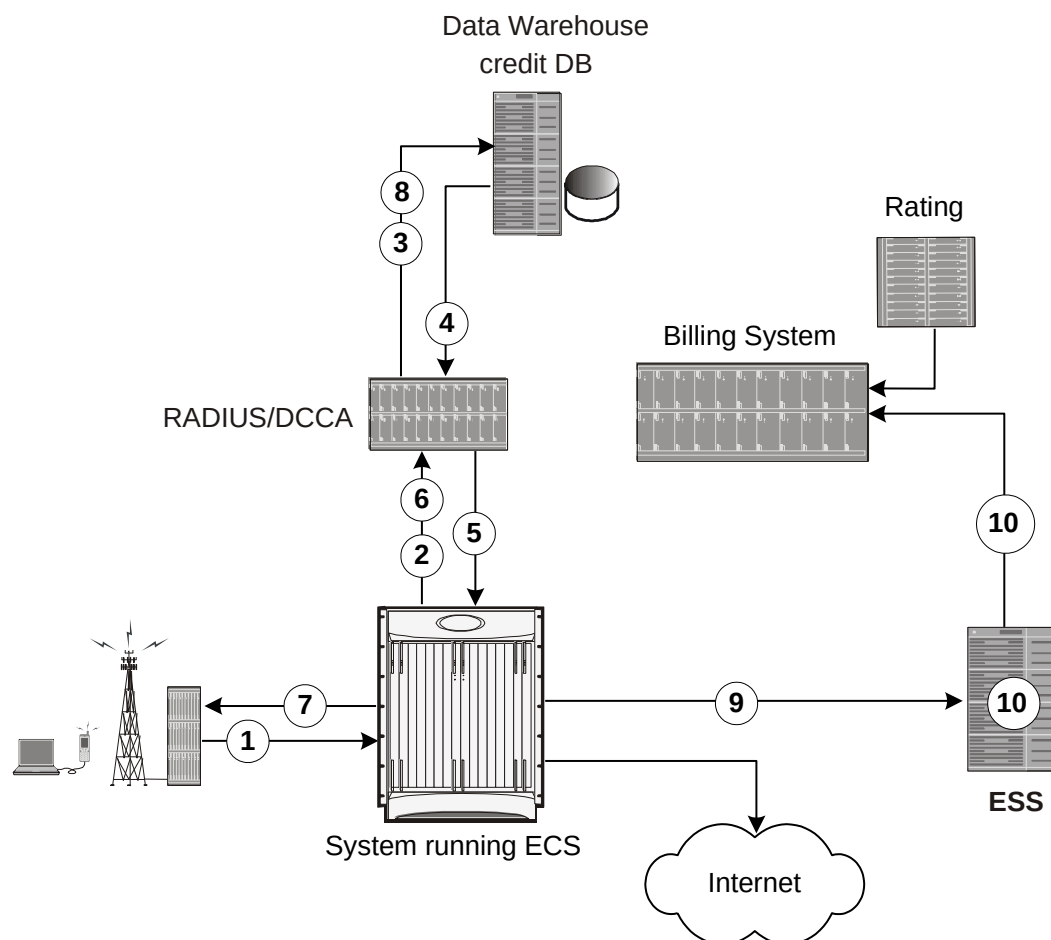
Figure 85. Prepaid Charging in GPRS/UMTS/CDMA-2000 Networks
