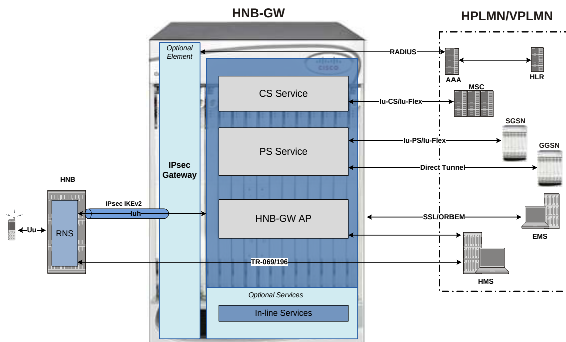
Figure 119. HNB-GW in UMTS Network and Interfaces
