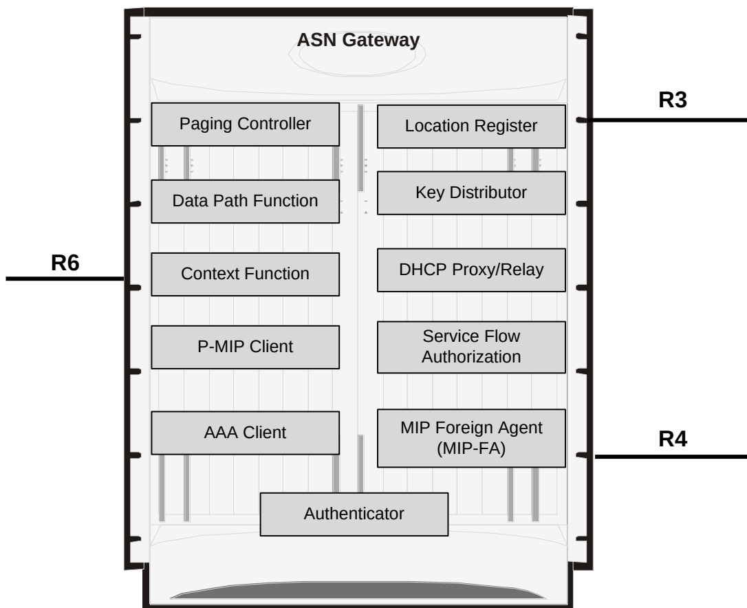
Figure 35. Functional view of ASN Gateway Profile-C
