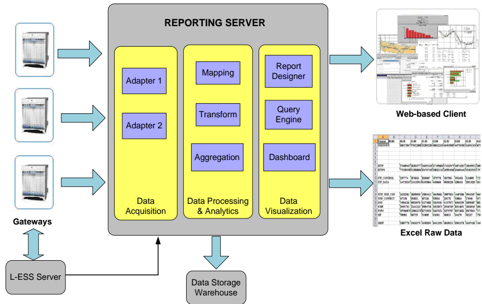
Figure 4. End-to-end Component Mapping
