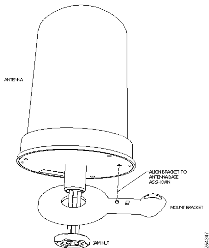
Figure 4 Antenna Bracket
