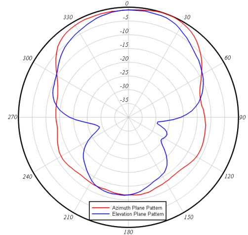
Middle Antenna Azimuth and Elevation Radiation Patterns
