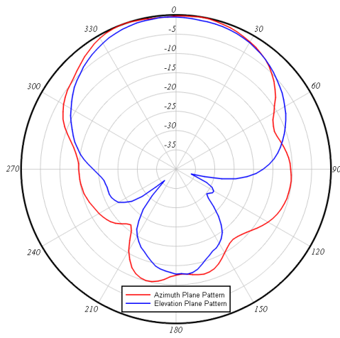
Right Antenna Azimuth and Elevation Radiation Patterns
