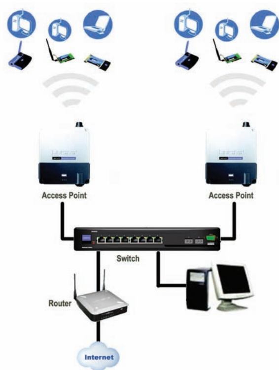
Example of Simple Wireless Network
