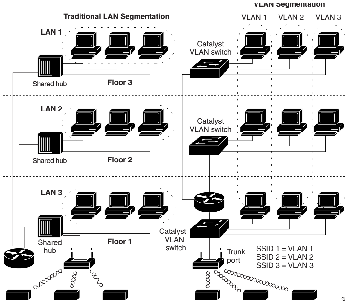
Figure 9-1 LAN and VLAN Segmentation with Wireless Devices
