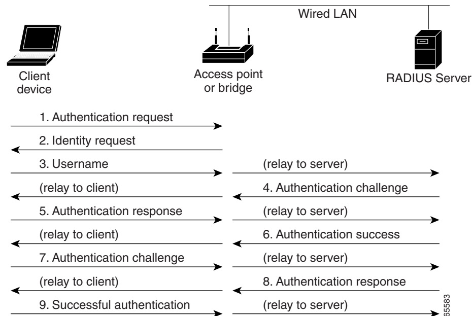
Figure 8-1 Sequence for EAP Authentication
