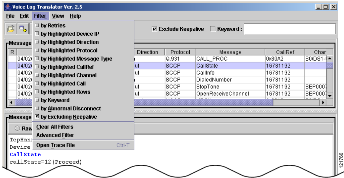
Figure 3 Cisco VLT Toolbar: Successive Display of Choices
