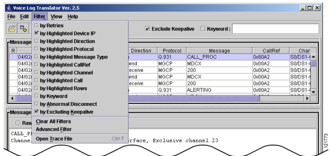
Figure 9 Cisco VLT Filter Menu
