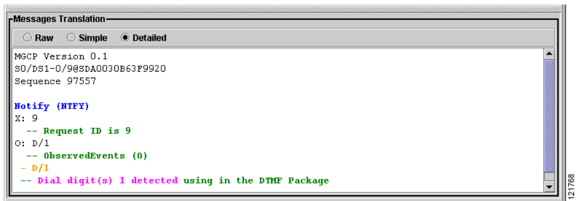
Figure 6 Cisco VLT Detailed Translation
