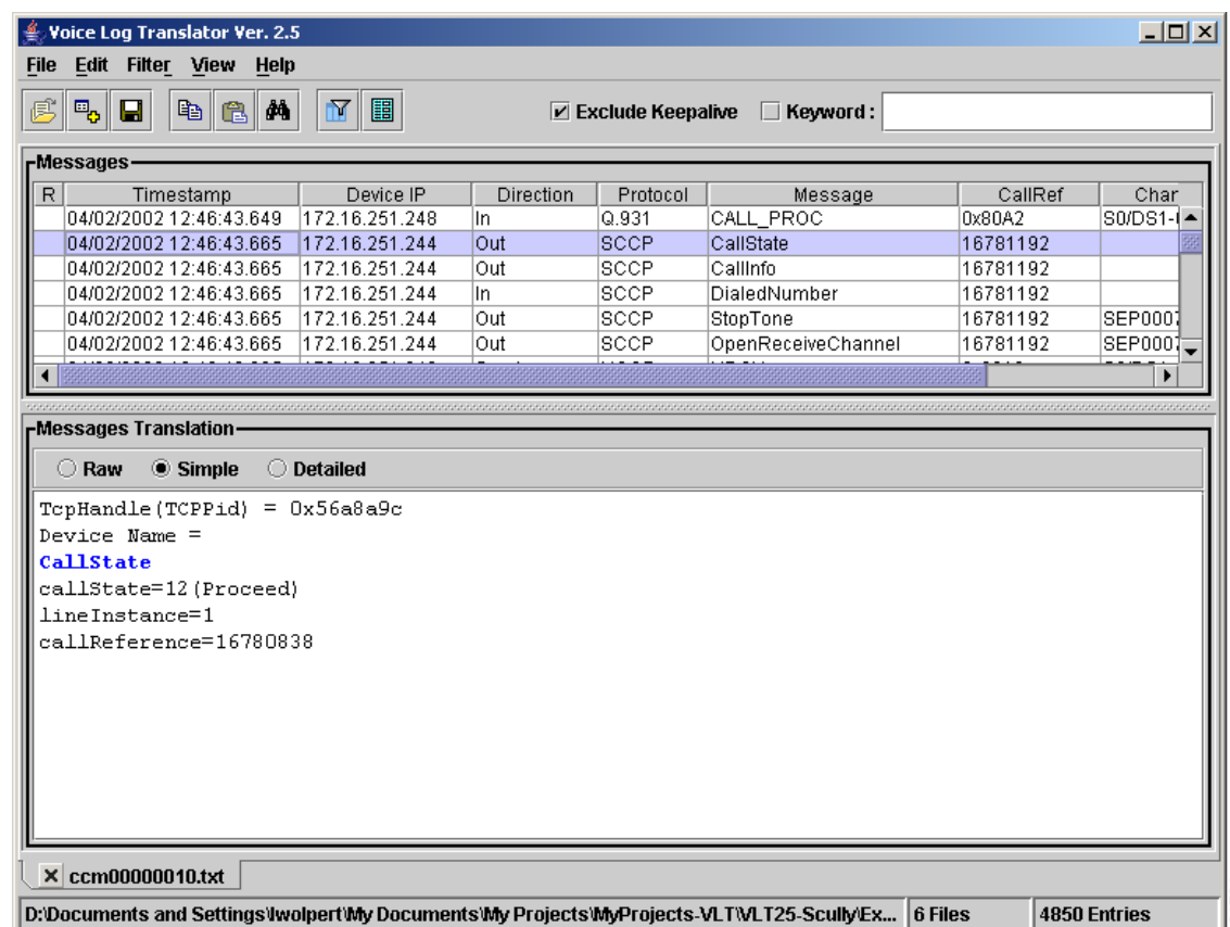
Figure 1 Cisco VLT User Interface
