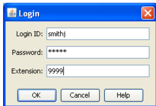
Figure 3. Login window
