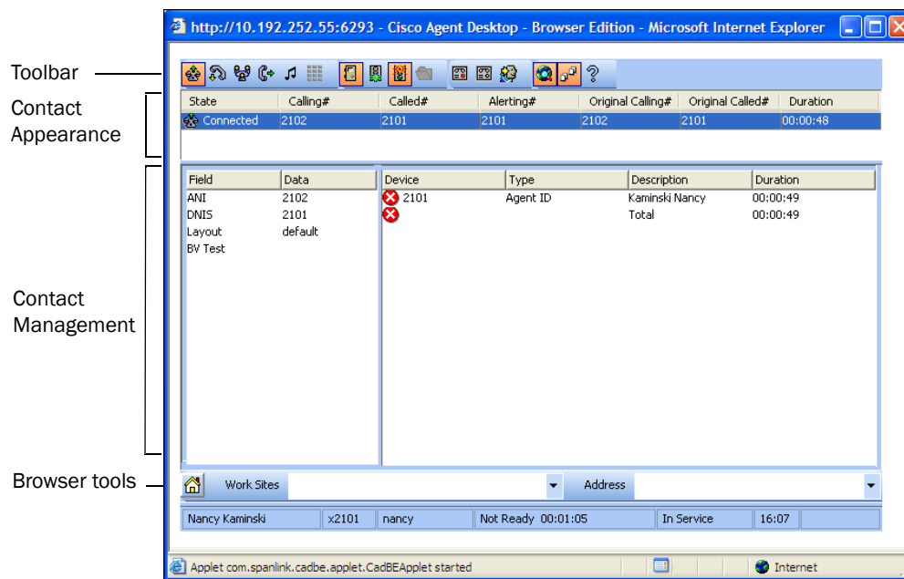
Figure 1. CAD-BE interface
