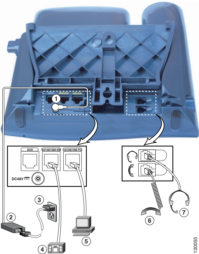
Figure 3-1 Cisco Unified IP Phone 7970 Series Rear Cable Connections
