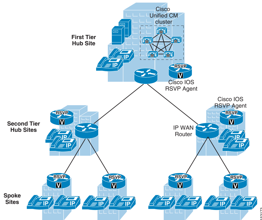
Figure 9-26 Two-Tier Hub-and-Spoke Topology with Centralized Unified CM
