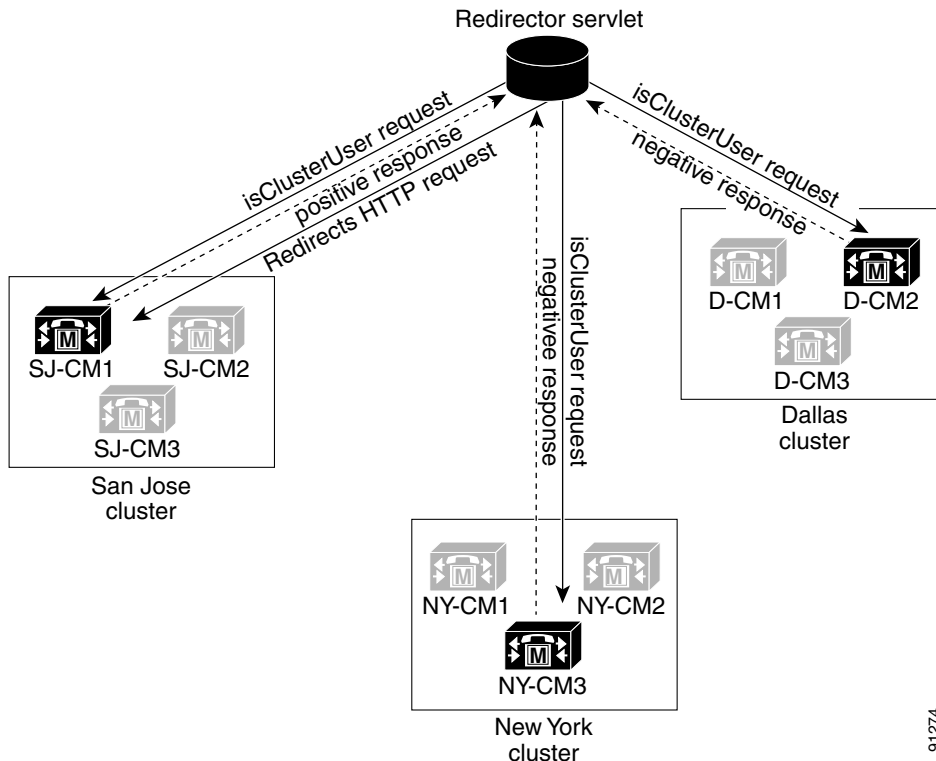
Figure 8-1 Multiple Clusters
