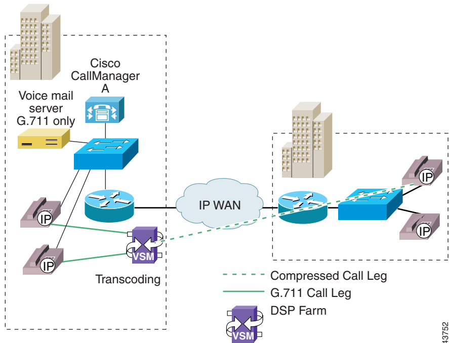
Figure 24-1 Multisite WAN Using Centralized MTP Transcoding and Conferencing Services
