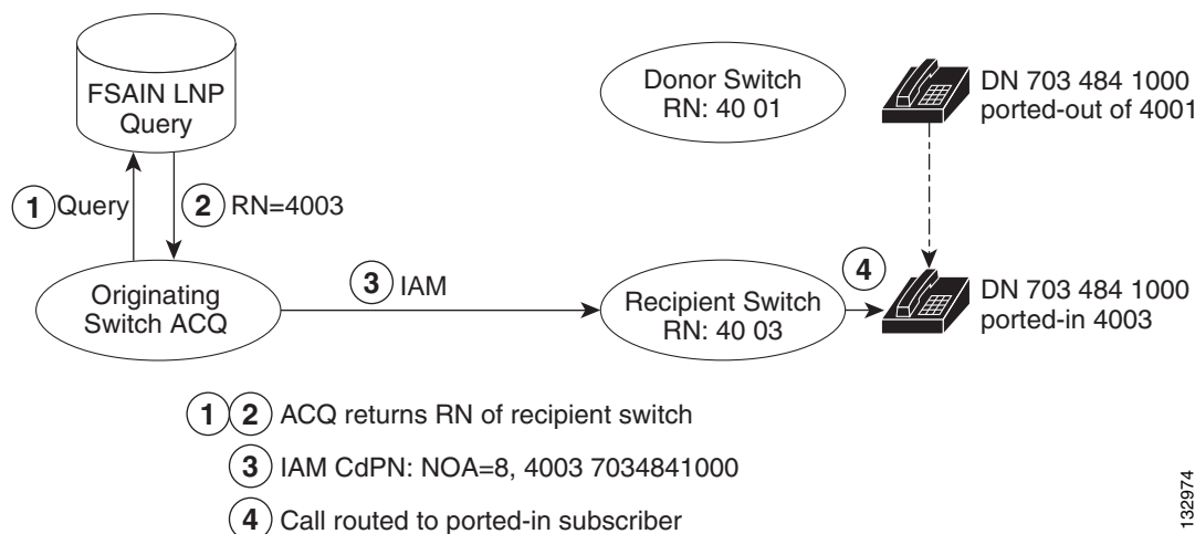
Figure 2-7 ACQ
