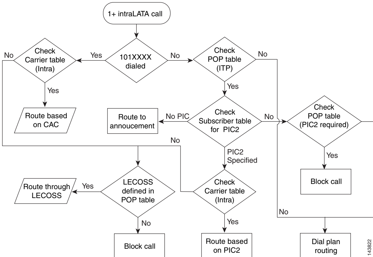
Figure 2-19 1+ IntraLATA Call
