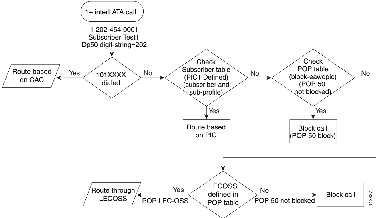
Figure 6-7 1+ InterLATA Call
