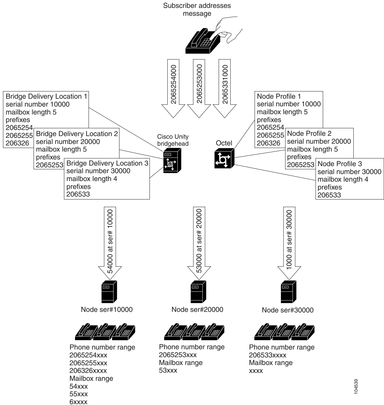
Figure 1: Network Addressing
