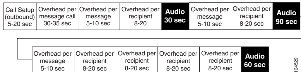
Figure 15: Outbound Message Delivery Call—Example 1
