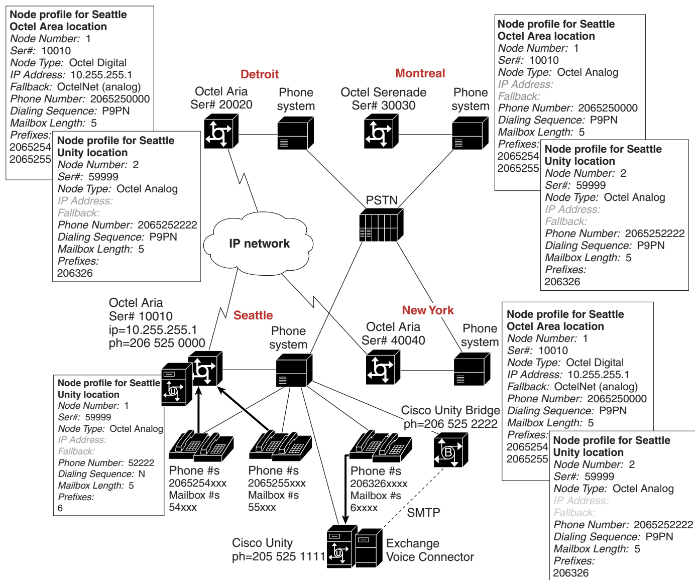
Figure 5: Changes to the Network Node Configuration to Accommodate a Migration to Cisco Unity
