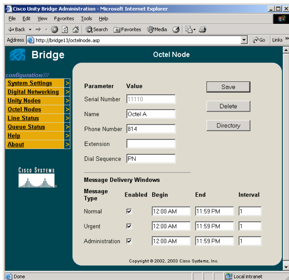
Figure 41: Octel Node Page in the Bridge Administrator
