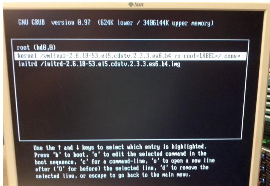
Figure 35: GRUB
