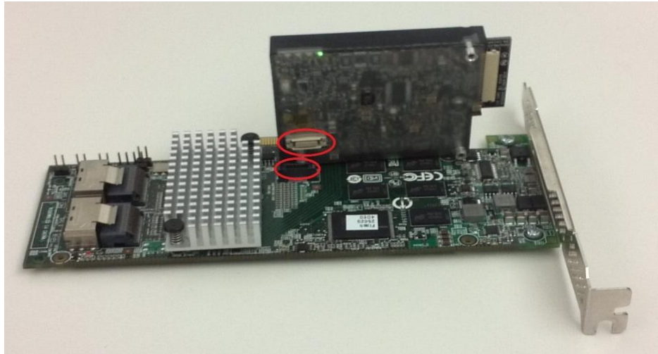
Figure 2B: MegaRAID 9261-8i and BBU
