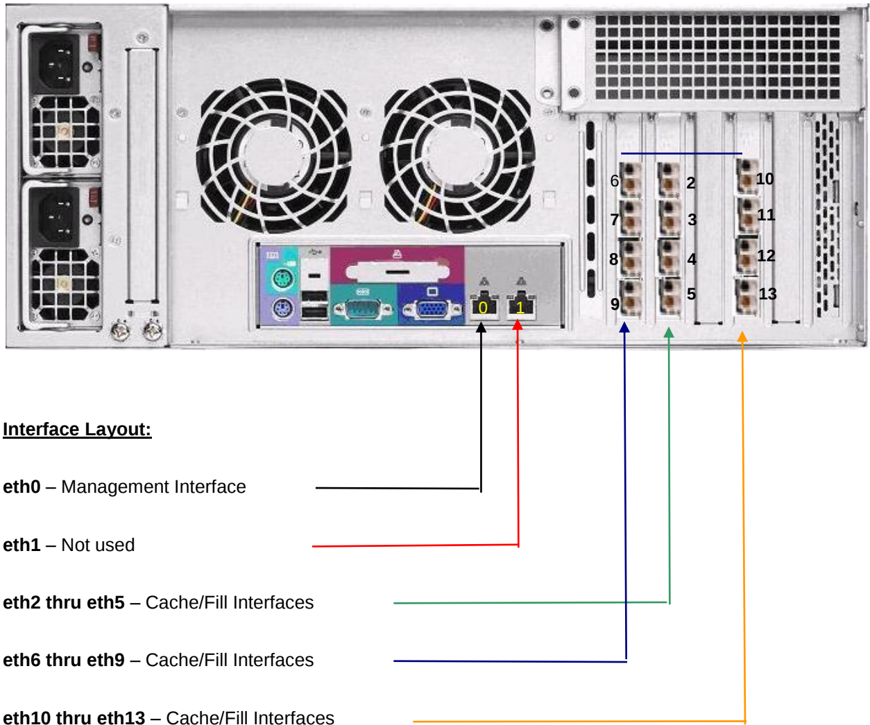
Figure 3C: Caching Gateway Back View
