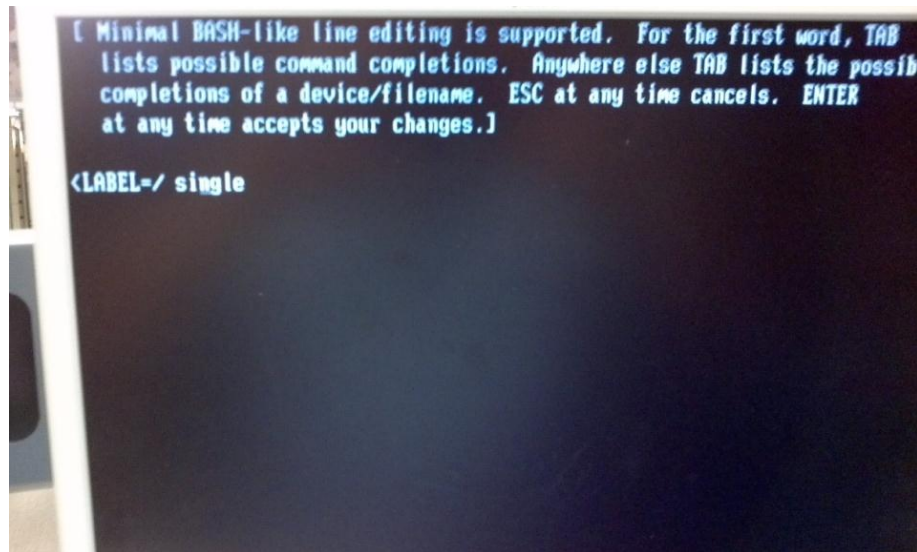
Figure 9: Bash
