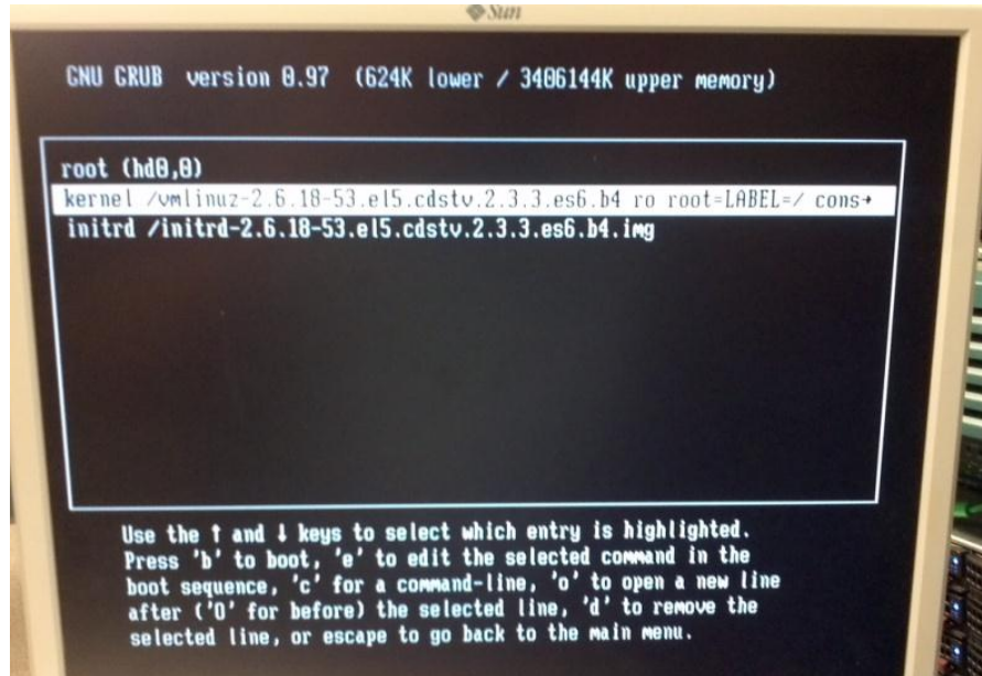
Figure 37: GRUB
