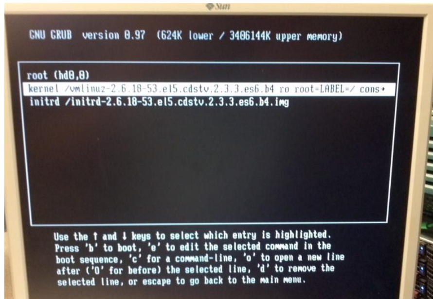
Figure 22: GRUB
