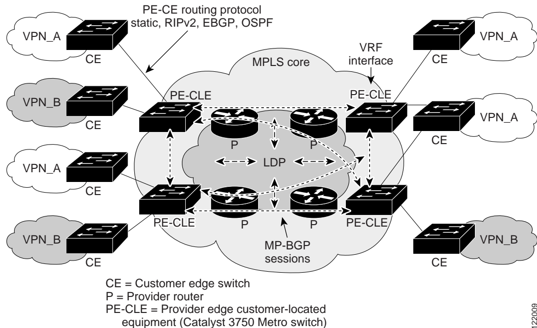
Figure 1-3 MPLS VPN Configuration
