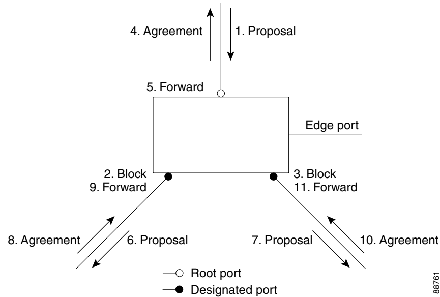
Figure 17-9 Sequence of Events During Rapid Convergence
