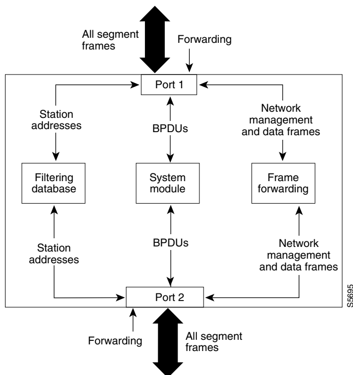
Figure 17-6 Interface 2 in Forwarding State
