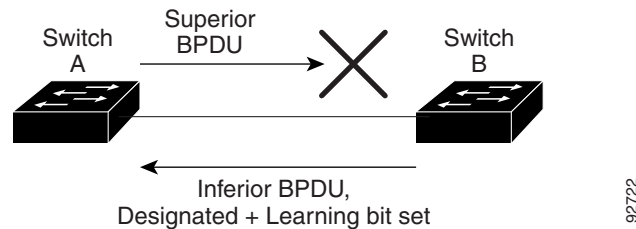
Figure 17-12 Detecting Unidirectional Link Failure
