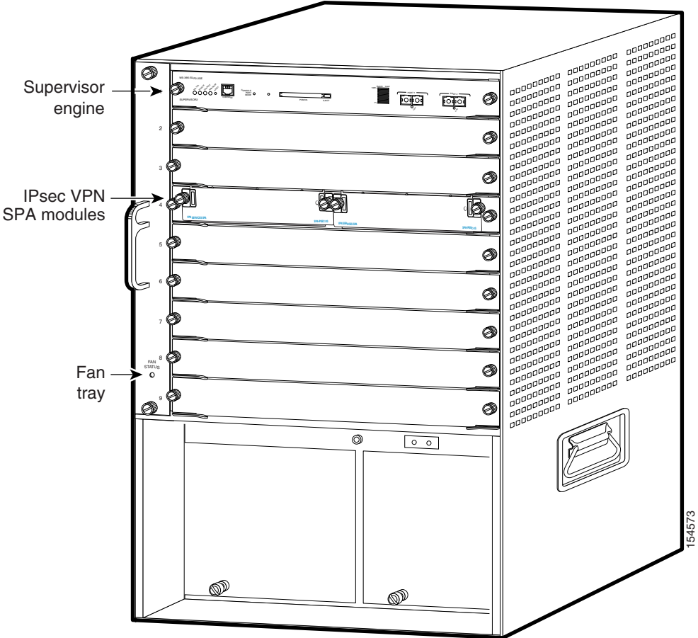
Figure 2 Catalyst 6509 and Catalyst 6509-E Switches
