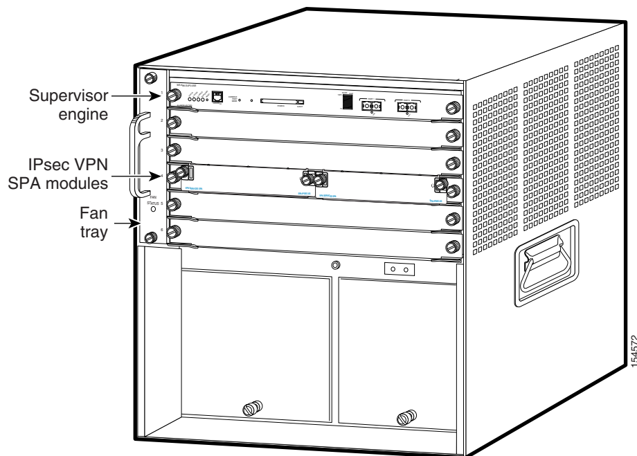
Figure 1 Catalyst 6506 and Catalyst 6506-E Switches
