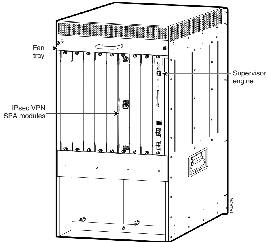
Figure 4 Cisco 7609 Router
