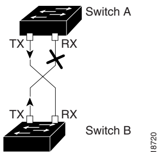
Figure 24-1 Unidirectional Link
