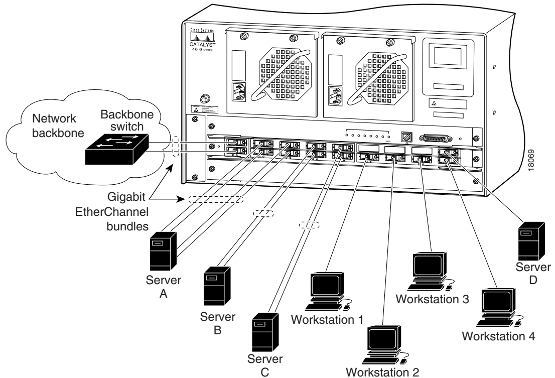
Figure 6-1 Example Server Switching Network Topology
