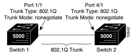
Figure 12-7 IEEE 802.1Q Trunking: Final Network Configuration
