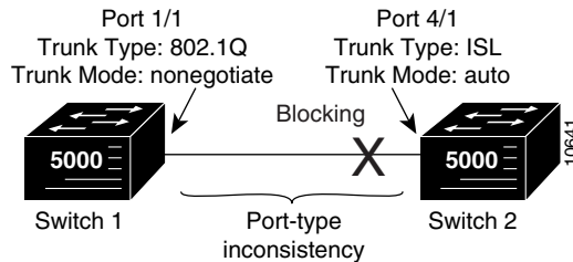
Figure 12-6 IEEE 802.1Q Trunking: Port-Type Inconsistency
