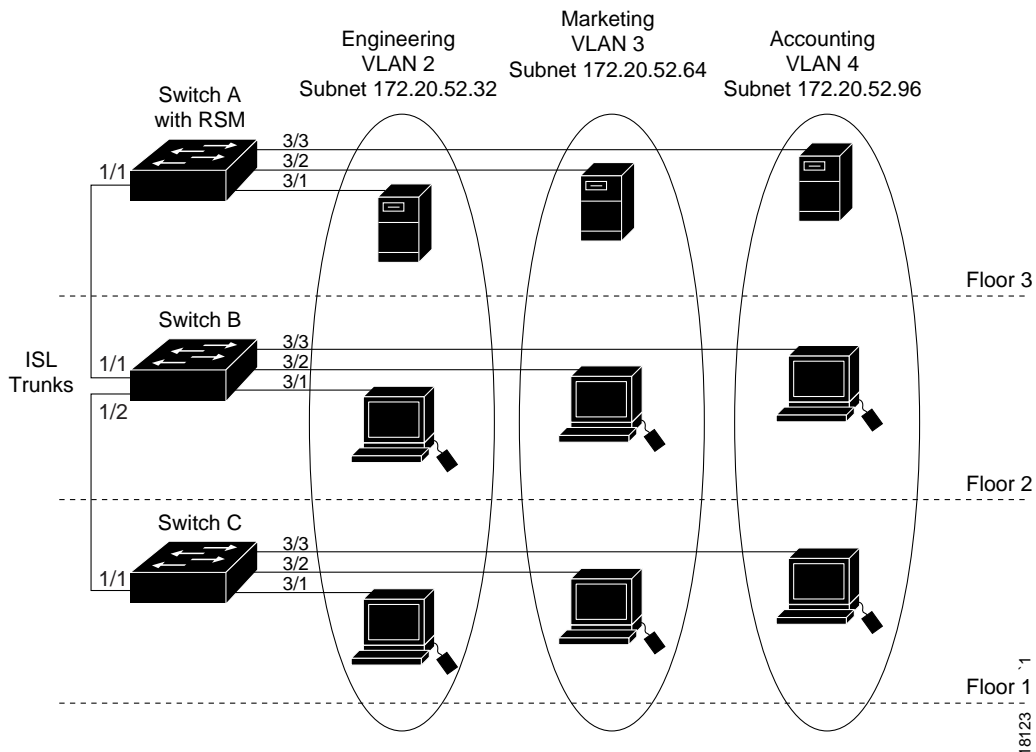
Figure 39-3 InterVLAN Routing with the RSM Example Configuration
