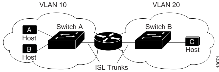
Figure 39-1 Basic InterVLAN Routing Topology
