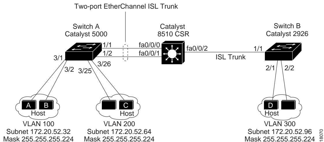
Figure 39-5 InterVLAN Routing with External Catalyst 8510 CSR Example Configuration
