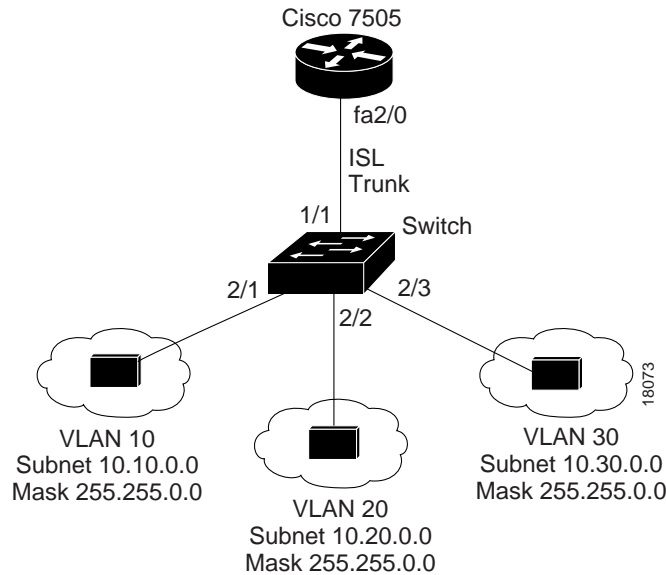
Figure 39-4 InterVLAN Routing with External Cisco 7505 Example Configuration
