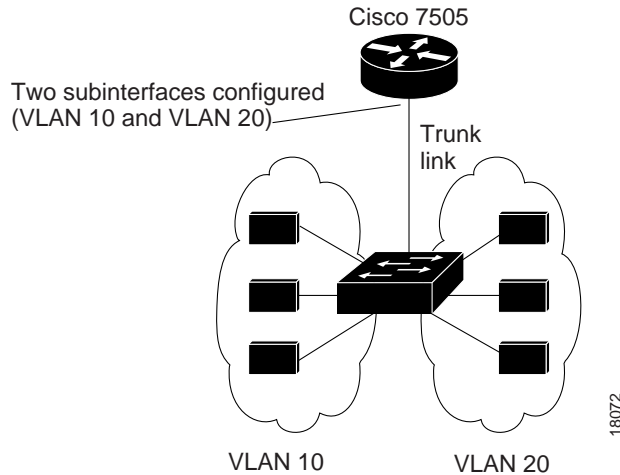
Figure 39-2 InterVLAN Routing Over a Single Trunk Link
