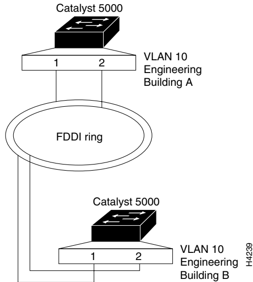
Figure 44-2 Multiple Catalyst 5000 Series Switch VLAN Configuration without Trunking
