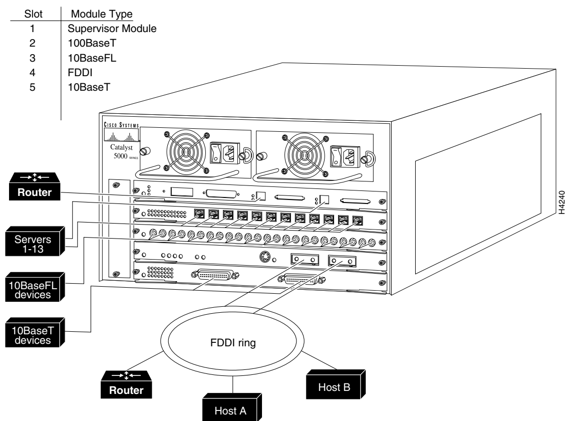
Figure 44-1 Single Catalyst 5000 Series Switch Configuration
