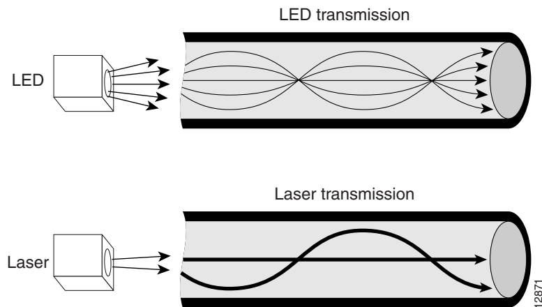
Figure B-1 LED Transmission Compared to Laser Transmission
