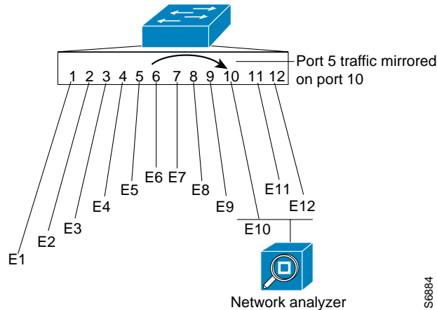
Figure 33-1 Example SPAN Configuration
