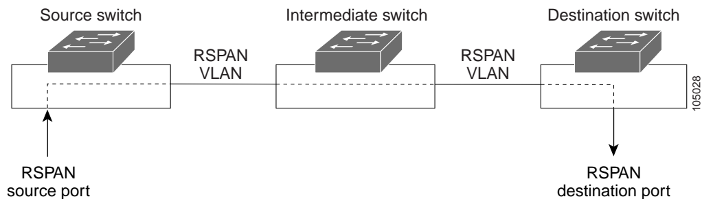
Figure 33-2 Example of RSPAN Configuration
