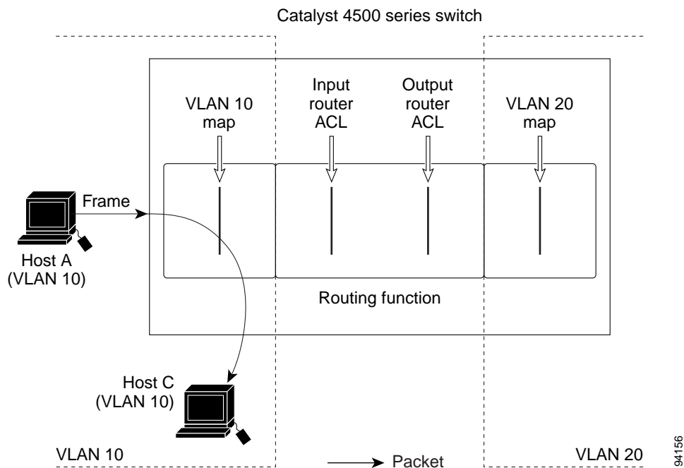
Figure 24-5 Applying ACLs on Switched Packets
