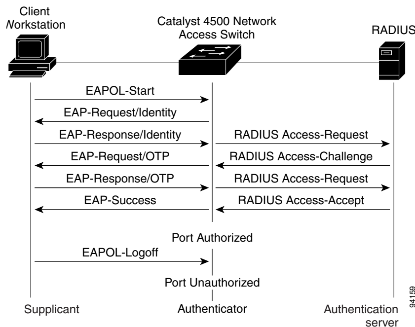
Figure 26-2 Message Exchange
