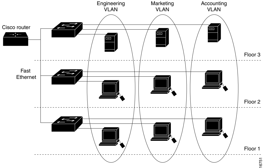
Figure 7-1 Sample VLANs
