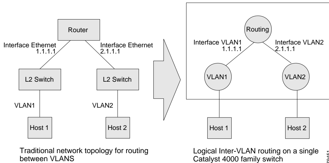
Figure 18-1 Logical Layer 3 VLAN Interfaces for the Catalyst 4000 Family
