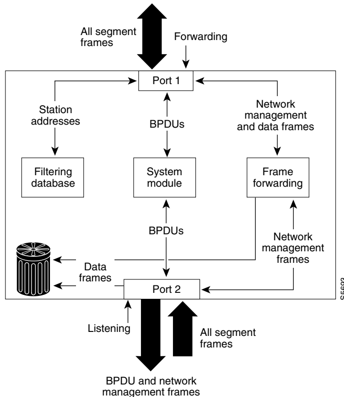
Figure 12-4 Layer 2 Interface in Listening State
