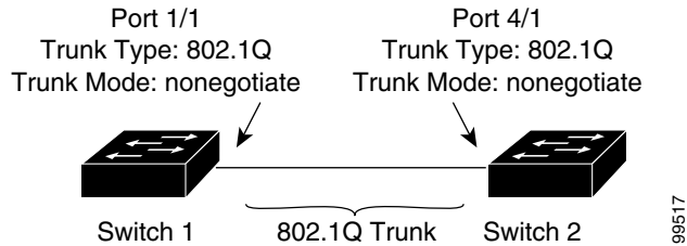
Figure 11-6 802.1Q Trunking: Final Network Configuration
