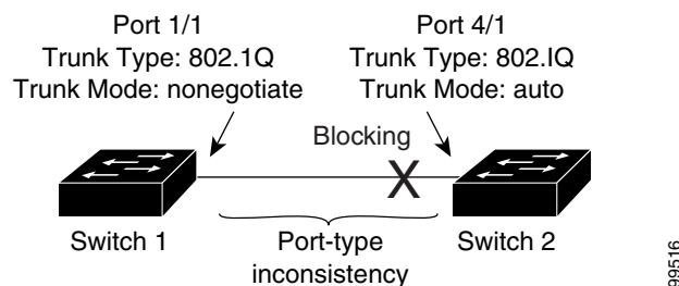
Figure 11-5 802.1Q Trunking: Port-Type Inconsistency
