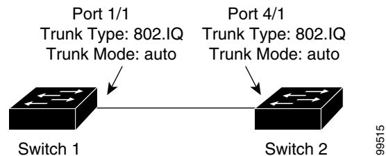
Figure 11-4 802.1Q Trunking: Initial Network Configuration
