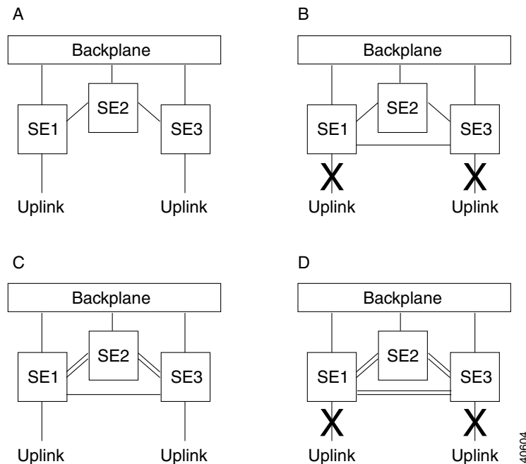
Figure 33-1 Switch Acceleration Configuration Modes
