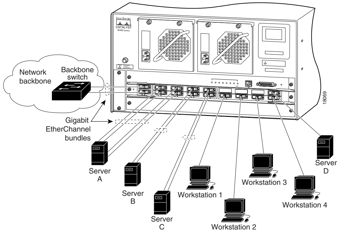
Figure 5-1 Example Server Switching Network Topology
