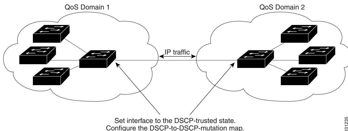
Figure 37-15 DSCP-Trusted State on a Port Bordering Another QoS Domain
