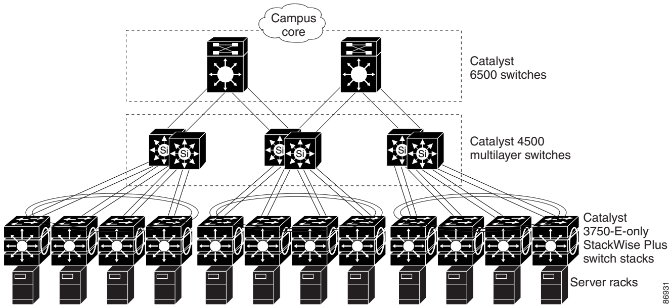
Figure 0-5 Server Aggregation
