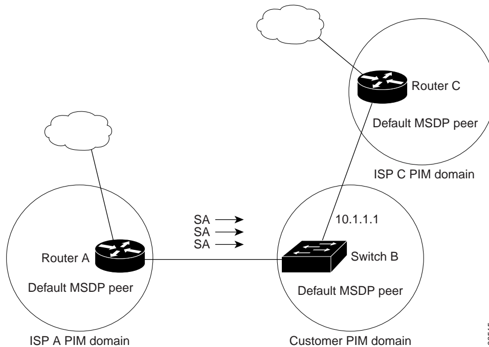
Figure 43-2 Default MSDP Peer Network
