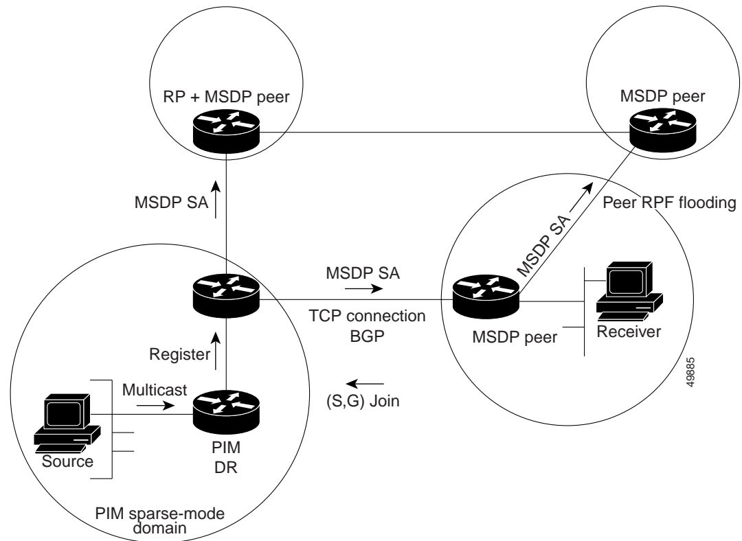
Figure 43-1 MSDP Running Between RP Peers
