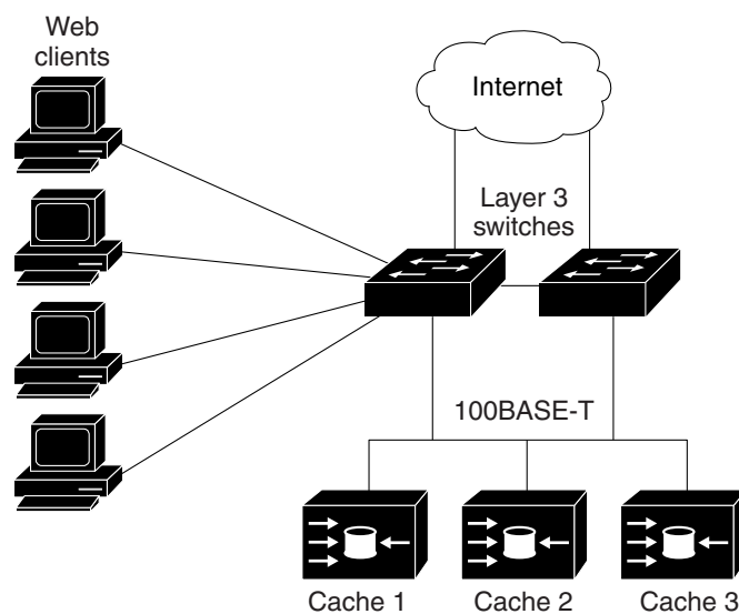
Figure 45-1 Cisco Cache Engine and WCCP Network Configuration
