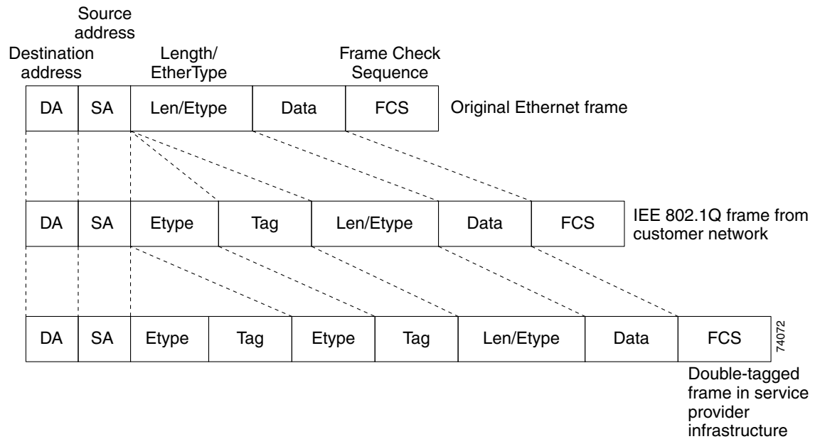
Figure 18-2 Original (Normal), IEEE 802.1Q, and Double-Tagged Ethernet Packet Formats
