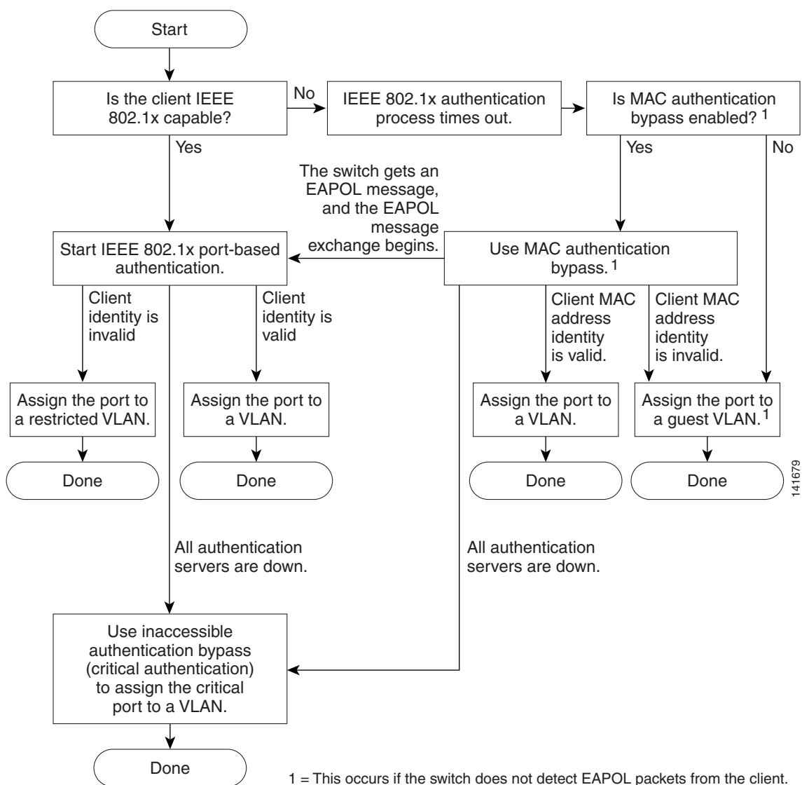
Figure 10-2 Authentication Flowchart
