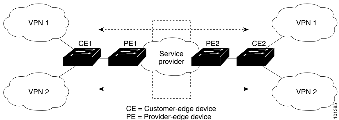
Figure 38-6 Catalyst 3750 Switches Acting as Multiple Virtual CEs
